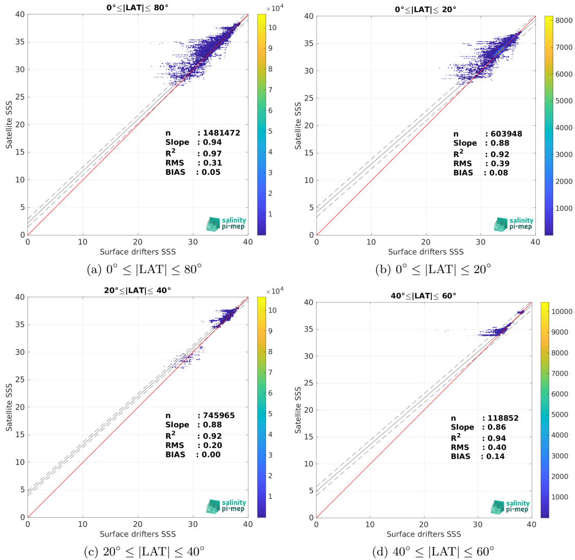
Figure 8: Contour maps of the concentration of SMAP SSS L4 OI v2 - Monthly (IPRC) SSS (y-axis) versus Surface drifters SSS (x-axis) at match-up pairs for different latitude bands. For each plot, the red line shows x=y . The black thin and dashed lines indicate a linear fit through the data cloud and the \pm 95\% confidence levels, respectively. The number match-up pairs n , the slope and R^2 coefficient of the linear fit, the root mean square (RMS) and the mean bias between satellite and in situ data are indicated for each latitude band in each plots.
