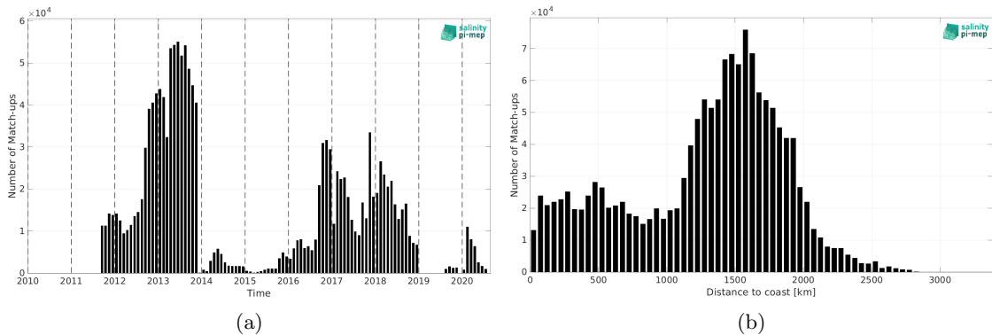
Figure 1: Number of match-ups between Surface drifters and SMAP SSS L4 OI v2 - Monthly (IPRC) SSS as a function of time (a) and as function of the distance to coast (b) over the Global Ocean Pi-MEP region and for the full satellite product period.
