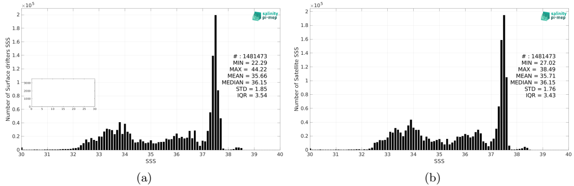
Figure 2: Histograms of SSS from Surface drifters (a) and SMAP SSS L4 OI v2 - Monthly (IPRC) (b) considering all match-up pairs per bins of 0.1 over the Global Ocean Pi-MEP region and for the full satellite product period.
