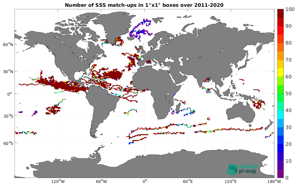
Figure 3: Number of SSS match-ups between Surface drifters SSS and the SMAP SSS L4 OI v2 - Monthly (IPRC) SSS product for the Global Ocean Pi-MEP region over 1°×1° boxes and for the full satellite product period.
