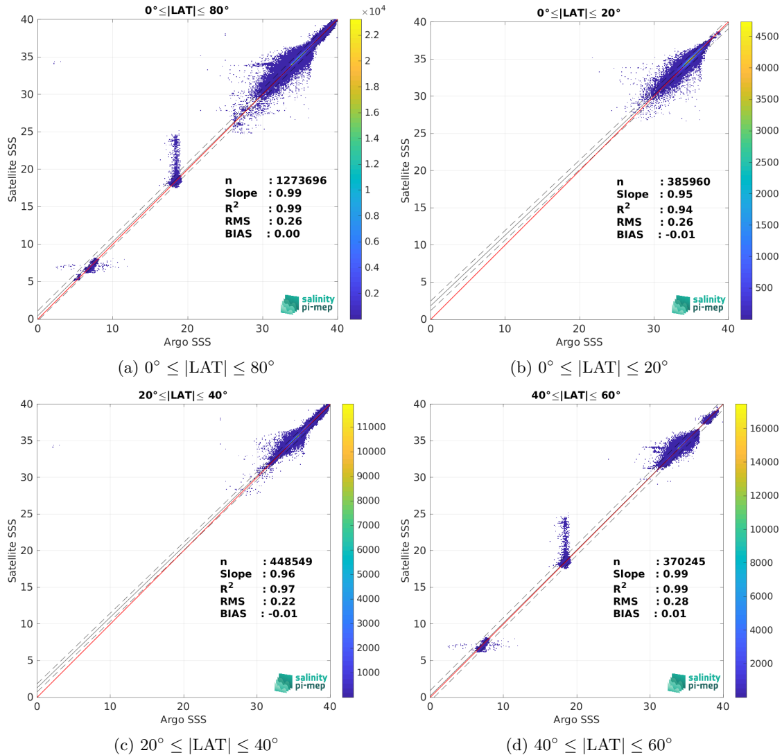
Figure 9: Contour maps of the concentration of SMAP SSS L4 OI v2 - Monthly (IPRC) SSS (y-axis) versus Argo SSS (x-axis) at match-up pairs for different latitude bands. For each plot, the red line shows x=y . The black thin and dashed lines indicate a linear fit through the data cloud and the \pm 95\% confidence levels, respectively. The number match-up pairs n , the slope and R^2 coefficient of the linear fit, the root mean square (RMS) and the mean bias between satellite and in situ data are indicated for each latitude band in each plots.
