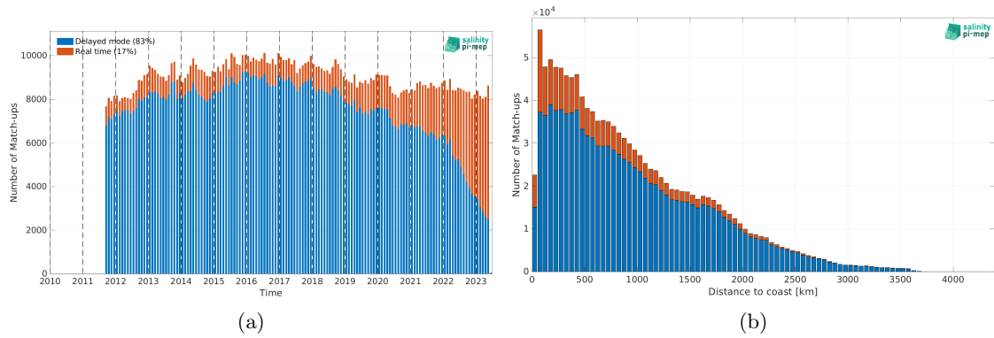
Figure 1: Number of match-ups between Argo and SMAP SSS L4 OI v2 - Monthly (IPRC) SSS as a function of time (a) and as function of the distance to coast (b) over the Global Ocean Pi-MEP region and for the full satellite product period.
