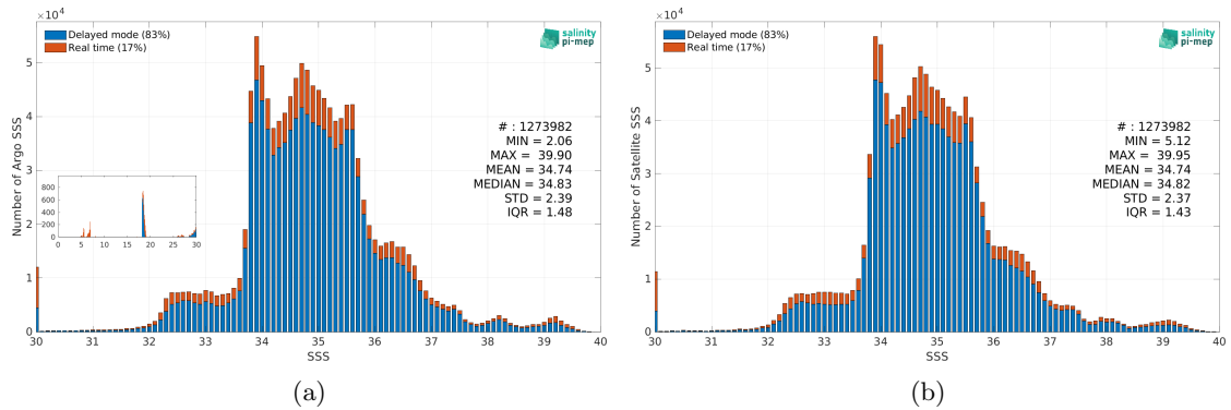
Figure 2: Histograms of SSS from Argo (a) and SMAP SSS L4 OI v2 - Monthly (IPRC) (b) considering all match-up pairs per bins of 0.1 over the Global Ocean Pi-MEP region and for the full satellite product period.
