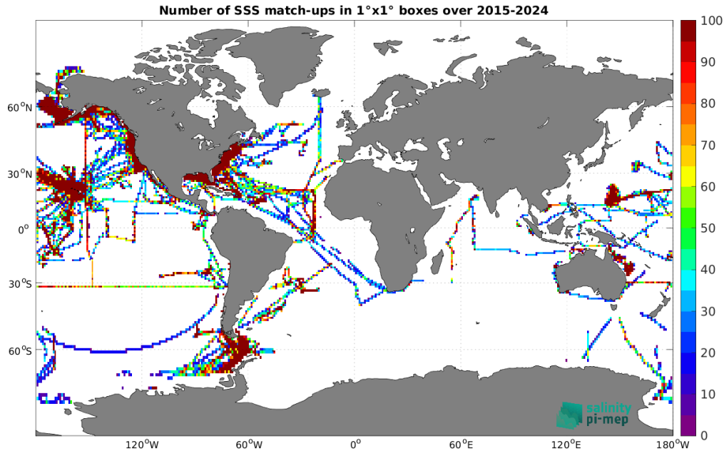
Figure 5: Number of SSS match-ups between TSG (SAMOS) SSS and the SMAP SSS L3 v6 - 8-Day running (RSS) SSS product for the Global Ocean Pi-MEP region over 1^\circ \times 1^\circ boxes and for the full satellite product period.
