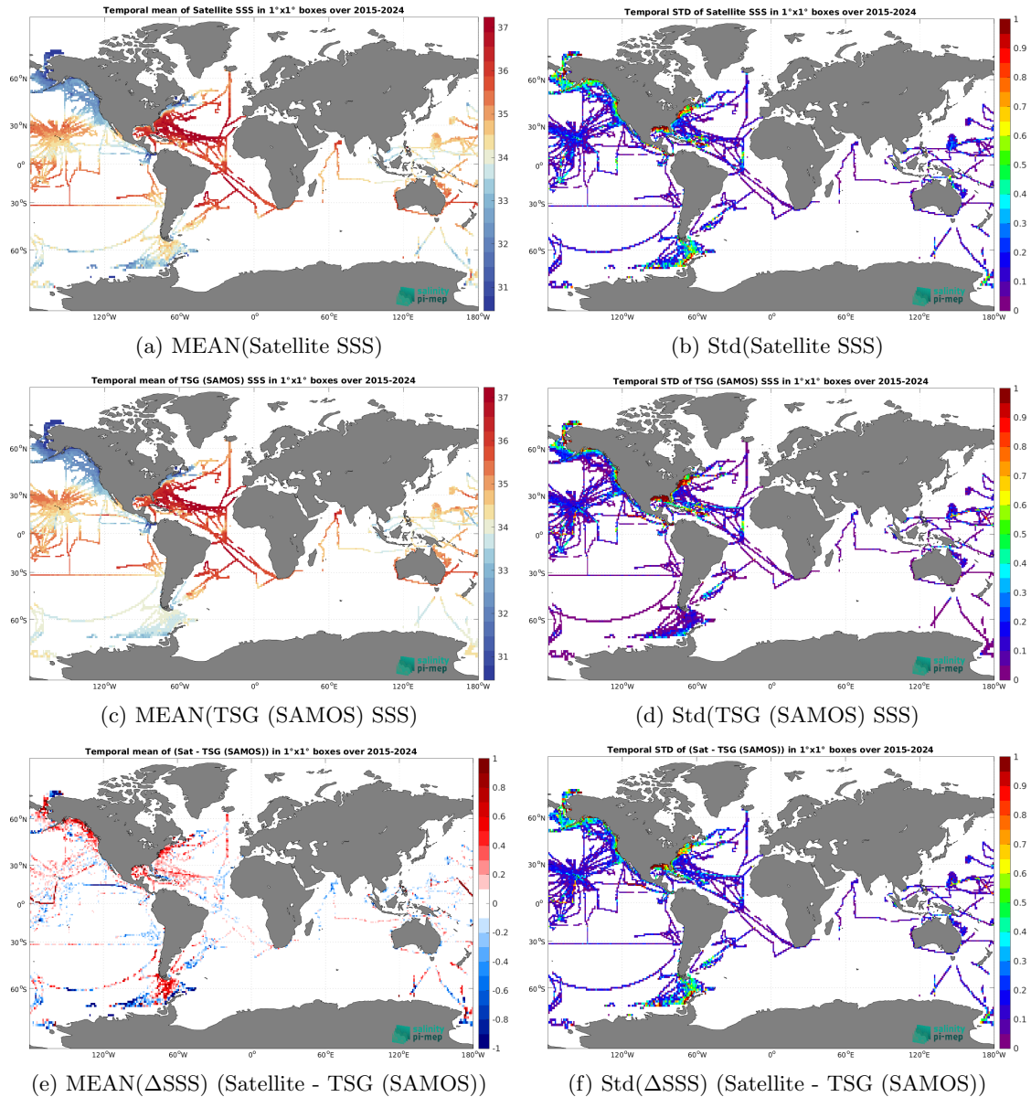
Figure 7: Temporal mean (left) and Std (right) of SSS from SMAP SSS L3 v6 - 8-Day running (RSS) (top), TSG (SAMOS) (middle), and of \Delta SSS (Satellite - TSG (SAMOS)). Only match-up pairs are used to generate these maps.
