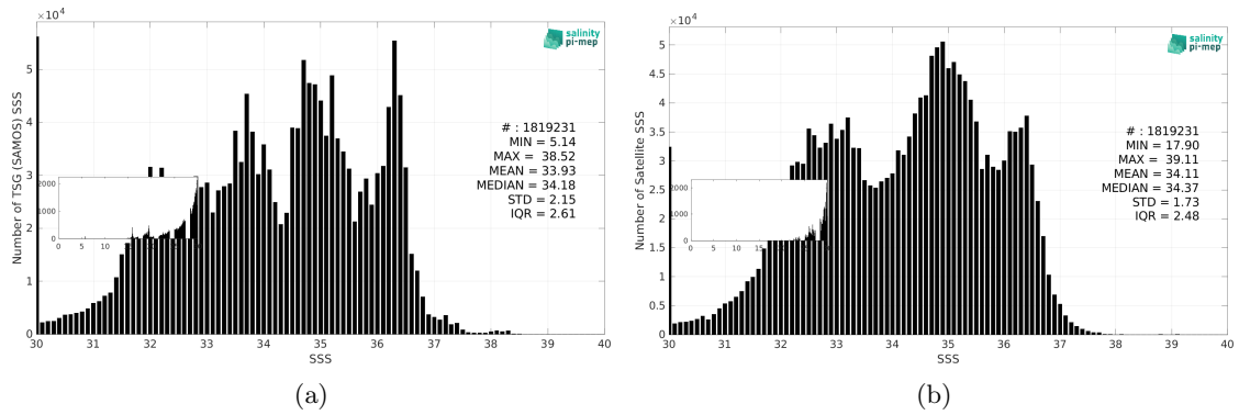
Figure 3: Histograms of SSS from TSG (SAMOS) (a) and SMAP SSS L3 v6 - 8-Day running (RSS) (b) considering all match-up pairs per bins of 0.1 over the Global Ocean Pi-MEP region and for the full satellite product period.
