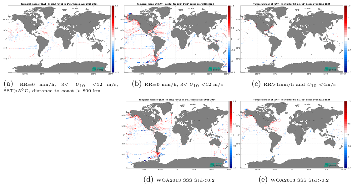
Figure 14: Temporal mean gridded over spatial boxes of size 1^\circ \times 1^\circ of \Delta SSS (SMAP SSS L3 v6 - 8-Day running (RSS) - TSG (SAMOS)) for 5 different subdatasets corresponding to:RR=0 mm/h, 3 < U_{10} < 12 m/s, SST > 5^\circ\text{C} , distance to coast > 800 km (a), RR=0 mm/h, 3 < U_{10} < 12 m/s (b), RR > 1 mm/h and U_{10} < 4 m/s (c), WOA2013 SSS Std < 0.2 (d), WOA2013 SSS Std > 0.2 (e).
