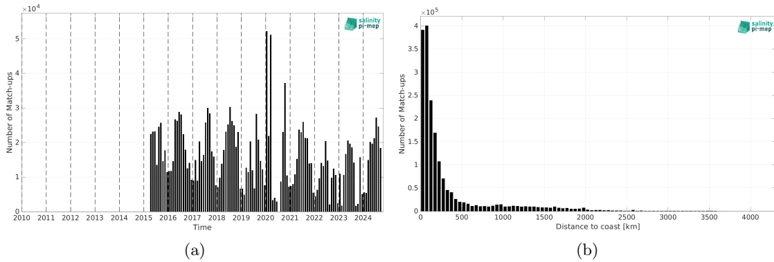
Figure 2: Number of match-ups between TSG (SAMOS) and SMAP SSS L3 v6 - 8-Day running (RSS) SSS as a function of time (a) and as function of the distance to coast (b) over the Global Ocean Pi-MEP region and for the full satellite product period.
