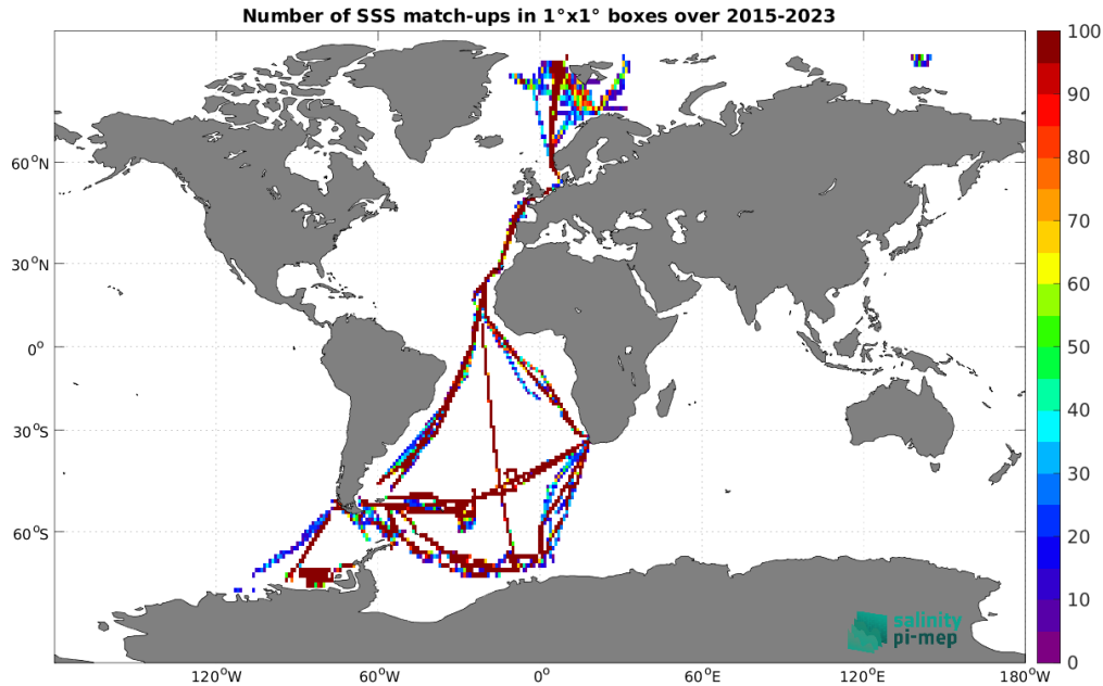
Figure 5: Number of SSS match-ups between TSG (Polarstern) SSS and the SMAP SSS L3 v6 - 8-Day running (RSS) SSS product for the Global Ocean Pi-MEP region over 1°×1° boxes and for the full satellite product period.
