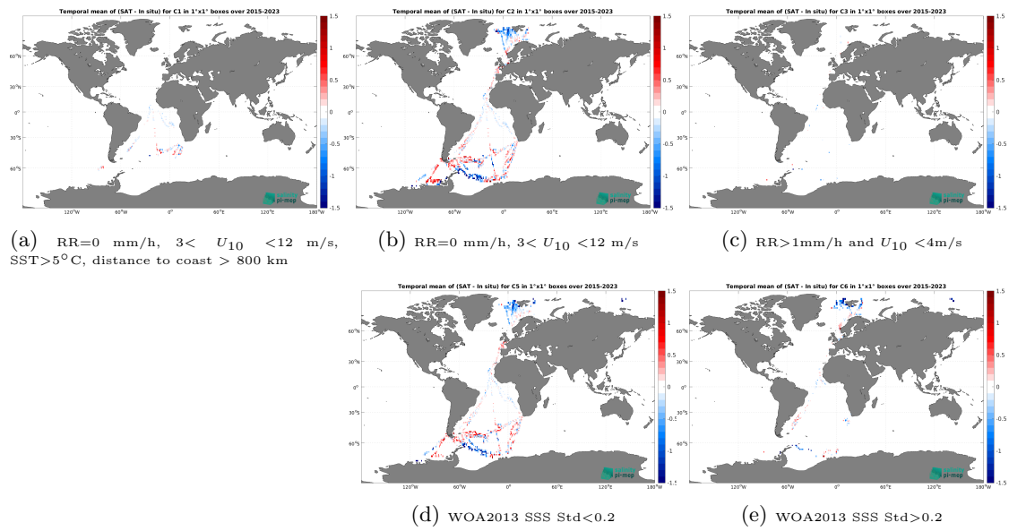
Figure 14: Temporal mean gridded over spatial boxes of size 1^\circ \times 1^\circ of \Delta SSS (SMAP SSS L3 v6 - 8-Day running (RSS) - TSG (Polarstern)) for 5 different subdatasets corresponding to:RR=0 mm/h, 3 < U_{10} < 12 m/s, SST > 5^\circ\text{C} , distance to coast > 800 km (a), RR=0 mm/h, 3 < U_{10} < 12 m/s (b), RR > 1 mm/h and U_{10} < 4 m/s (c), WOA2013 SSS Std < 0.2 (d), WOA2013 SSS Std > 0.2 (e).
