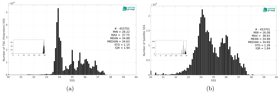
Figure 3: Histograms of SSS from TSG (Polarstern) (a) and SMAP SSS L3 v6 - 8-Day running (RSS) (b) considering all match-up pairs per bins of 0.1 over the Global Ocean Pi-MEP region and for the full satellite product period.
