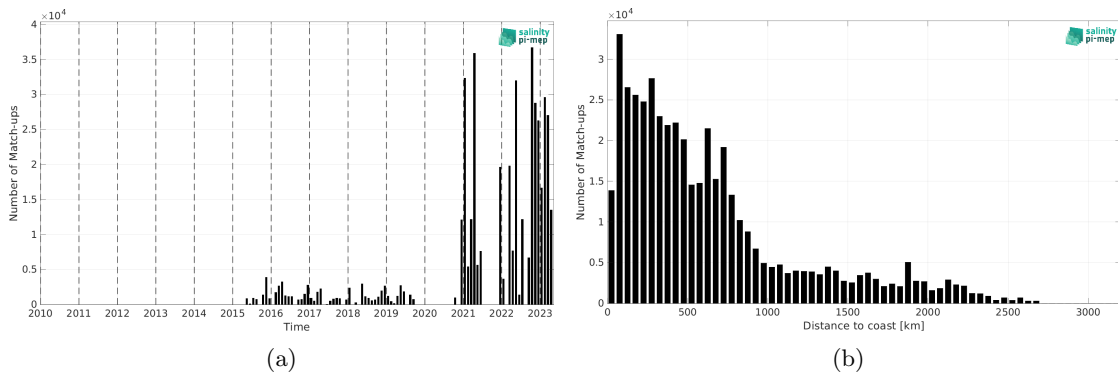
Figure 2: Number of match-ups between TSG (Polarstern) and SMAP SSS L3 v6 - 8-Day running (RSS) SSS as a function of time (a) and as function of the distance to coast (b) over the Global Ocean Pi-MEP region and for the full satellite product period.
