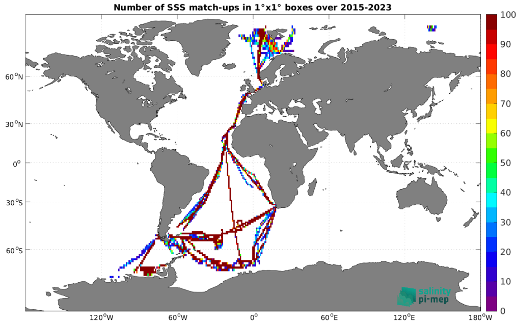
Figure 5: Number of SSS match-ups between TSG (Polarstern) SSS and the SMAP SSS L3 v6 - 8-Day running (RSS) SSS product for the Global Ocean Pi-MEP region over 1^\circ \times 1^\circ boxes and for the full satellite product period.
