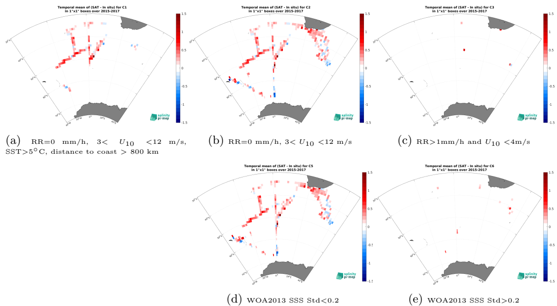
Figure 14: Temporal mean gridded over spatial boxes of size 1^\circ \times 1^\circ of \Delta\text{SSS} (SMAP SSS L3 v6 - 8-Day running (RSS) - TSG (NCEI-0170743)) for 5 different subdatasets corresponding to: RR=0 mm/h, 3 < U_{10} < 12 m/s, SST > 5^\circ\text{C} , distance to coast > 800 km (a), RR=0 mm/h, 3 < U_{10} < 12 m/s (b), RR > 1 mm/h and U_{10} < 4 m/s (c), WOA2013 SSS Std < 0.2 (d), WOA2013 SSS Std > 0.2 (e).
