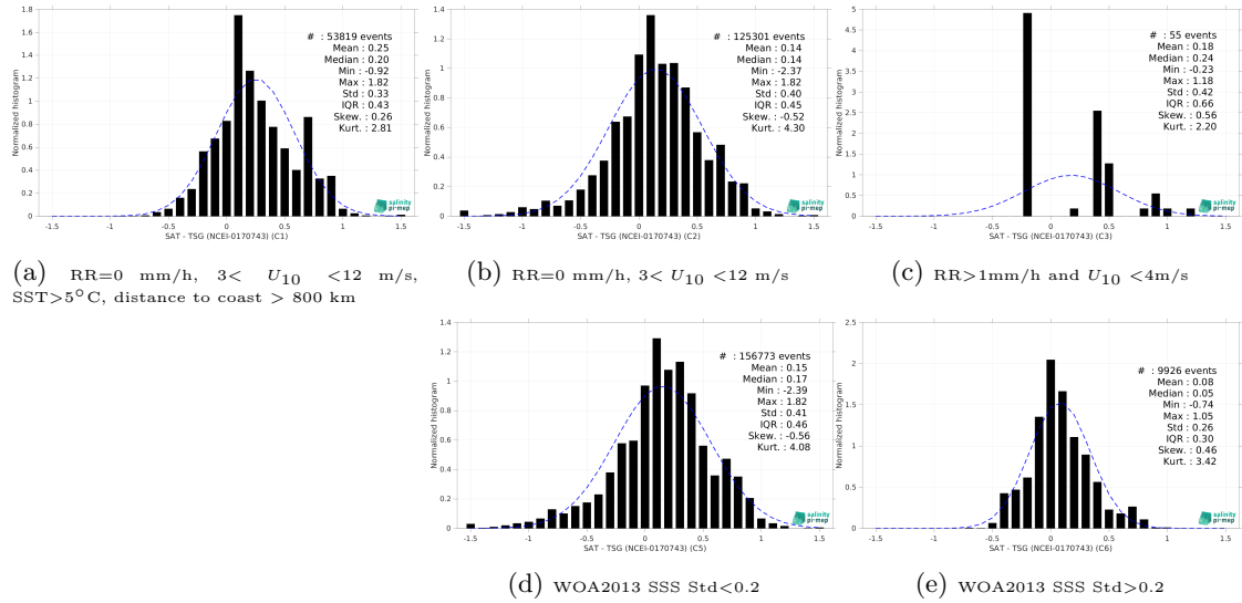
Figure 15: Normalized histogram of \Delta SSS (SMAP SSS L3 v6 - 8-Day running (RSS) - TSG (NCEI-0170743)) for 5 different subdatasets corresponding to: RR=0 mm/h, 3 < U_{10} < 12 m/s, SST > 5°C, distance to coast > 800 km (a), RR=0 mm/h, 3 < U_{10} < 12 m/s (b), RR > 1mm/h and U_{10} < 4 m/s (c), WOA2013 SSS Std < 0.2 (d), WOA2013 SSS Std > 0.2 (e).
