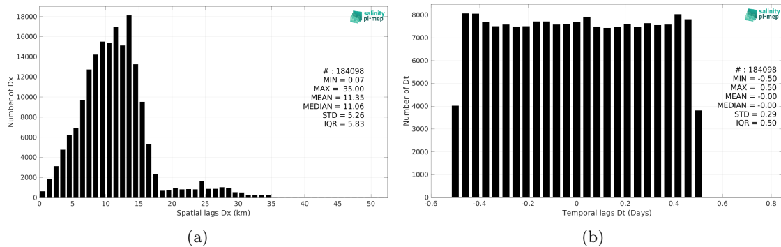
Figure 6: Histograms of the spatial (a) and temporal (b) lags between the location/time of the TSG (NCEI-0170743) measurement and the date of the corresponding SMAP SSS L3 v6 - 8-Day running (RSS) SSS pixel.
