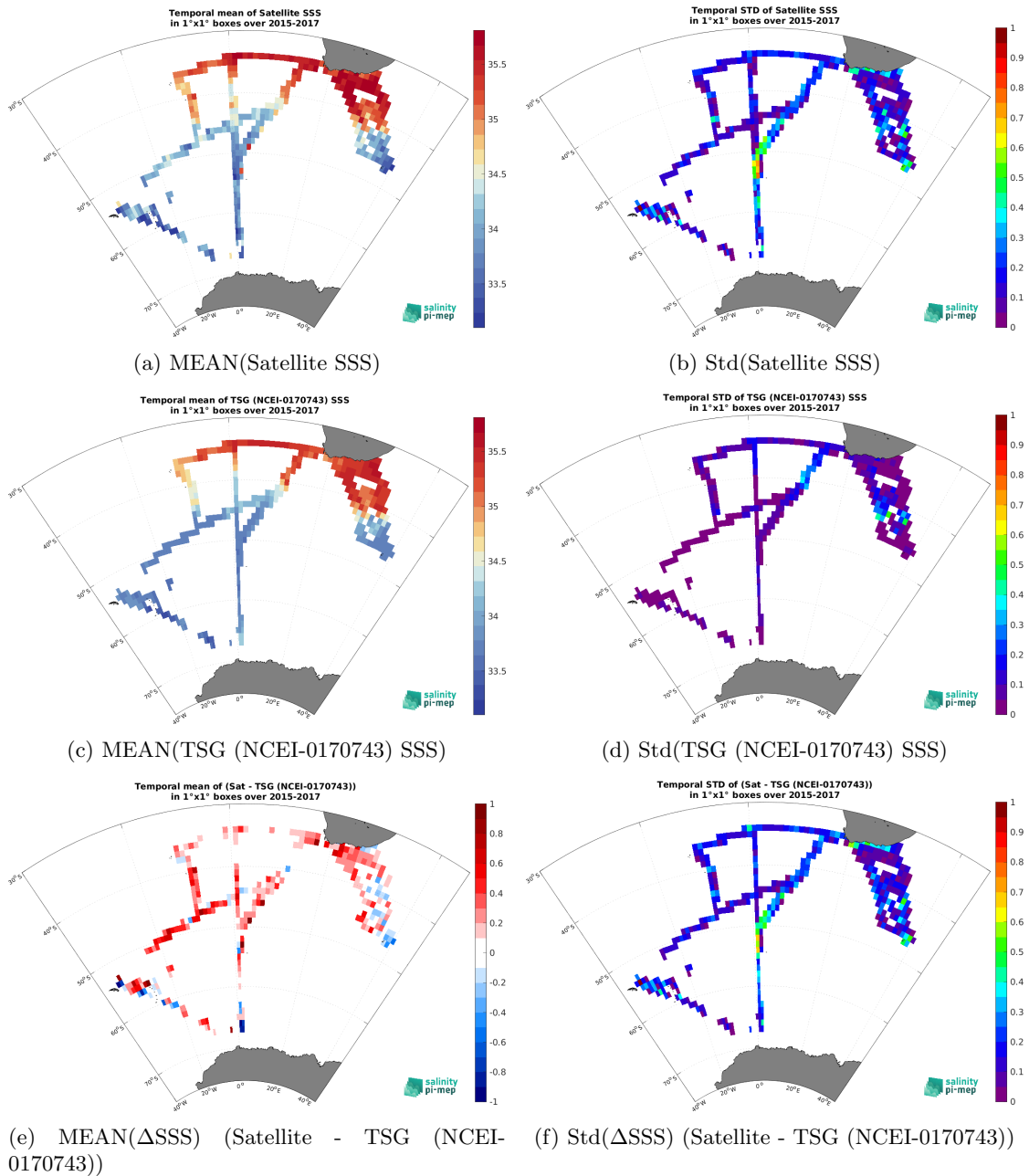
Figure 7: Temporal mean (left) and Std (right) of SSS from SMAP SSS L3 v6 - 8-Day running (RSS) (top), TSG (NCEI-0170743) (middle), and of \Delta SSS (Satellite - TSG (NCEI-0170743)). Only match-up pairs are used to generate these maps.
