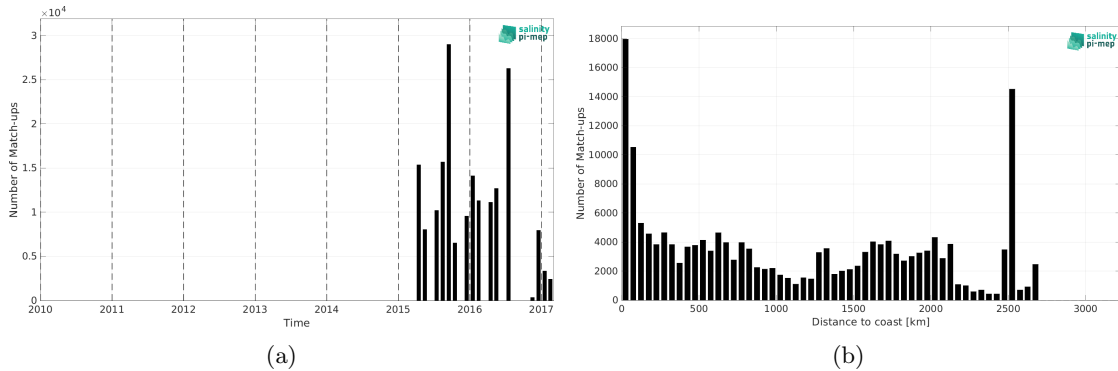
Figure 2: Number of match-ups between TSG (NCEI-0170743) and SMAP SSS L3 v6 - 8-Day running (RSS) SSS as a function of time (a) and as function of the distance to coast (b) over the Global Ocean Pi-MEP region and for the full satellite product period.
