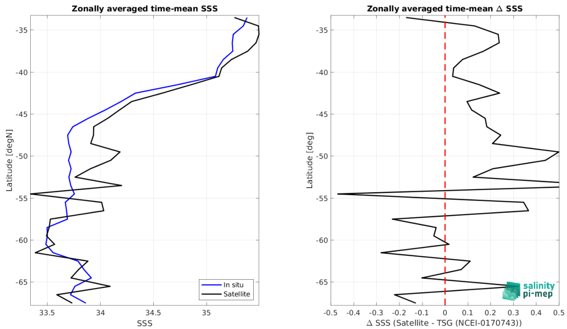
Figure 9: Left panel: Zonal mean SSS from SMAP SSS L3 v6 - 8-Day running (RSS) satellite product (black) and from TSG (NCEI-0170743) (blue). Right panel: Zonal mean of \Delta SSS (Satellite - TSG (NCEI-0170743)) for all the collected Pi-MEP match-up pairs estimated over the full satellite product period.
