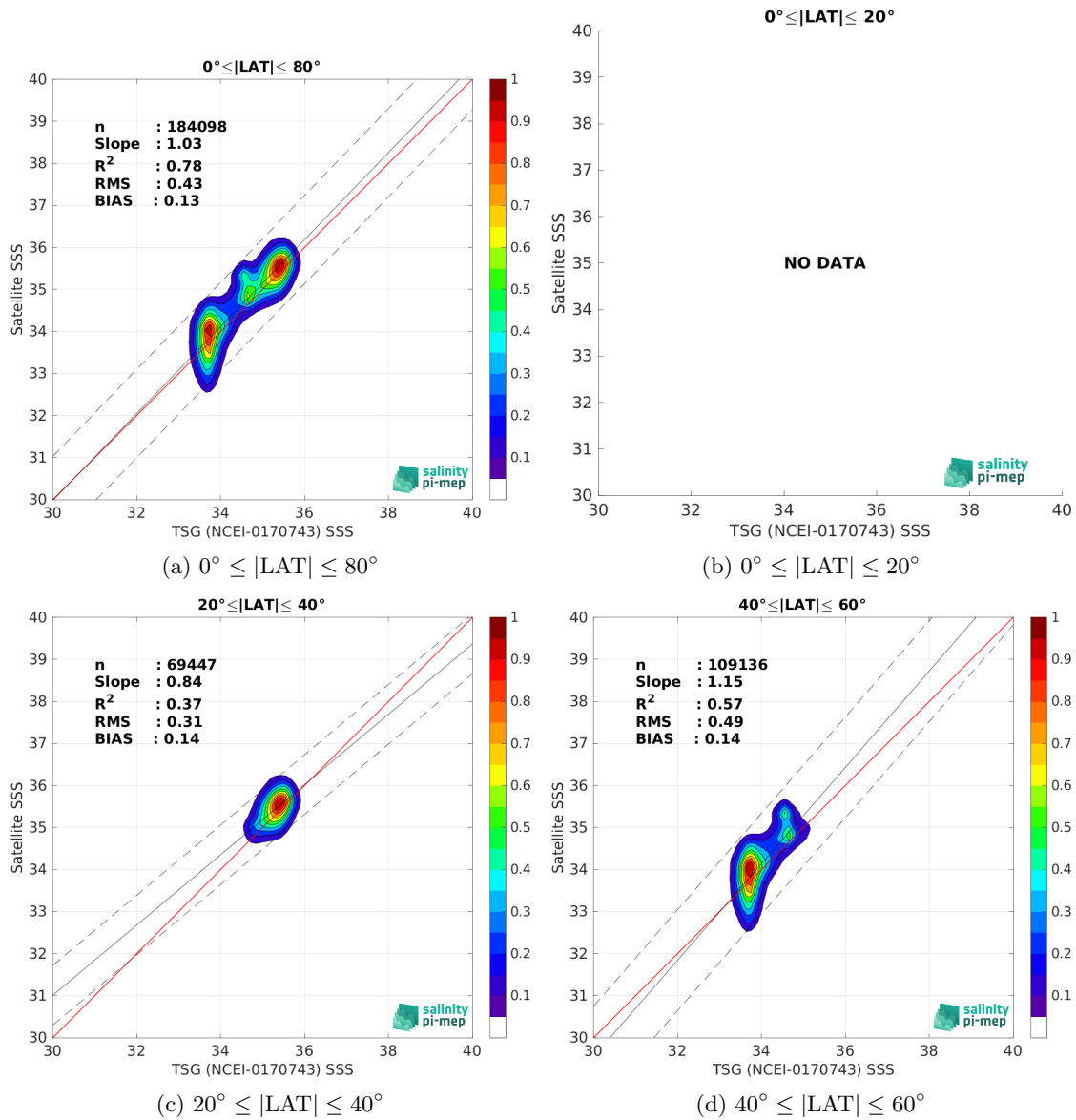
Figure 10: Contour maps of the concentration of SMAP SSS L3 v6 - 8-Day running (RSS) SSS (y-axis) versus TSG (NCEI-0170743) SSS (x-axis) at match-up pairs for different latitude bands. For each plot, the red line shows x=y . The black thin and dashed lines indicate a linear fit through the data cloud and the \pm 95\% confidence levels, respectively. The number match-up pairs n , the slope and R^2 coefficient of the linear fit, the root mean square (RMS) and the mean bias between satellite and in situ data are indicated for each latitude band in each plots.
