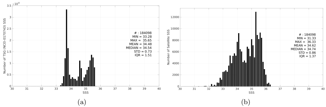
Figure 3: Histograms of SSS from TSG (NCEI-0170743) (a) and SMAP SSS L3 v6 - 8-Day running (RSS) (b) considering all match-up pairs per bins of 0.1 over the Global Ocean Pi-MEP region and for the full satellite product period.
