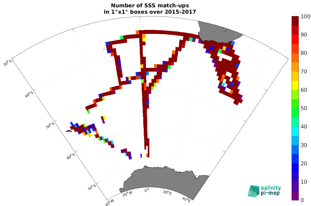
Figure 5: Number of SSS match-ups between TSG (NCEI-0170743) SSS and the SMAP SSS L3 v6 - 8-Day running (RSS) SSS product for the Global Ocean Pi-MEP region over 1^{\circ} \times 1^{\circ} boxes and for the full satellite product period.
