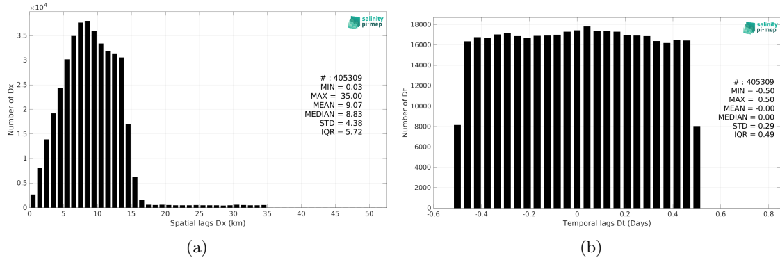
Figure 6: Histograms of the spatial (a) and temporal (b) lags between the location/time of the TSG (LEGOS-Survostral) measurement and the date of the corresponding SMAP SSS L3 v6 - 8-Day running (RSS) SSS pixel.
