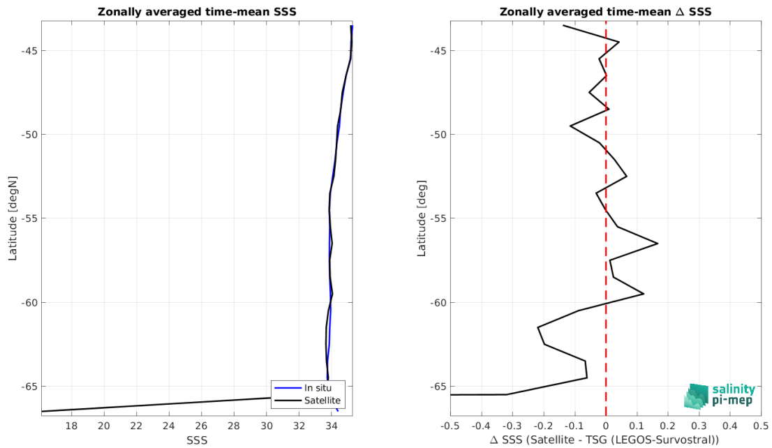
Figure 9: Left panel: Zonal mean SSS from SMAP SSS L3 v6 - 8-Day running (RSS) satellite product (black) and from TSG (LEGOS-Survostral) (blue). Right panel: Zonal mean of \Delta SSS (Satellite - TSG (LEGOS-Survostral)) for all the collected Pi-MEP match-up pairs estimated over the full satellite product period.
