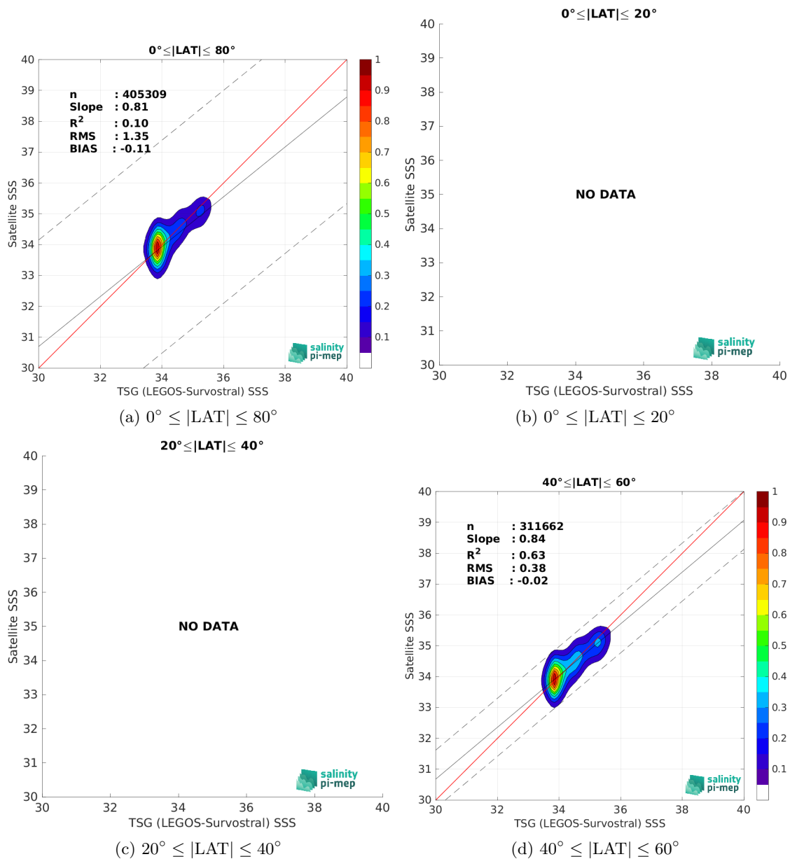
Figure 10: Contour maps of the concentration of SMAP SSS L3 v6 - 8-Day running (RSS) SSS (y-axis) versus TSG (LEGOS-Survostral) SSS (x-axis) at match-up pairs for different latitude bands. For each plot, the red line shows x=y . The black thin and dashed lines indicate a linear fit through the data cloud and the \pm 95\% confidence levels, respectively. The number match-up pairs n , the slope and R^2 coefficient of the linear fit, the root mean square (RMS) and the mean bias between satellite and in situ data are indicated for each latitude band in each plots.
