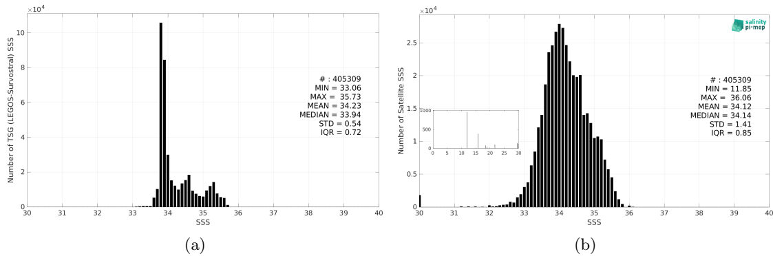
Figure 3: Histograms of SSS from TSG (LEGOS-Survostral) (a) and SMAP SSS L3 v6 - 8-Day running (RSS) (b) considering all match-up pairs per bins of 0.1 over the Global Ocean Pi-MEP region and for the full satellite product period.
