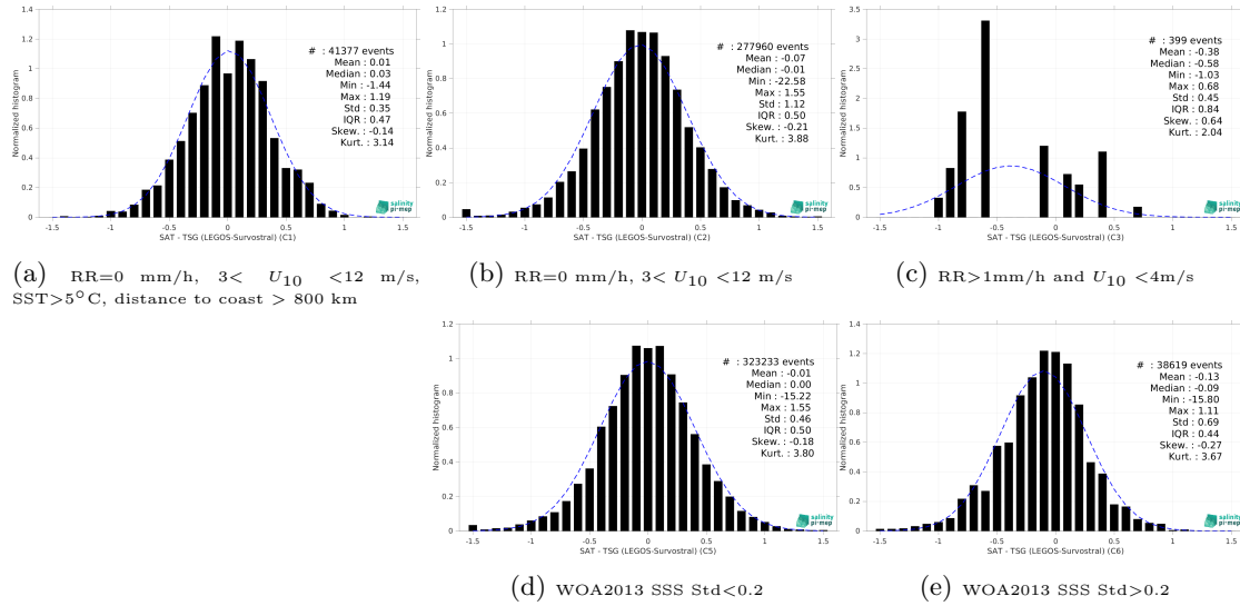
Figure 15: Normalized histogram of \Delta SSS (SMAP SSS L3 v6 - 8-Day running (RSS) - TSG (LEGOS-Survostral)) for 5 different subdatasets corresponding to: RR=0 mm/h, 3 < U_{10} < 12 m/s, SST > 5°C, distance to coast > 800 km (a), RR=0 mm/h, 3 < U_{10} < 12 m/s (b), RR > 1mm/h and U_{10} < 4 m/s (c), WOA2013 SSS Std < 0.2 (d), WOA2013 SSS Std > 0.2 (e).
