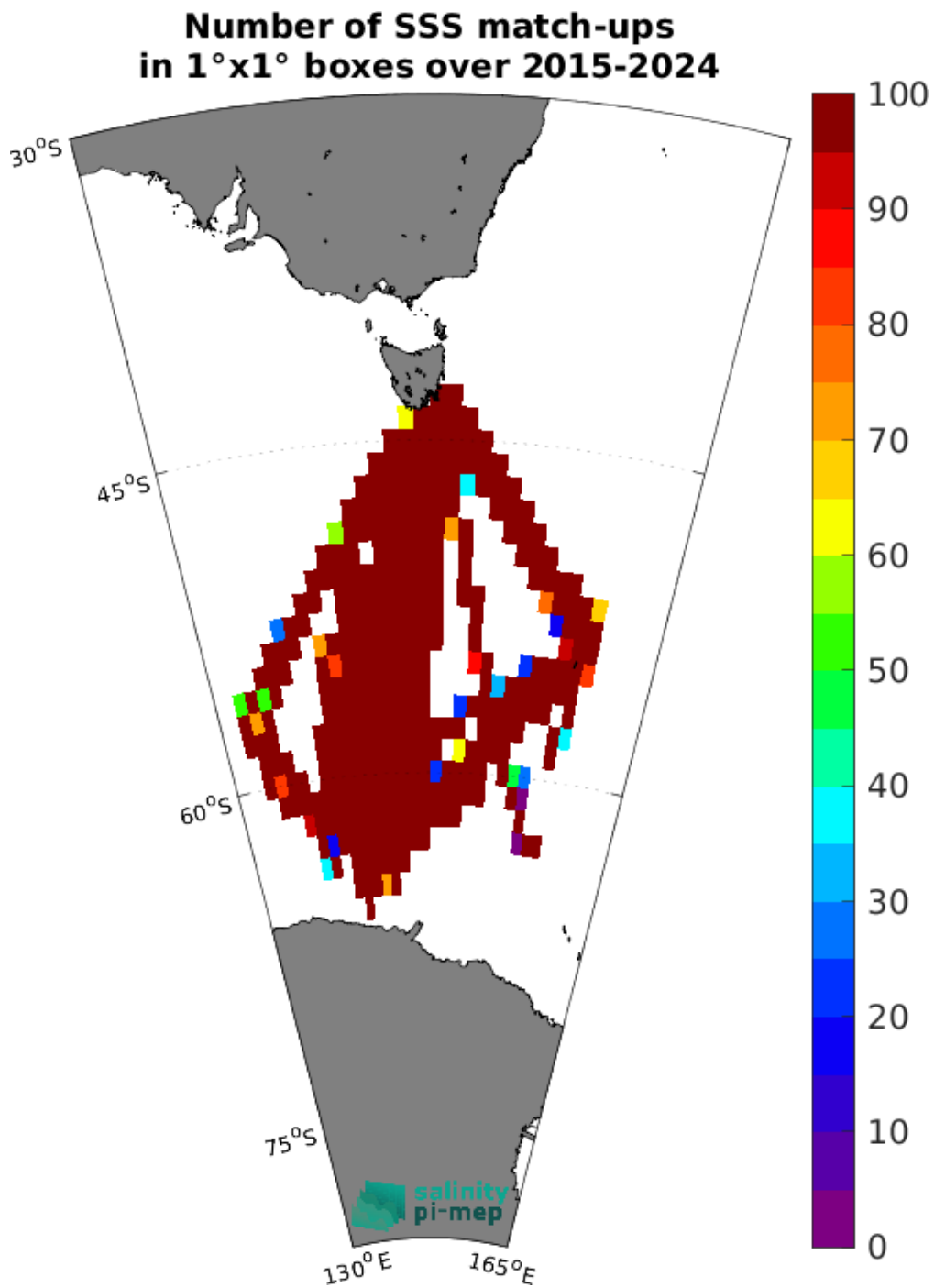
Figure 5: Number of SSS match-ups between TSG (LEGOS-Survostral) SSS and the SMAP SSS L3 v6 - 8-Day running (RSS) SSS product for the Global Ocean Pi-MEP region over 1°x1° boxes and for the full satellite product period.
