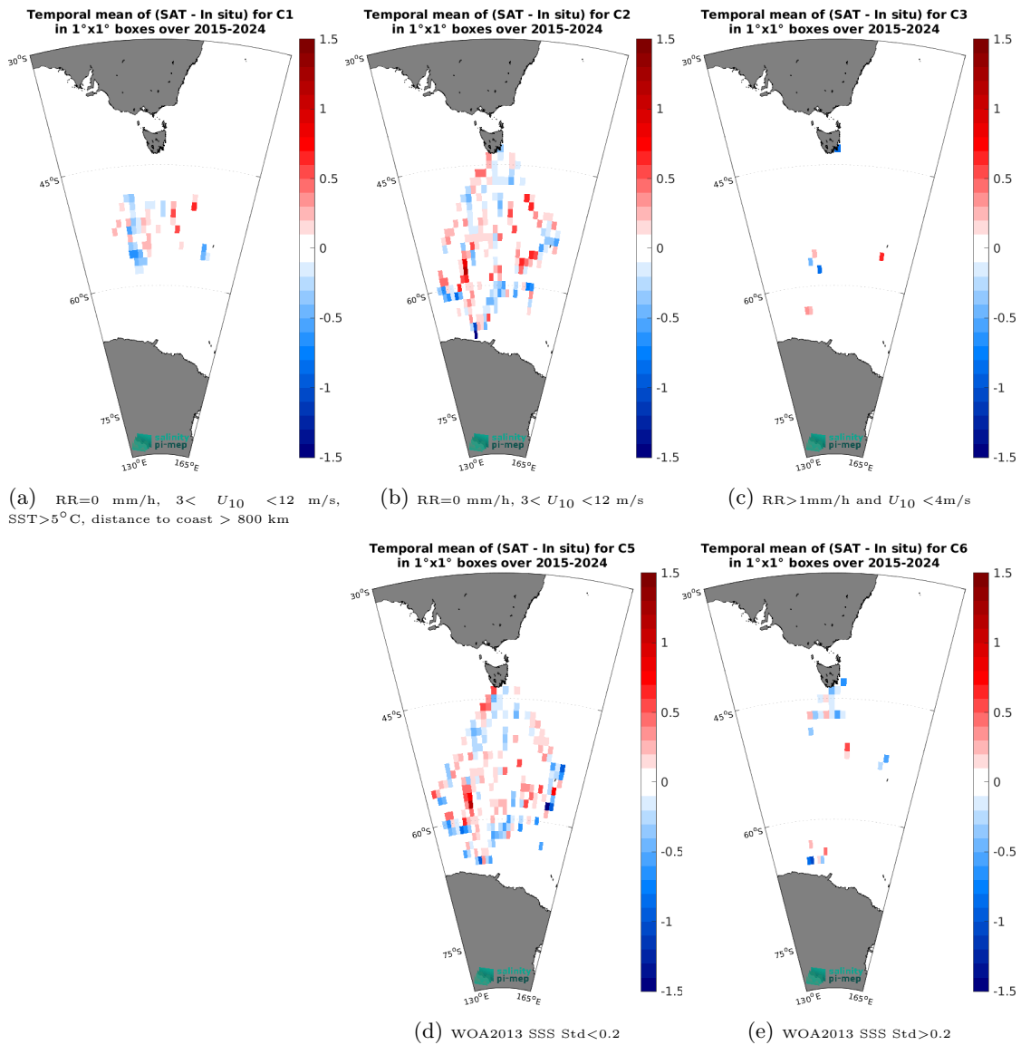
Figure 14: Temporal mean gridded over spatial boxes of size 1^\circ \times 1^\circ of \Delta SSS (SMAP SSS L3 v6 - 8-Day running (RSS) - TSG (LEGOS-Survostral)) for 5 different subdatasets corresponding to:RR=0 mm/h, 3 < U_{10} < 12 m/s, SST>5°C, distance to coast > 800 km (a), RR=0 mm/h, 3 < U_{10} < 12 m/s (b), RR>1mm/h and U_{10} < 4 m/s (c), WOA2013 SSS Std<0.2 (d), WOA2013 SSS Std>0.2 (e).
