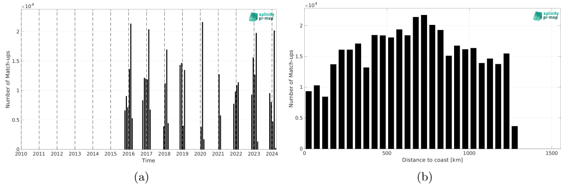
Figure 2: Number of match-ups between TSG (LEGOS-Survostral) and SMAP SSS L3 v6 - 8-Day running (RSS) SSS as a function of time (a) and as function of the distance to coast (b) over the Global Ocean Pi-MEP region and for the full satellite product period.
