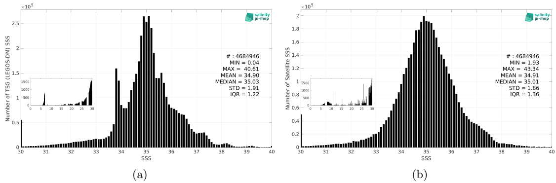
Figure 3: Histograms of SSS from TSG (LEGOS-DM) (a) and SMAP SSS L3 v6 - 8-Day running (RSS) (b) considering all match-up pairs per bins of 0.1 over the Global Ocean Pi-MEP region and for the full satellite product period.
