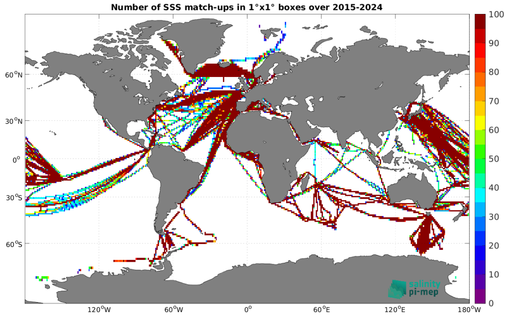
Figure 5: Number of SSS match-ups between TSG (LEGOS-DM) SSS and the SMAP SSS L3 v6 - 8-Day running (RSS) SSS product for the Global Ocean Pi-MEP region over 1^\circ \times 1^\circ boxes and for the full satellite product period.
