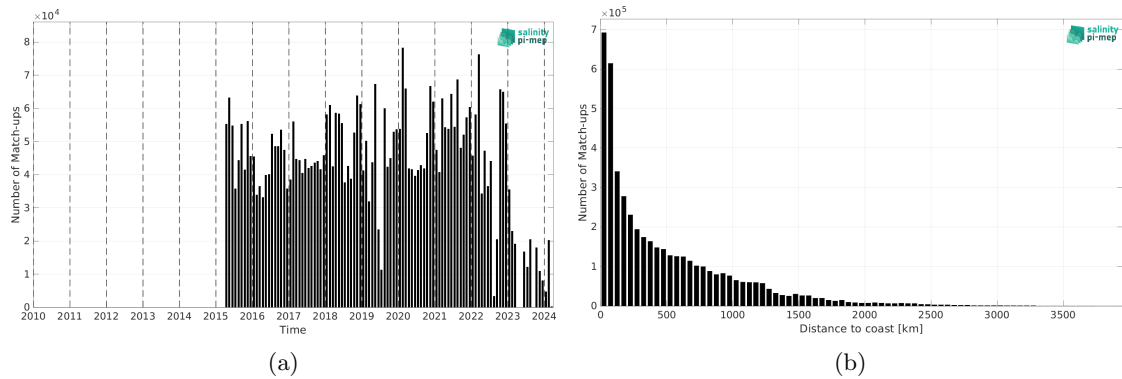
Figure 2: Number of match-ups between TSG (LEGOS-DM) and SMAP SSS L3 v6 - 8-Day running (RSS) SSS as a function of time (a) and as function of the distance to coast (b) over the Global Ocean Pi-MEP region and for the full satellite product period.
