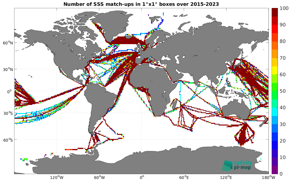
Figure 5: Number of SSS match-ups between TSG (LEGOS-DM) SSS and the SMAP SSS L3 v6 - 8-Day running (RSS) SSS product for the Global Ocean Pi-MEP region over 1°x1° boxes and for the full satellite product period.
