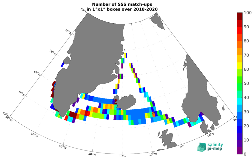
Figure 5: Number of SSS match-ups between TSG (Lauge-Koch) SSS and the SMAP SSS L3 v6 - 8-Day running (RSS) SSS product for the Global Ocean Pi-MEP region over 1^\circ \times 1^\circ boxes and for the full satellite product period.
