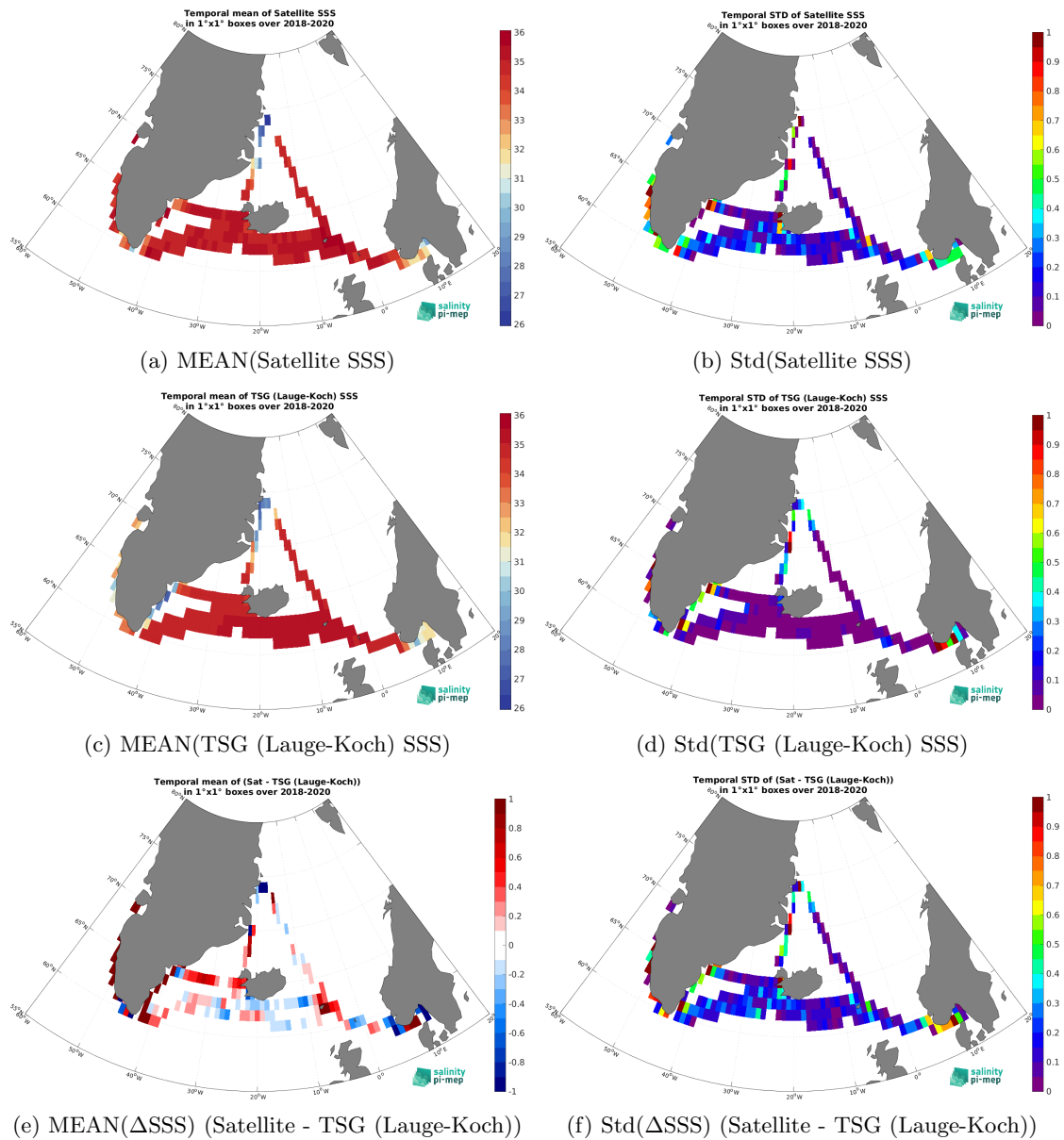
Figure 7: Temporal mean (left) and Std (right) of SSS from SMAP SSS L3 v6 - 8-Day running (RSS) (top), TSG (Lauge-Koch) (middle), and of \Delta SSS (Satellite - TSG (Lauge-Koch)). Only match-up pairs are used to generate these maps.
