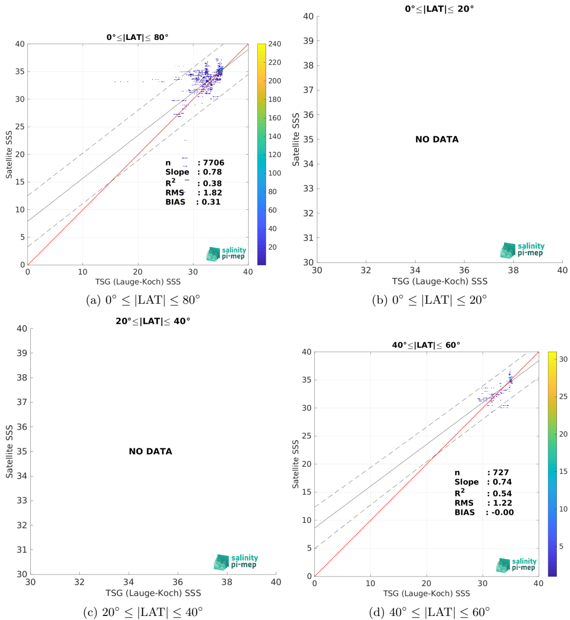
Figure 10: Contour maps of the concentration of SMAP SSS L3 v6 - 8-Day running (RSS) SSS (y-axis) versus TSG (Lauge-Koch) SSS (x-axis) at match-up pairs for different latitude bands. For each plot, the red line shows x=y . The black thin and dashed lines indicate a linear fit through the data cloud and the \pm 95\% confidence levels, respectively. The number match-up pairs n , the slope and R^2 coefficient of the linear fit, the root mean square (RMS) and the mean bias between satellite and in situ data are indicated for each latitude band in each plots.
