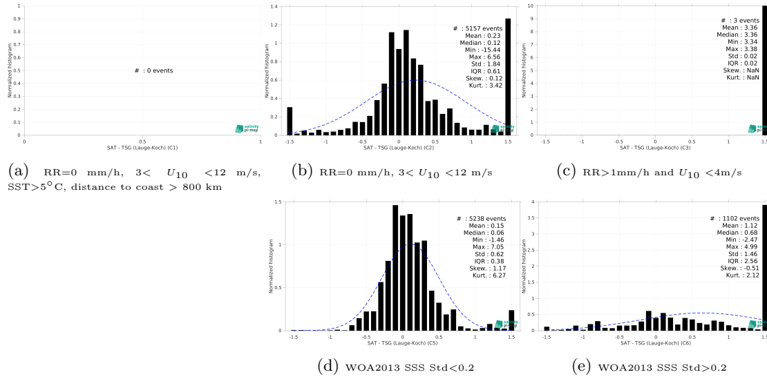
Figure 15: Normalized histogram of \Delta SSS (SMAP SSS L3 v6 - 8-Day running (RSS) - TSG (Lauge-Koch)) for 5 different subdatasets corresponding to: RR=0 mm/h, 3 < U_{10} < 12 m/s, SST>5°C, distance to coast > 800 km (a), RR=0 mm/h, 3 < U_{10} < 12 m/s (b), RR>1mm/h and U_{10} < 4 m/s (c), WOA2013 SSS Std<0.2 (d), WOA2013 SSS Std>0.2 (e).
