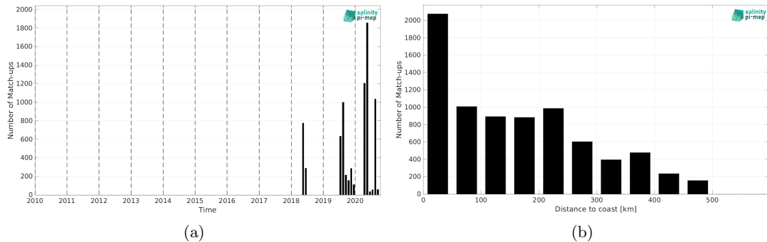
Figure 2: Number of match-ups between TSG (Lauge-Koch) and SMAP SSS L3 v6 - 8-Day running (RSS) SSS as a function of time (a) and as function of the distance to coast (b) over the Global Ocean Pi-MEP region and for the full satellite product period.
