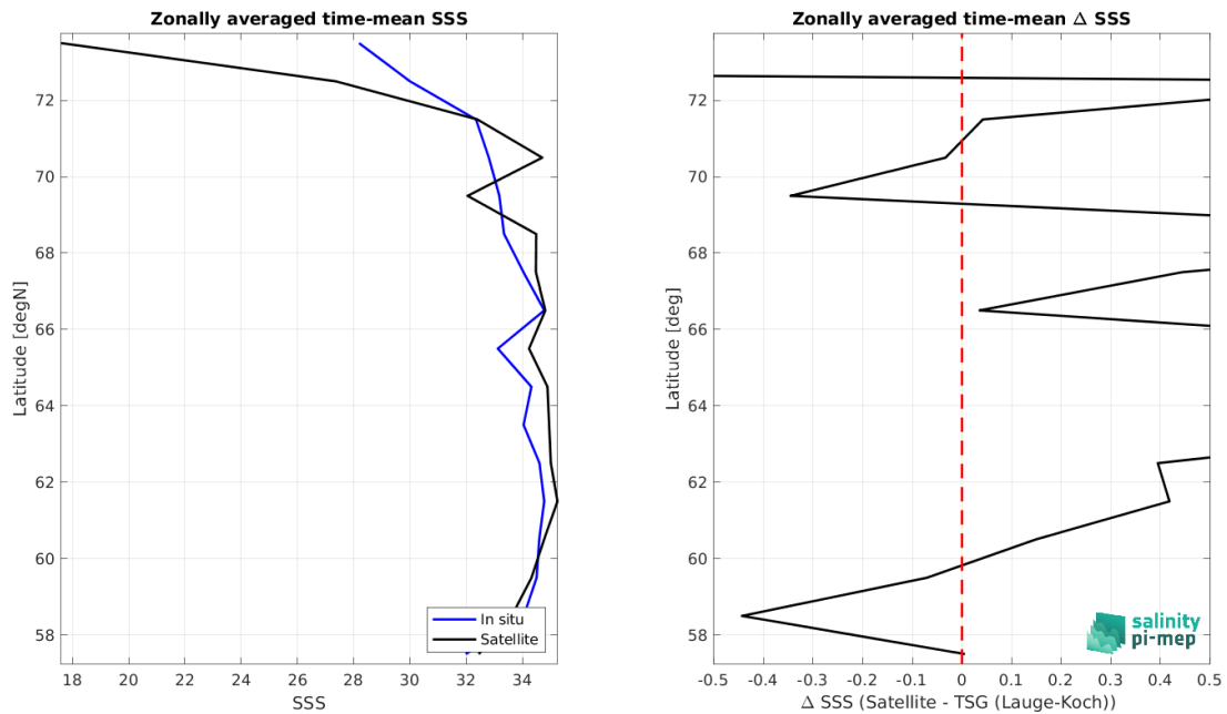
Figure 9: Left panel: Zonal mean SSS from SMAP SSS L3 v6 - 8-Day running (RSS) satellite product (black) and from TSG (Lauge-Koch) (blue). Right panel: Zonal mean of \Delta SSS (Satellite - TSG (Lauge-Koch)) for all the collected Pi-MEP match-up pairs estimated over the full satellite product period.
