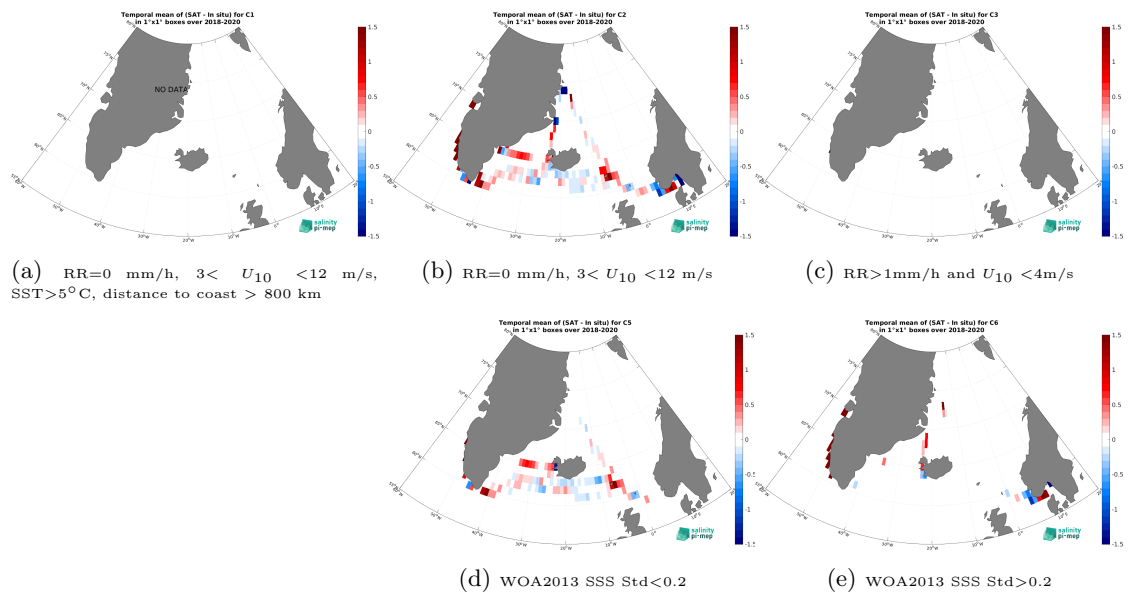
Figure 14: Temporal mean gridded over spatial boxes of size 1^\circ \times 1^\circ of \Delta SSS (SMAP SSS L3 v6 - 8-Day running (RSS) - TSG (Lauge-Koch)) for 5 different subdatasets corresponding to:RR=0 mm/h, 3 < U_{10} < 12 m/s, SST > 5^\circ\text{C} , distance to coast > 800 km (a), RR=0 mm/h, 3 < U_{10} < 12 m/s (b), RR > 1 mm/h and U_{10} < 4 m/s (c), WOA2013 SSS Std < 0.2 (d), WOA2013 SSS Std > 0.2 (e).
