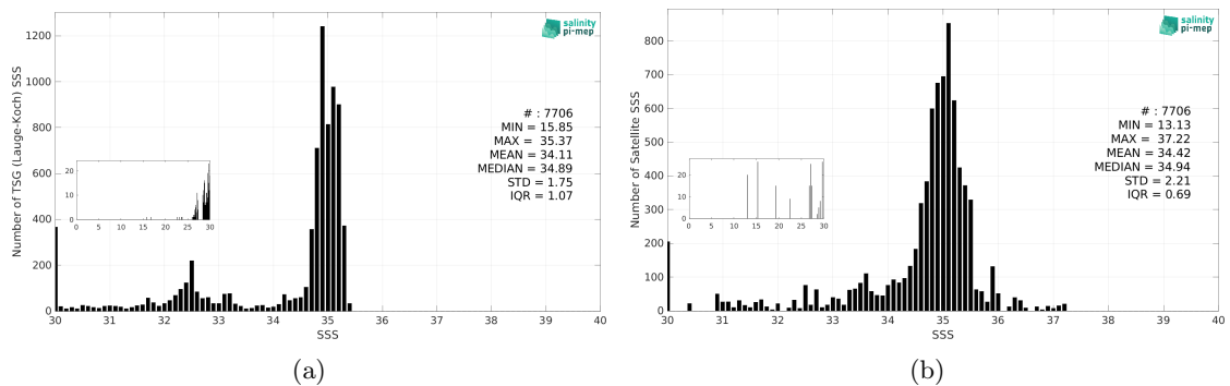
Figure 3: Histograms of SSS from TSG (Lauge-Koch) (a) and SMAP SSS L3 v6 - 8-Day running (RSS) (b) considering all match-up pairs per bins of 0.1 over the Global Ocean Pi-MEP region and for the full satellite product period.
