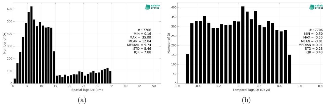
Figure 6: Histograms of the spatial (a) and temporal (b) lags between the location/time of the TSG (Lauge-Koch) measurement and the date of the corresponding SMAP SSS L3 v6 - 8-Day running (RSS) SSS pixel.
