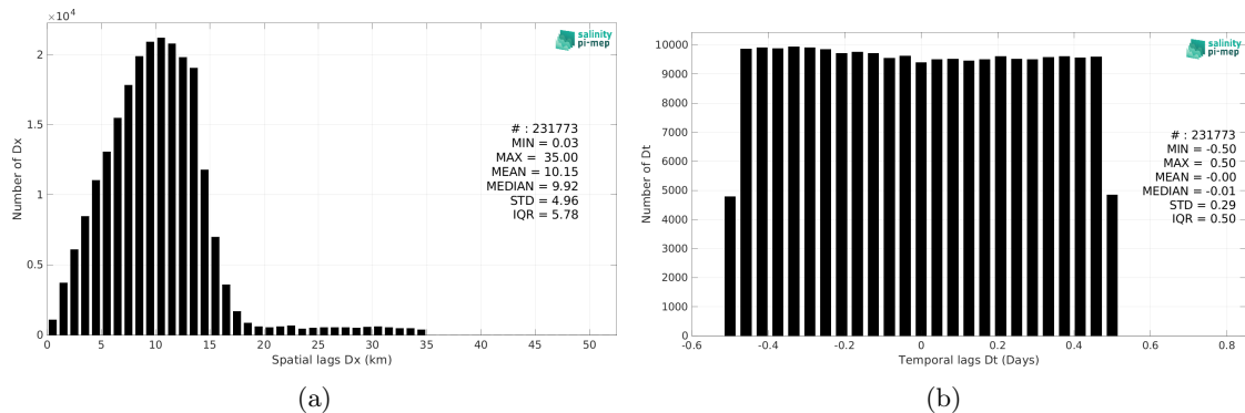
Figure 6: Histograms of the spatial (a) and temporal (b) lags between the location/time of the TSG (GOSUD-Sailing-ship) measurement and the date of the corresponding SMAP SSS L3 v6 - 8-Day running (RSS) SSS pixel.
