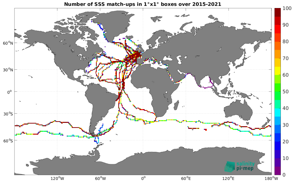
Figure 5: Number of SSS match-ups between TSG (GOSUD-Sailing-ship) SSS and the SMAP SSS L3 v6 - 8-Day running (RSS) SSS product for the Global Ocean Pi-MEP region over 1^\circ \times 1^\circ boxes and for the full satellite product period.
