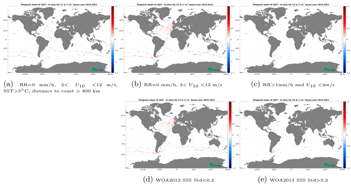
Figure 14: Temporal mean gridded over spatial boxes of size 1^\circ \times 1^\circ of \Delta SSS (SMAP SSS L3 v6 - 8-Day running (RSS) - TSG (GOSUD-Sailing-ship)) for 5 different subdatasets corresponding to: RR=0 mm/h, 3 < U_{10} < 12 m/s, SST > 5^\circ\text{C} , distance to coast > 800 km (a), RR=0 mm/h, 3 < U_{10} < 12 m/s (b), RR > 1 mm/h and U_{10} < 4 m/s (c), WOA2013 SSS Std < 0.2 (d), WOA2013 SSS Std > 0.2 (e).
