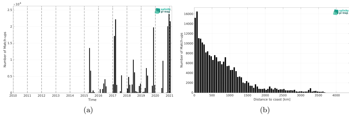
Figure 2: Number of match-ups between TSG (GOSUD-Sailing-ship) and SMAP SSS L3 v6 - 8-Day running (RSS) SSS as a function of time (a) and as function of the distance to coast (b) over the Global Ocean Pi-MEP region and for the full satellite product period.
