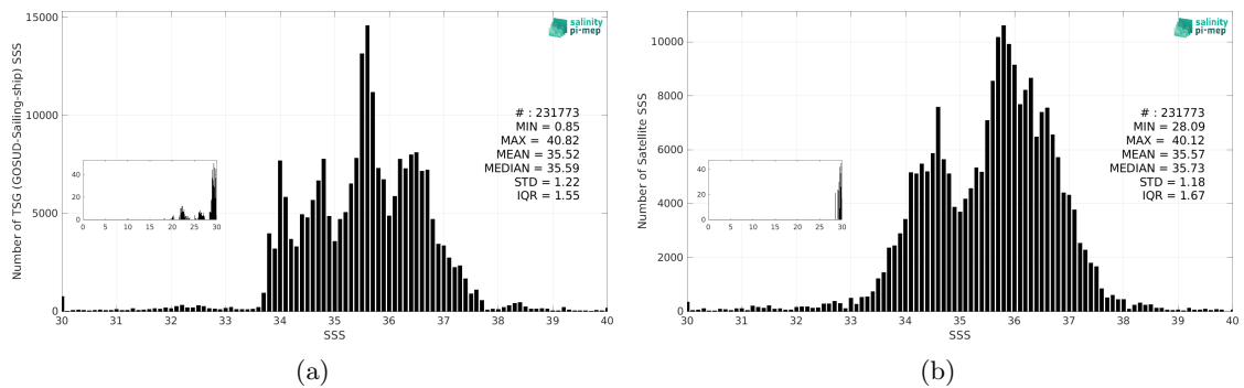
Figure 3: Histograms of SSS from TSG (GOSUD-Sailing-ship) (a) and SMAP SSS L3 v6 - 8-Day running (RSS) (b) considering all match-up pairs per bins of 0.1 over the Global Ocean Pi-MEP region and for the full satellite product period.
