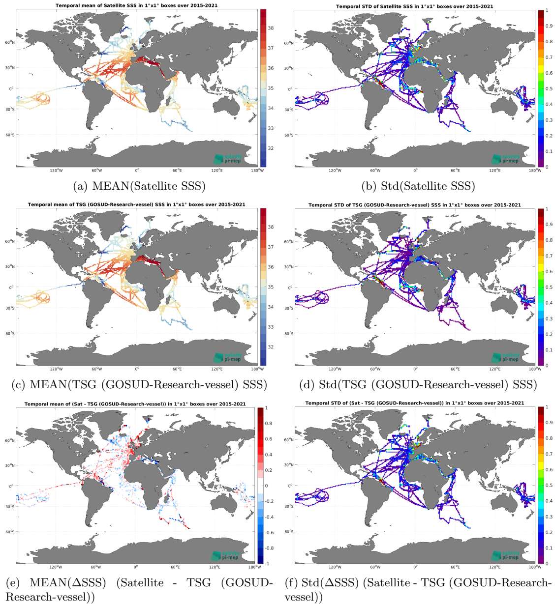
Figure 7: Temporal mean (left) and Std (right) of SSS from SMAP SSS L3 v6 - 8-Day running (RSS) (top), TSG (GOSUD-Research-vessel) (middle), and of \Delta SSS (Satellite - TSG (GOSUD-Research-vessel)). Only match-up pairs are used to generate these maps.
