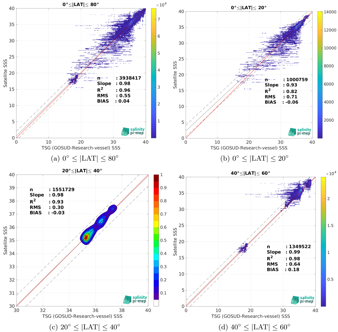
Figure 10: Contour maps of the concentration of SMAP SSS L3 v6 - 8-Day running (RSS) SSS (y-axis) versus TSG (GOSUD-Research-vessel) SSS (x-axis) at match-up pairs for different latitude bands. For each plot, the red line shows x=y . The black thin and dashed lines indicate a linear fit through the data cloud and the \pm 95\% confidence levels, respectively. The number match-up pairs n , the slope and R^2 coefficient of the linear fit, the root mean square (RMS) and the mean bias between satellite and in situ data are indicated for each latitude band in each plots.
