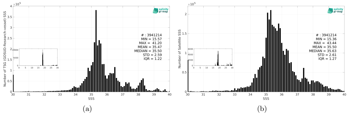
Figure 3: Histograms of SSS from TSG (GOSUD-Research-vessel) (a) and SMAP SSS L3 v6 - 8-Day running (RSS) (b) considering all match-up pairs per bins of 0.1 over the Global Ocean Pi-MEP region and for the full satellite product period.
