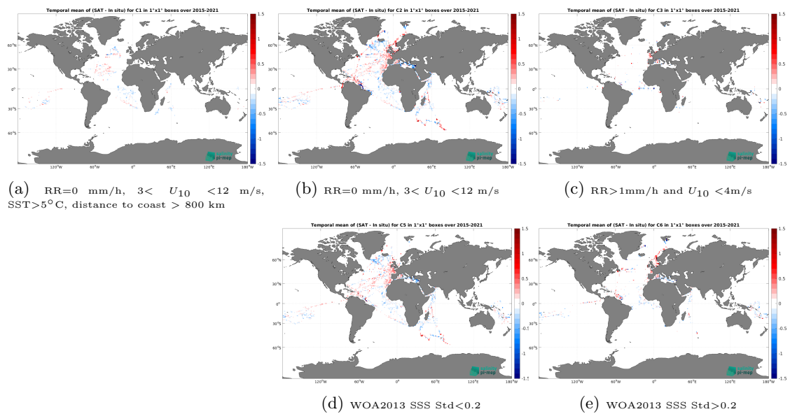
Figure 14: Temporal mean gridded over spatial boxes of size 1^\circ \times 1^\circ of \Delta SSS (SMAP SSS L3 v6 - 8-Day running (RSS) - TSG (GOSUD-Research-vessel)) for 5 different subdatasets corresponding to:RR=0 mm/h, 3 < U_{10} < 12 m/s, SST > 5^\circ\text{C} , distance to coast > 800 km (a), RR=0 mm/h, 3 < U_{10} < 12 m/s (b), RR > 1 mm/h and U_{10} < 4 m/s (c), WOA2013 SSS Std < 0.2 (d), WOA2013 SSS Std > 0.2 (e).
