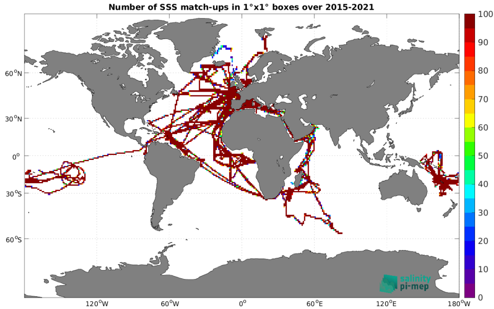
Figure 5: Number of SSS match-ups between TSG (GOSUD-Research-vessel) SSS and the SMAP SSS L3 v6 - 8-Day running (RSS) SSS product for the Global Ocean Pi-MEP region over 1^\circ \times 1^\circ boxes and for the full satellite product period.
