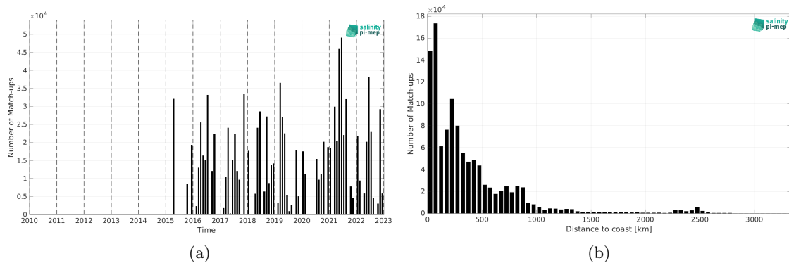
Figure 2: Number of match-ups between TSG (CSIC-UTM) and SMAP SSS L3 v6 - 8-Day running (RSS) SSS as a function of time (a) and as function of the distance to coast (b) over the Global Ocean Pi-MEP region and for the full satellite product period.
