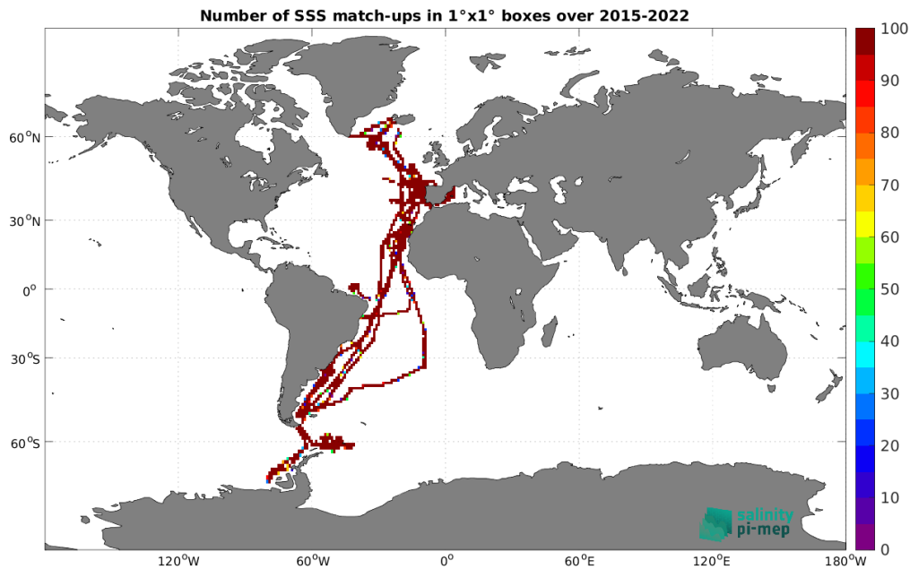
Figure 5: Number of SSS match-ups between TSG (CSIC-UTM) SSS and the SMAP SSS L3 v6 - 8-Day running (RSS) SSS product for the Global Ocean Pi-MEP region over 1°×1° boxes and for the full satellite product period.
