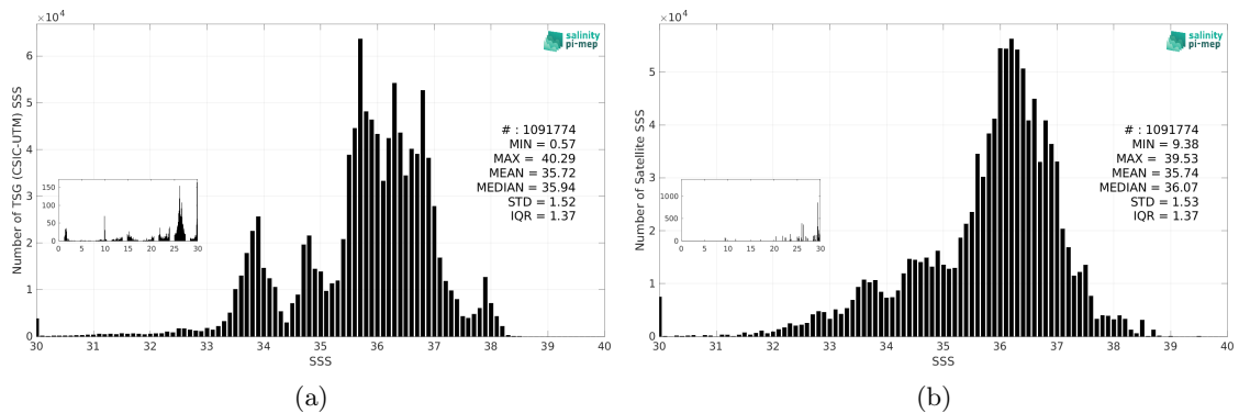
Figure 3: Histograms of SSS from TSG (CSIC-UTM) (a) and SMAP SSS L3 v6 - 8-Day running (RSS) (b) considering all match-up pairs per bins of 0.1 over the Global Ocean Pi-MEP region and for the full satellite product period.
