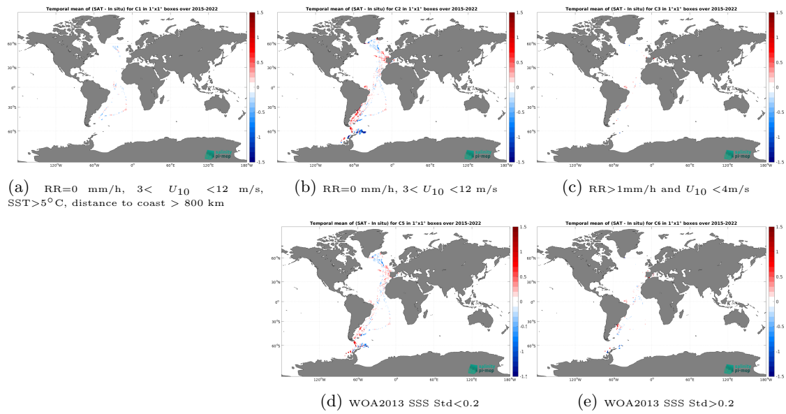
Figure 14: Temporal mean gridded over spatial boxes of size 1^\circ \times 1^\circ of \Delta SSS (SMAP SSS L3 v6 - 8-Day running (RSS) - TSG (CSIC-UTM)) for 5 different subdatasets corresponding to:RR=0 mm/h, 3 < U_{10} < 12 m/s, SST > 5^\circ\text{C} , distance to coast > 800 km (a), RR=0 mm/h, 3 < U_{10} < 12 m/s (b), RR > 1 mm/h and U_{10} < 4 m/s (c), WOA2013 SSS Std < 0.2 (d), WOA2013 SSS Std > 0.2 (e).
