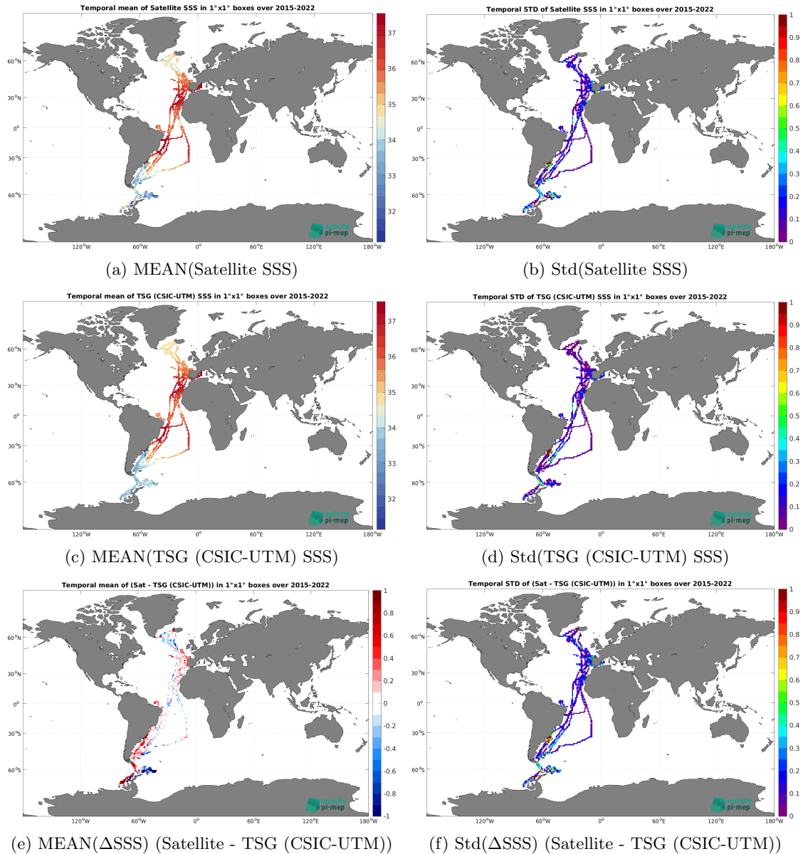
Figure 7: Temporal mean (left) and Std (right) of SSS from SMAP SSS L3 v6 - 8-Day running (RSS) (top), TSG (CSIC-UTM) (middle), and of \Delta SSS (Satellite - TSG (CSIC-UTM)). Only match-up pairs are used to generate these maps.
