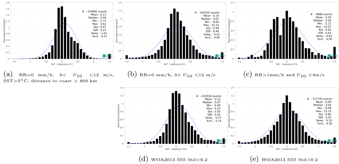
Figure 15: Normalized histogram of \Delta\text{SSS} (SMAP SSS L3 v6 - 8-Day running (RSS) - Sairdrone) for 5 different subdatasets corresponding to: RR=0 mm/h, 3 < U_{10} < 12 m/s, SST > 5^\circ\text{C} , distance to coast > 800 km (a), RR=0 mm/h, 3 < U_{10} < 12 m/s (b), RR > 1 mm/h and U_{10} < 4 m/s (c), WOA2013 SSS Std < 0.2 (d), WOA2013 SSS Std > 0.2 (e).
