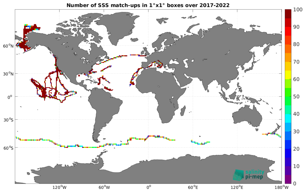
Figure 5: Number of SSS match-ups between Saildrone SSS and the SMAP SSS L3 v6 - 8-Day running (RSS) SSS product for the Global Ocean Pi-MEP region over 1^\circ \times 1^\circ boxes and for the full satellite product period.
