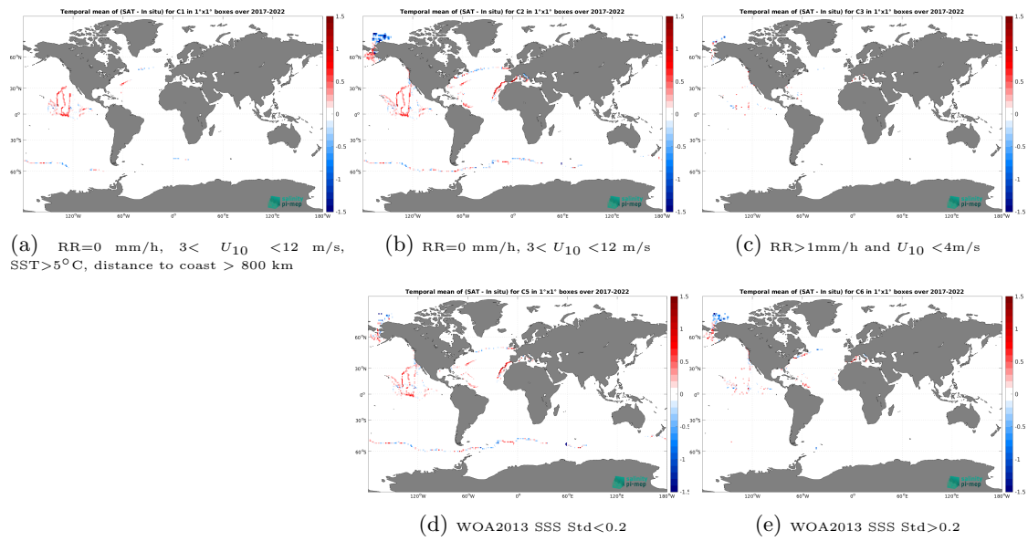
Figure 14: Temporal mean gridded over spatial boxes of size 1^\circ \times 1^\circ of \Delta SSS (SMAP SSS L3 v6 - 8-Day running (RSS) - Sairdrone) for 5 different subdatasets corresponding to:RR=0 mm/h, 3 < U_{10} < 12 m/s, SST > 5^\circ\text{C} , distance to coast > 800 km (a), RR=0 mm/h, 3 < U_{10} < 12 m/s (b), RR > 1 mm/h and U_{10} < 4 m/s (c), WOA2013 SSS Std < 0.2 (d), WOA2013 SSS Std > 0.2 (e).
