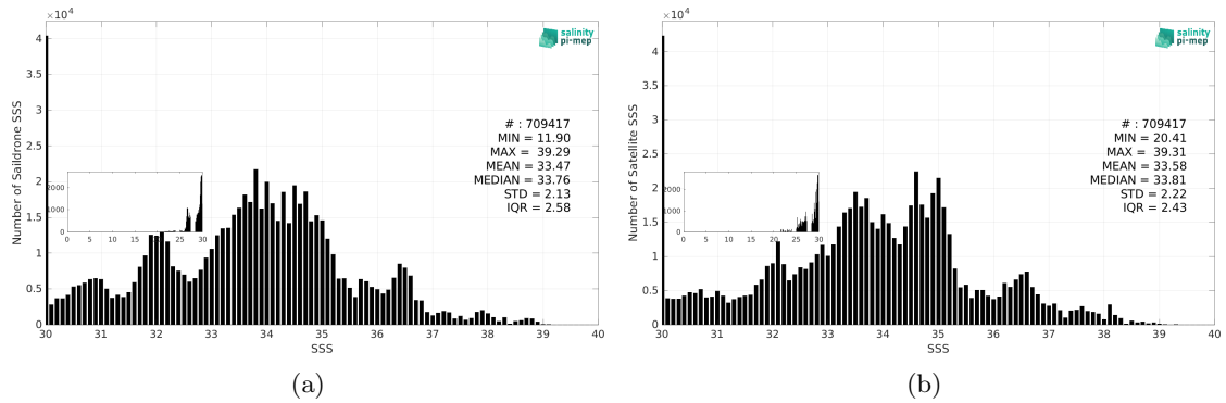
Figure 3: Histograms of SSS from Saildrone (a) and SMAP SSS L3 v6 - 8-Day running (RSS) (b) considering all match-up pairs per bins of 0.1 over the Global Ocean Pi-MEP region and for the full satellite product period.
