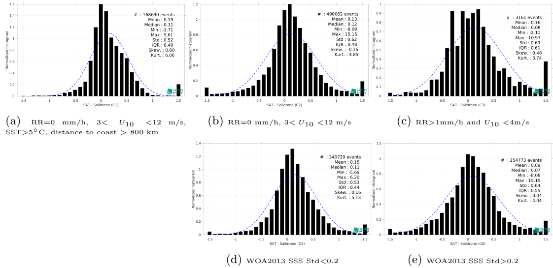
Figure 15: Normalized histogram of \Delta SSS (SMAP SSS L3 v6 - 8-Day running (RSS) - Sairdronne) for 5 different subdatasets corresponding to: RR=0 mm/h, 3 < U_{10} < 12 m/s, SST>5°C, distance to coast > 800 km (a), RR=0 mm/h, 3 < U_{10} < 12 m/s (b), RR>1mm/h and U_{10} < 4 m/s (c), WOA2013 SSS Std<0.2 (d), WOA2013 SSS Std>0.2 (e).
