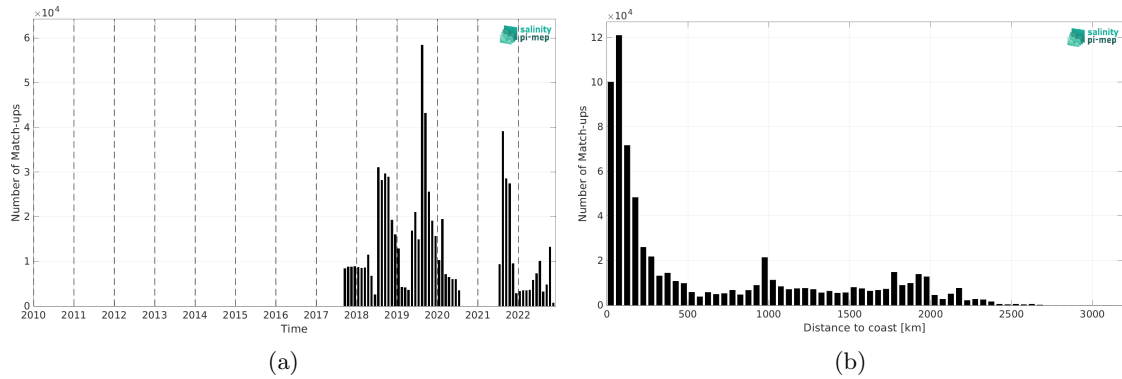
Figure 2: Number of match-ups between Saildrone and SMAP SSS L3 v6 - 8-Day running (RSS) SSS as a function of time (a) and as function of the distance to coast (b) over the Global Ocean Pi-MEP region and for the full satellite product period.
