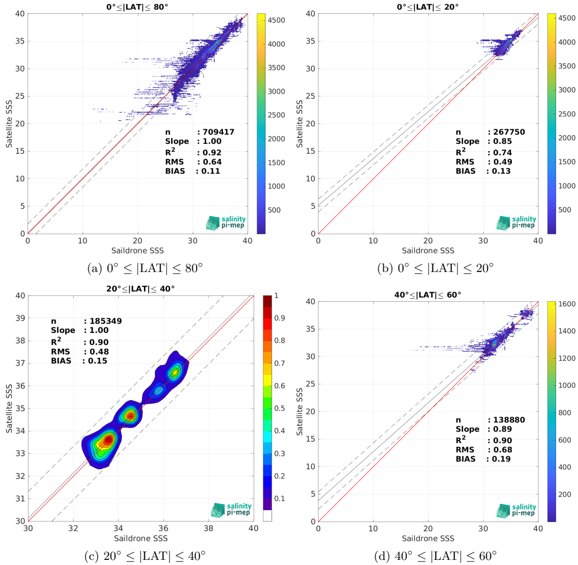
Figure 10: Contour maps of the concentration of SMAP SSS L3 v6 - 8-Day running (RSS) SSS (y-axis) versus Saildrone SSS (x-axis) at match-up pairs for different latitude bands. For each plot, the red line shows x=y . The black thin and dashed lines indicate a linear fit through the data cloud and the \pm 95\% confidence levels, respectively. The number match-up pairs n , the slope and R^2 coefficient of the linear fit, the root mean square (RMS) and the mean bias between satellite and in situ data are indicated for each latitude band in each plots.
