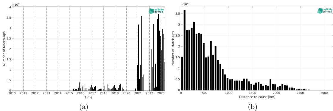
Figure 2: Number of match-ups between TSG (Polarstern) and SMAP SSS L3 v6 - Monthly (RSS) SSS as a function of time (a) and as function of the distance to coast (b) over the Global Ocean Pi-MEP region and for the full satellite product period.
