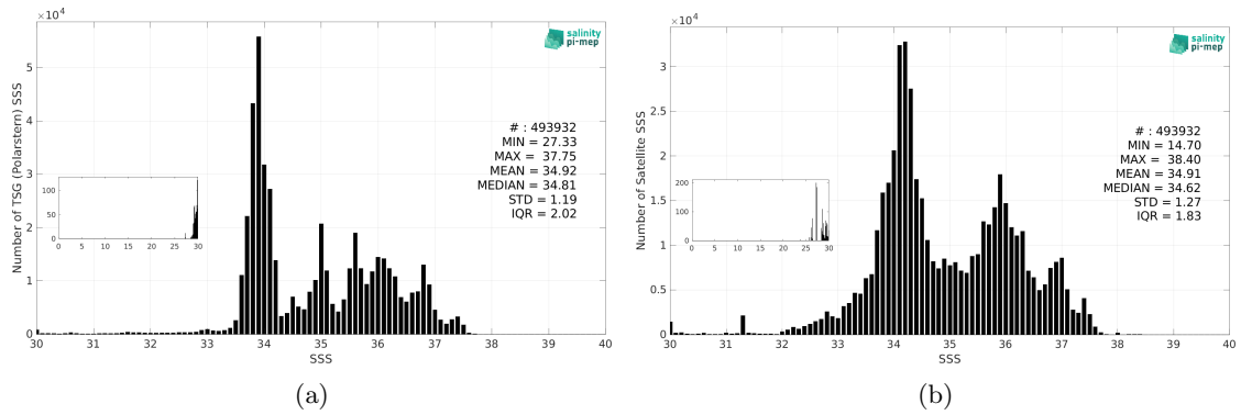
Figure 3: Histograms of SSS from TSG (Polarstern) (a) and SMAP SSS L3 v6 - Monthly (RSS) (b) considering all match-up pairs per bins of 0.1 over the Global Ocean Pi-MEP region and for the full satellite product period.
