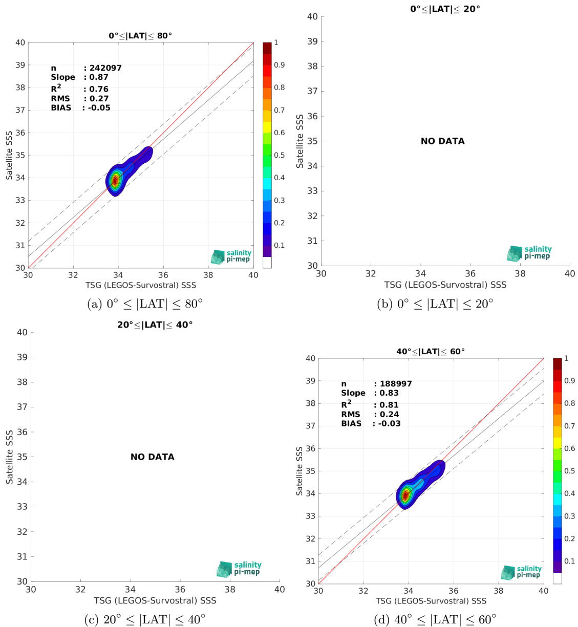
Figure 10: Contour maps of the concentration of SMAP SSS L3 v6 - Monthly (RSS) SSS (y-axis) versus TSG (LEGOS-Survostral) SSS (x-axis) at match-up pairs for different latitude bands. For each plot, the red line shows x=y . The black thin and dashed lines indicate a linear fit through the data cloud and the \pm 95\% confidence levels, respectively. The number match-up pairs n , the slope and R^2 coefficient of the linear fit, the root mean square (RMS) and the mean bias between satellite and in situ data are indicated for each latitude band in each plots.
