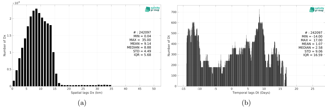
Figure 6: Histograms of the spatial (a) and temporal (b) lags between the location/time of the TSG (LEGOS-Survostral) measurement and the date of the corresponding SMAP SSS L3 v6 - Monthly (RSS) SSS pixel.
