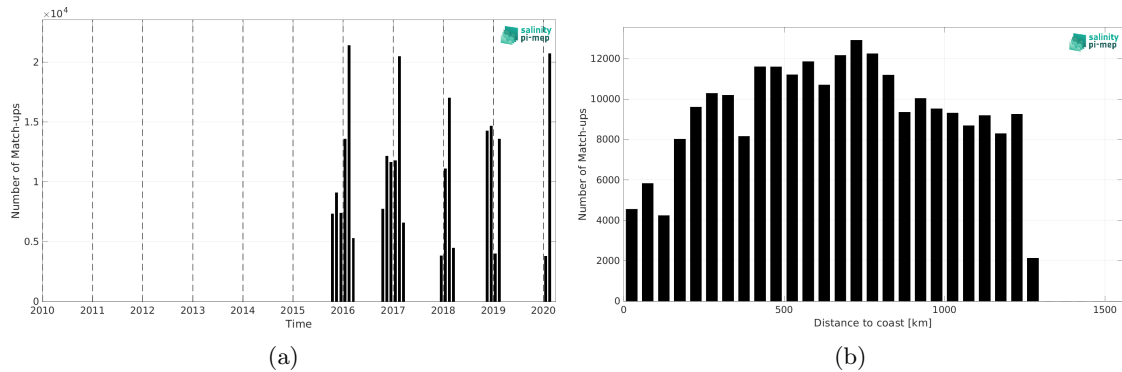
Figure 2: Number of match-ups between TSG (LEGOS-Survostral) and SMAP SSS L3 v6 - Monthly (RSS) SSS as a function of time (a) and as function of the distance to coast (b) over the Global Ocean Pi-MEP region and for the full satellite product period.
