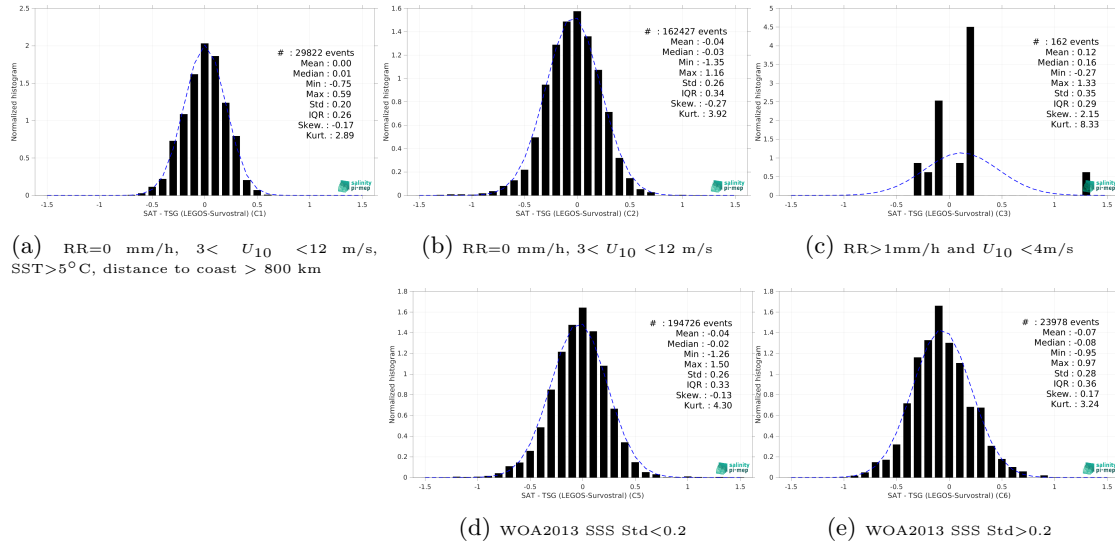
Figure 15: Normalized histogram of \Delta SSS (SMAP SSS L3 v6 - Monthly (RSS) - TSG (LEGOS-Survostral)) for 5 different subdatasets corresponding to: RR=0 mm/h, 3 < U_{10} < 12 m/s, SST > 5°C, distance to coast > 800 km (a), RR=0 mm/h, 3 < U_{10} < 12 m/s (b), RR > 1mm/h and U_{10} < 4 m/s (c), WOA2013 SSS Std < 0.2 (d), WOA2013 SSS Std > 0.2 (e).
