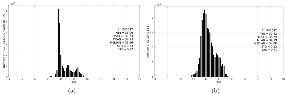
Figure 3: Histograms of SSS from TSG (LEGOS-Survostral) (a) and SMAP SSS L3 v6 - Monthly (RSS) (b) considering all match-up pairs per bins of 0.1 over the Global Ocean Pi-MEP region and for the full satellite product period.
