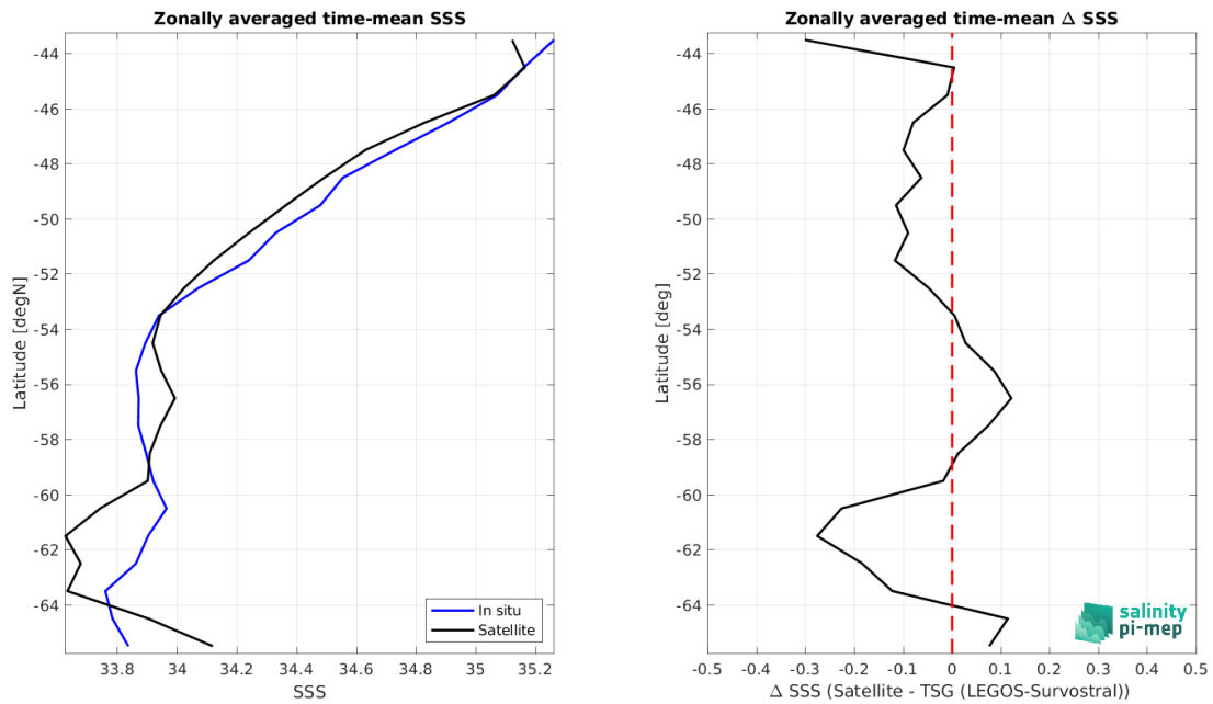
Figure 9: Left panel: Zonal mean SSS from SMAP SSS L3 v6 - Monthly (RSS) satellite product (black) and from TSG (LEGOS-Survostral) (blue). Right panel: Zonal mean of \Delta SSS (Satellite - TSG (LEGOS-Survostral)) for all the collected Pi-MEP match-up pairs estimated over the full satellite product period.
