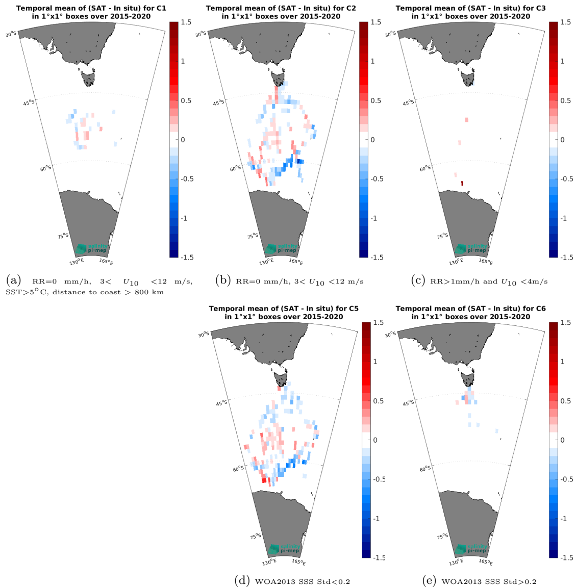
Figure 14: Temporal mean gridded over spatial boxes of size 1^\circ \times 1^\circ of \Delta\text{SSS} (SMAP SSS L3 v6 - Monthly (RSS) - TSG (LEGOS-Survostral)) for 5 different subdatasets corresponding to: RR=0 mm/h, 3 < U_{10} < 12 m/s, SST > 5^\circ\text{C} , distance to coast > 800 km (a), RR=0 mm/h, 3 < U_{10} < 12 m/s (b), RR > 1 mm/h and U_{10} < 4 m/s (c), WOA2013 SSS Std < 0.2 (d), WOA2013 SSS Std > 0.2 (e).
