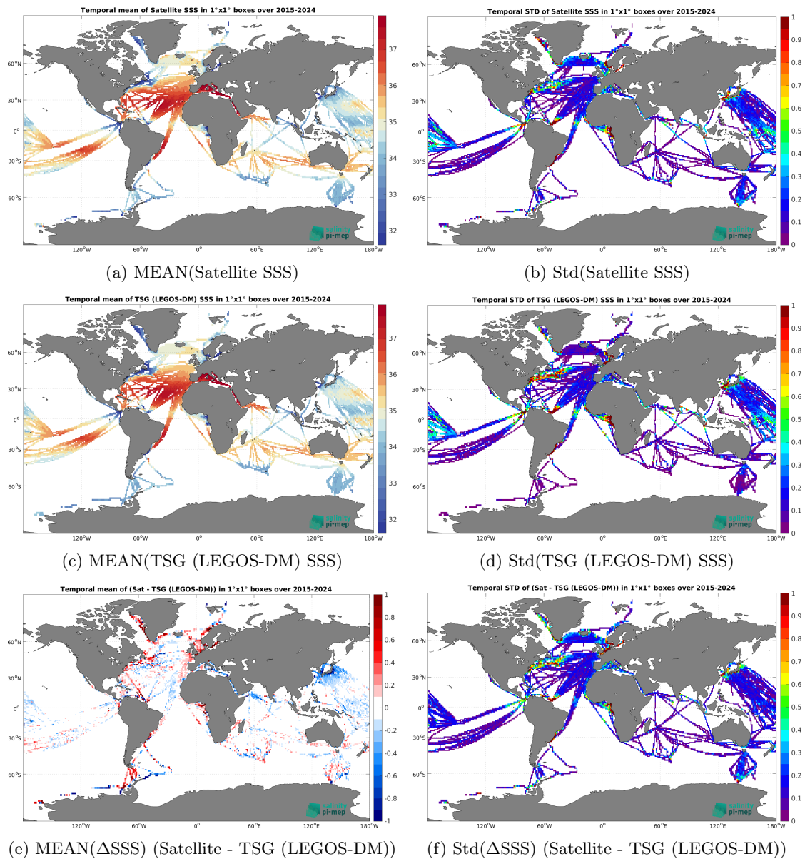
Figure 7: Temporal mean (left) and Std (right) of SSS from SMAP SSS L3 v6 - Monthly (RSS) (top), TSG (LEGOS-DM) (middle), and of \Delta SSS (Satellite - TSG (LEGOS-DM)). Only match-pairs are used to generate these maps.
