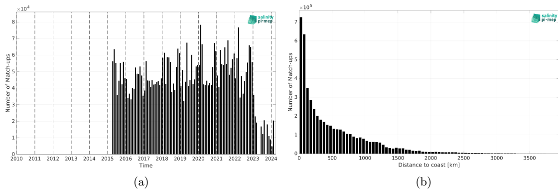
Figure 2: Number of match-ups between TSG (LEGOS-DM) and SMAP SSS L3 v6 - Monthly (RSS) SSS as a function of time (a) and as function of the distance to coast (b) over the Global Ocean Pi-MEP region and for the full satellite product period.
