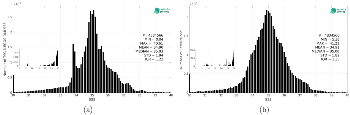
Figure 3: Histograms of SSS from TSG (LEGOS-DM) (a) and SMAP SSS L3 v6 - Monthly (RSS) (b) considering all match-up pairs per bins of 0.1 over the Global Ocean Pi-MEP region and for the full satellite product period.
