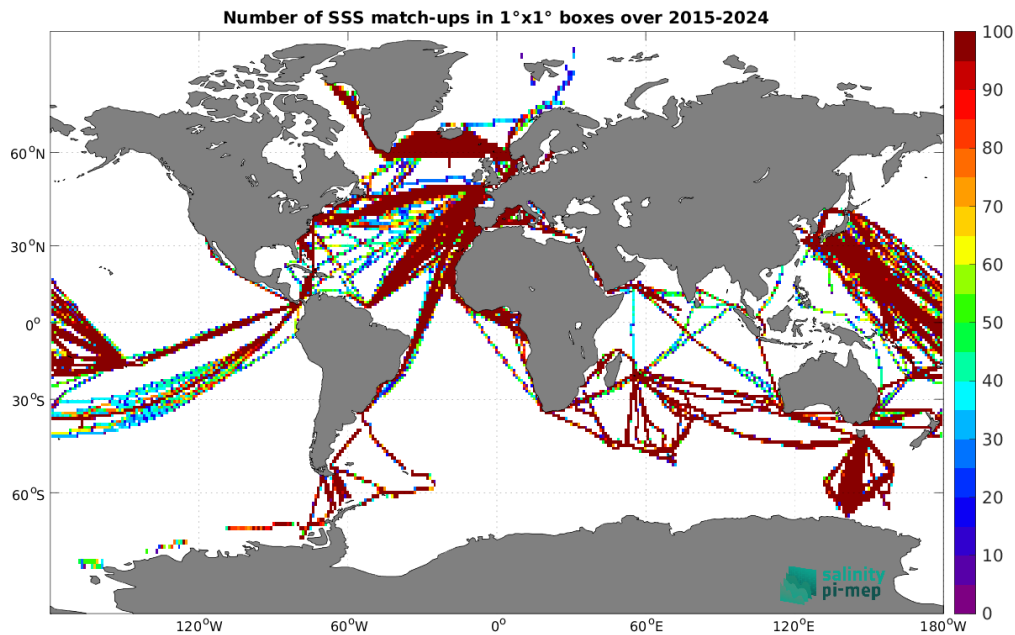
Figure 5: Number of SSS match-ups between TSG (LEGOS-DM) SSS and the SMAP SSS L3 v6 - Monthly (RSS) SSS product for the Global Ocean Pi-MEP region over 1^\circ \times 1^\circ boxes and for the full satellite product period.
