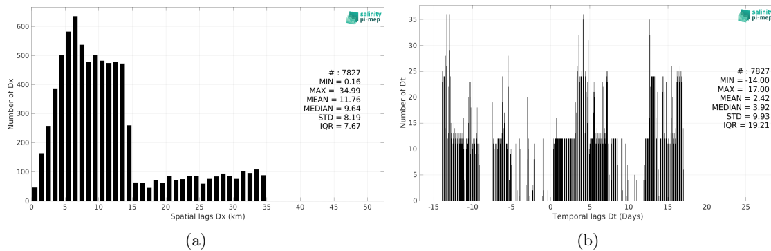
Figure 6: Histograms of the spatial (a) and temporal (b) lags between the location/time of the TSG (Lauge-Koch) measurement and the date of the corresponding SMAP SSS L3 v6 - Monthly (RSS) SSS pixel.
