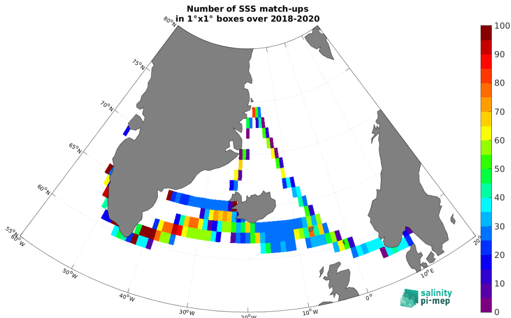
Figure 5: Number of SSS match-ups between TSG (Lauge-Koch) SSS and the SMAP SSS L3 v6 - Monthly (RSS) SSS product for the Global Ocean Pi-MEP region over 1^\circ \times 1^\circ boxes and for the full satellite product period.
