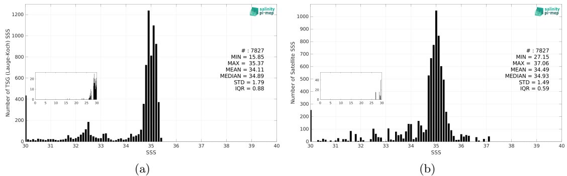
Figure 3: Histograms of SSS from TSG (Lauge-Koch) (a) and SMAP SSS L3 v6 - Monthly (RSS) (b) considering all match-up pairs per bins of 0.1 over the Global Ocean Pi-MEP region and for the full satellite product period.
