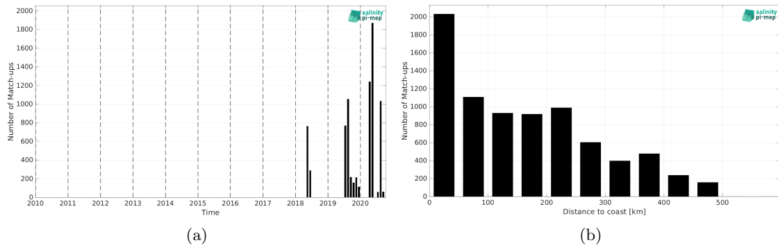
Figure 2: Number of match-ups between TSG (Lauge-Koch) and SMAP SSS L3 v6 - Monthly (RSS) SSS as a function of time (a) and as function of the distance to coast (b) over the Global Ocean Pi-MEP region and for the full satellite product period.
