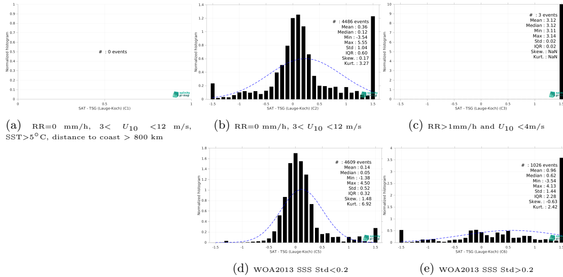
Figure 15: Normalized histogram of \Delta SSS (SMAP SSS L3 v6 - Monthly (RSS) - TSG (Lauge-Koch)) for 5 different subdatasets corresponding to: RR=0 mm/h, 3 < U_{10} < 12 m/s, SST>5°C, distance to coast > 800 km (a), RR=0 mm/h, 3 < U_{10} < 12 m/s (b), RR>1mm/h and U_{10} < 4 m/s (c), WOA2013 SSS Std<0.2 (d), WOA2013 SSS Std>0.2 (e).
