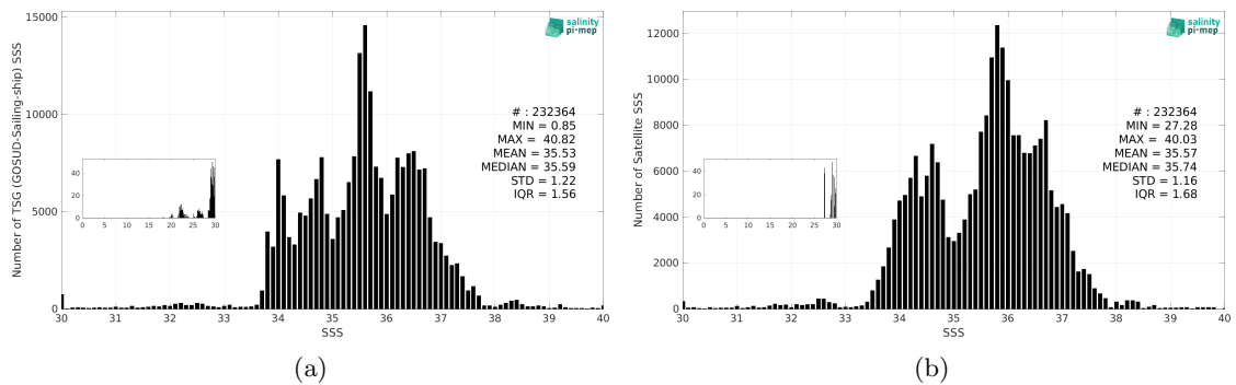
Figure 3: Histograms of SSS from TSG (GOSUD-Sailing-ship) (a) and SMAP SSS L3 v6 - Monthly (RSS) (b) considering all match-up pairs per bins of 0.1 over the Global Ocean Pi-MEP region and for the full satellite product period.
