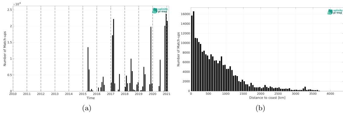
Figure 2: Number of match-ups between TSG (GOSUD-Sailing-ship) and SMAP SSS L3 v6 - Monthly (RSS) SSS as a function of time (a) and as function of the distance to coast (b) over the Global Ocean Pi-MEP region and for the full satellite product period.
