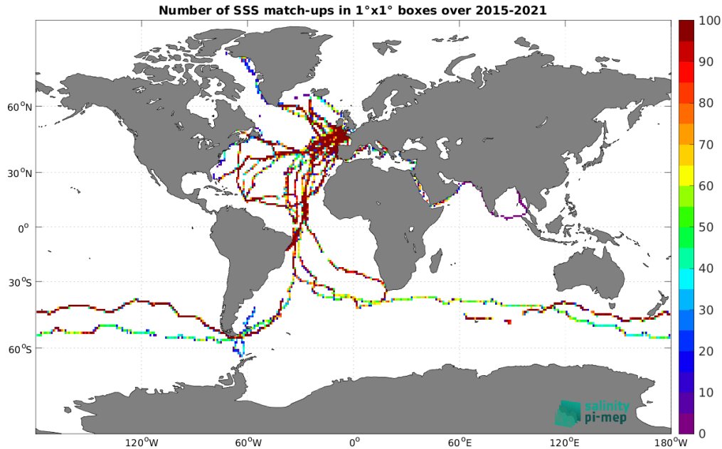
Figure 5: Number of SSS match-ups between TSG (GOSUD-Sailing-ship) SSS and the SMAP SSS L3 v6 - Monthly (RSS) SSS product for the Global Ocean Pi-MEP region over 1°x1° boxes and for the full satellite product period.
