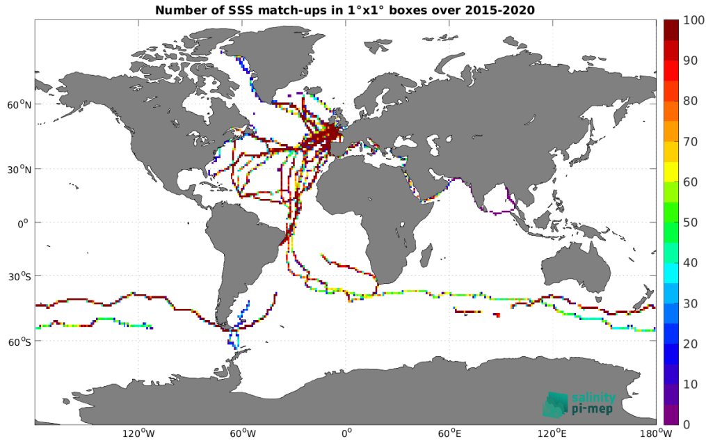
Figure 5: Number of SSS match-ups between TSG (GOSUD-Sailing-ship) SSS and the SMAP SSS L3 v6 - Monthly (RSS) SSS product for the Global Ocean Pi-MEP region over 1°×1° boxes and for the full satellite product period.
