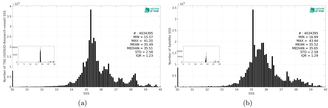
Figure 3: Histograms of SSS from TSG (GOSUD-Research-vessel) (a) and SMAP SSS L3 v6 - Monthly (RSS) (b) considering all match-up pairs per bins of 0.1 over the Global Ocean Pi-MEP region and for the full satellite product period.
