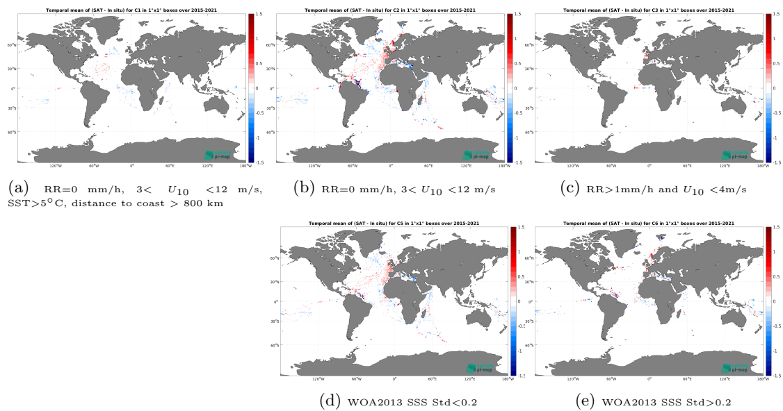
Figure 14: Temporal mean gridded over spatial boxes of size 1^\circ \times 1^\circ of \Delta SSS (SMAP SSS L3 v6 - Monthly (RSS) - TSG (GOSUD-Research-vessel)) for 5 different subdatasets corresponding to:RR=0 mm/h, 3 < U_{10} < 12 m/s, SST > 5^\circ\text{C} , distance to coast > 800 km (a), RR=0 mm/h, 3 < U_{10} < 12 m/s (b), RR > 1 mm/h and U_{10} < 4 m/s (c), WOA2013 SSS Std < 0.2 (d), WOA2013 SSS Std > 0.2 (e).
