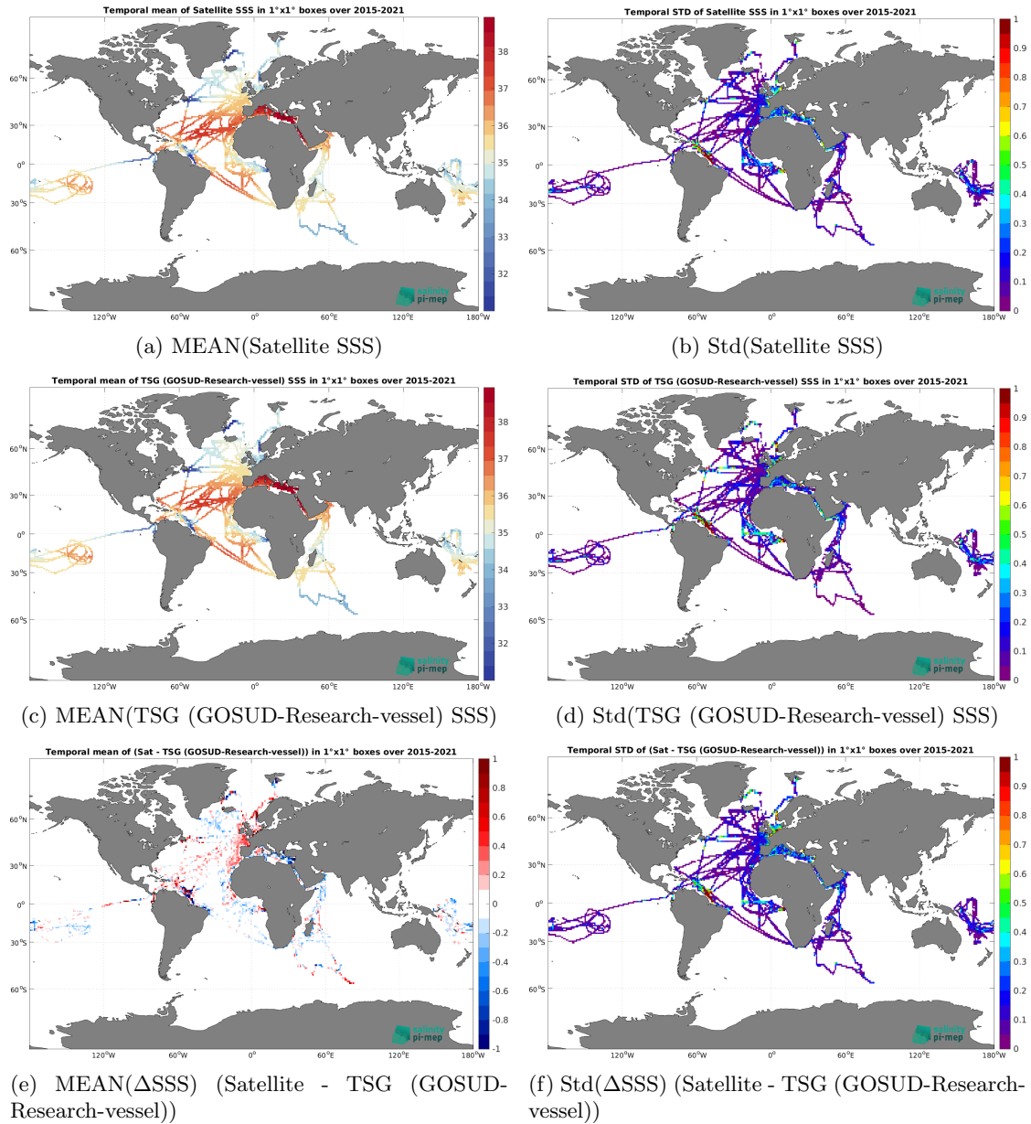
Figure 7: Temporal mean (left) and Std (right) of SSS from SMAP SSS L3 v6 - Monthly (RSS) (top), TSG (GOSUD-Research-vessel) (middle), and of \Delta SSS (Satellite - TSG (GOSUD-Research-vessel)). Only match-up pairs are used to generate these maps.
