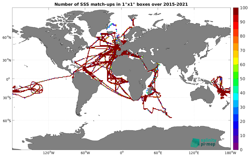
Figure 5: Number of SSS match-ups between TSG (GOSUD-Research-vessel) SSS and the SMAP SSS L3 v6 - Monthly (RSS) SSS product for the Global Ocean Pi-MEP region over 1^\circ \times 1^\circ boxes and for the full satellite product period.
