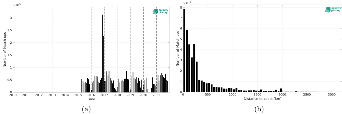
Figure 2: Number of match-ups between TSG (GOSUD-Research-vessel) and SMAP SSS L3 v6 - Monthly (RSS) SSS as a function of time (a) and as function of the distance to coast (b) over the Global Ocean Pi-MEP region and for the full satellite product period.
