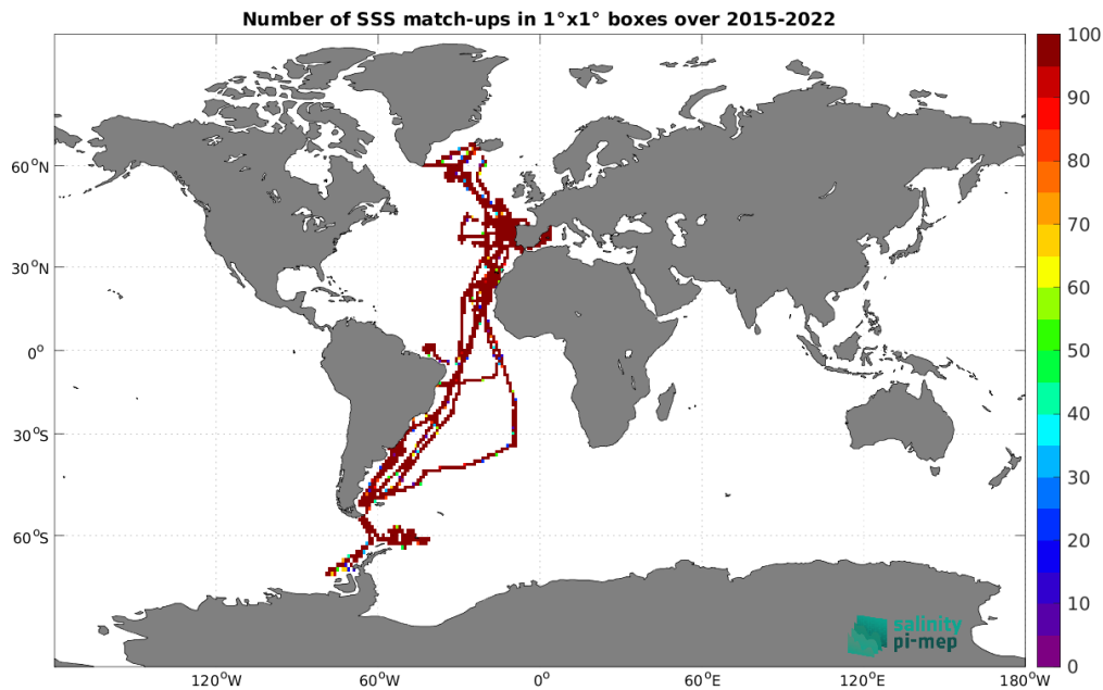
Figure 5: Number of SSS match-ups between TSG (CSIC-UTM) SSS and the SMAP SSS L3 v6 - Monthly (RSS) SSS product for the Global Ocean Pi-MEP region over 1°x1° boxes and for the full satellite product period.
