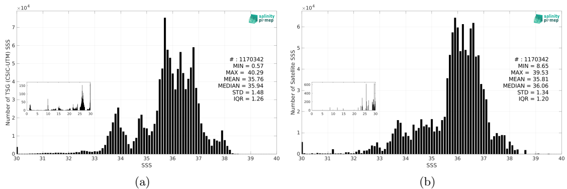
Figure 3: Histograms of SSS from TSG (CSIC-UTM) (a) and SMAP SSS L3 v6 - Monthly (RSS) (b) considering all match-up pairs per bins of 0.1 over the Global Ocean Pi-MEP region and for the full satellite product period.
