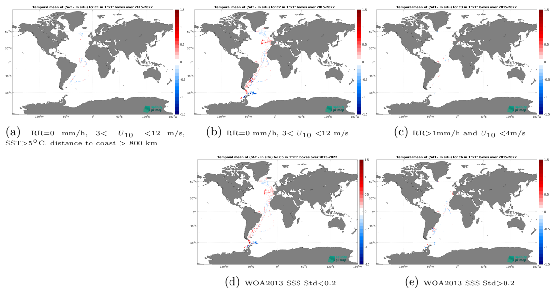
Figure 14: Temporal mean gridded over spatial boxes of size 1^\circ \times 1^\circ of \Delta SSS (SMAP SSS L3 v6 - Monthly (RSS) - TSG (CSIC-UTM)) for 5 different subdatasets corresponding to:RR=0 mm/h, 3 < U_{10} < 12 m/s, SST > 5^\circ\text{C} , distance to coast > 800 km (a), RR=0 mm/h, 3 < U_{10} < 12 m/s (b), RR > 1 mm/h and U_{10} < 4 m/s (c), WOA2013 SSS Std < 0.2 (d), WOA2013 SSS Std > 0.2 (e).
