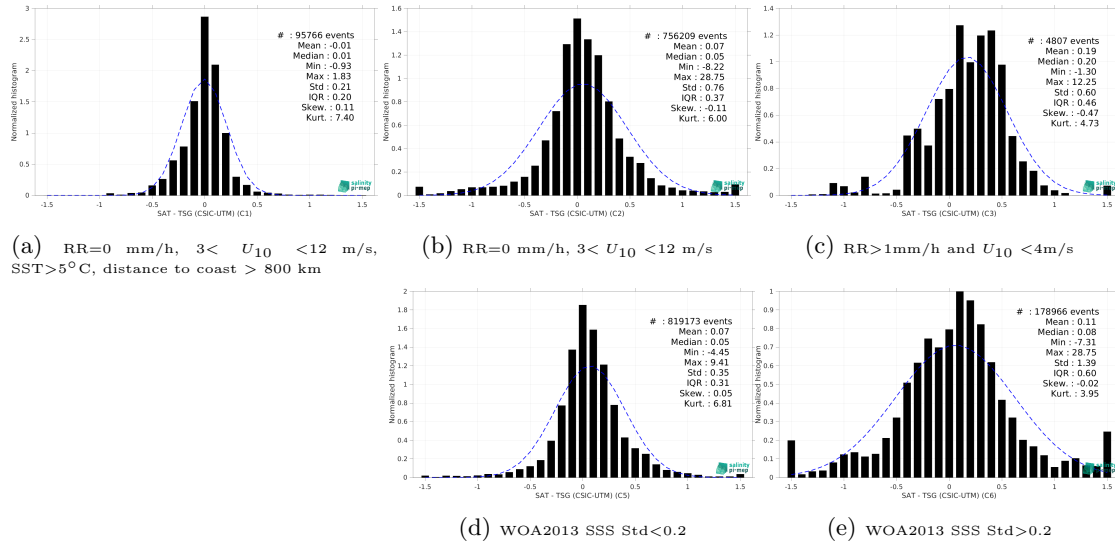
Figure 15: Normalized histogram of \Delta\text{SSS} (SMAP SSS L3 v6 - Monthly (RSS) - TSG (CSIC-UTM)) for 5 different subdatasets corresponding to: RR=0 mm/h, 3 < U_{10} < 12 m/s, SST > 5^\circ\text{C} , distance to coast > 800 km (a), RR=0 mm/h, 3 < U_{10} < 12 m/s (b), RR > 1 mm/h and U_{10} < 4 m/s (c), WOA2013 SSS Std < 0.2 (d), WOA2013 SSS Std > 0.2 (e).
