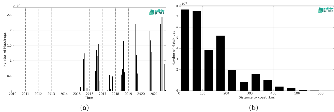
Figure 2: Number of match-ups between TSG (Amundsen) and SMAP SSS L3 v6 - Monthly (RSS) SSS as a function of time (a) and as function of the distance to coast (b) over the Global Ocean Pi-MEP region and for the full satellite product period.
