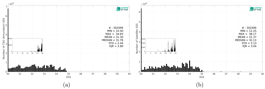
Figure 3: Histograms of SSS from TSG (Amundsen) (a) and SMAP SSS L3 v6 - Monthly (RSS) (b) considering all match-up pairs per bins of 0.1 over the Global Ocean Pi-MEP region and for the full satellite product period.
