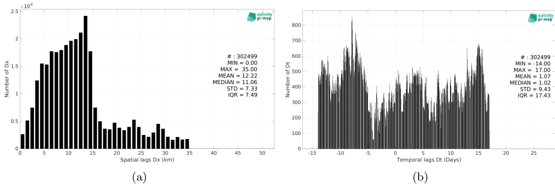
Figure 6: Histograms of the spatial (a) and temporal (b) lags between the location/time of the TSG (Amundsen) measurement and the date of the corresponding SMAP SSS L3 v6 - Monthly (RSS) SSS pixel.
