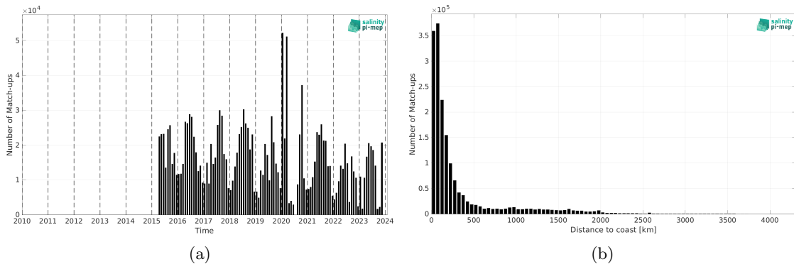
Figure 2: Number of match-ups between TSG (SAMOS) and SMAP SSS L3 v5.3 - 8-Day running (RSS) SSS as a function of time (a) and as function of the distance to coast (b) over the Global Ocean Pi-MEP region and for the full satellite product period.
