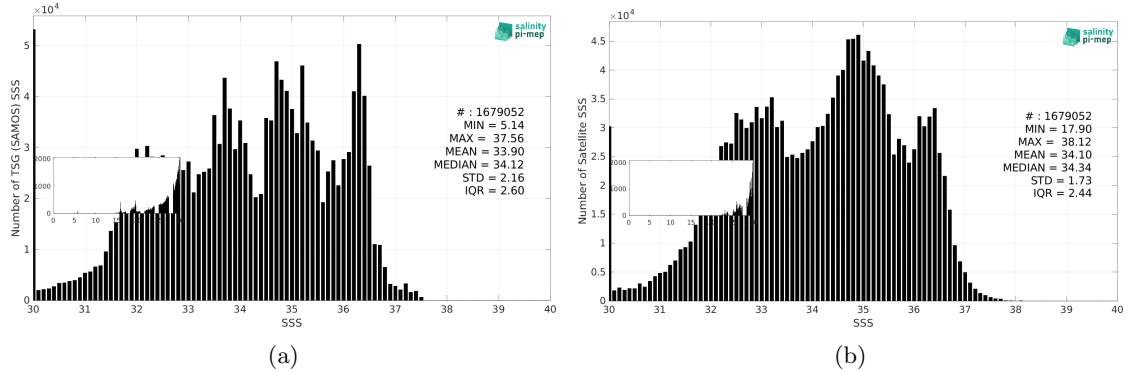
Figure 3: Histograms of SSS from TSG (SAMOS) (a) and SMAP SSS L3 v5.3 - 8-Day running (RSS) (b) considering all match-up pairs per bins of 0.1 over the Global Ocean Pi-MEP region and for the full satellite product period.
