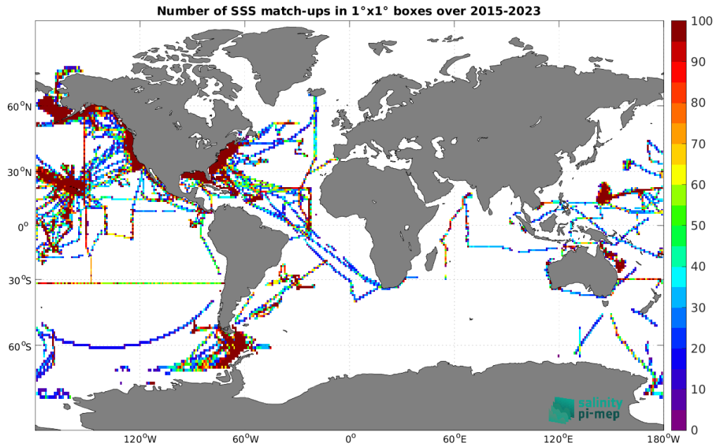
Figure 5: Number of SSS match-ups between TSG (SAMOS) SSS and the SMAP SSS L3 v5.3 - 8-Day running (RSS) SSS product for the Global Ocean Pi-MEP region over 1^\circ \times 1^\circ boxes and for the full satellite product period.
