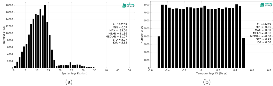
Figure 6: Histograms of the spatial (a) and temporal (b) lags between the location/time of the TSG (NCEI-0170743) measurement and the date of the corresponding SMAP SSS L3 v5.3 - 8-Day running (RSS) SSS pixel.
