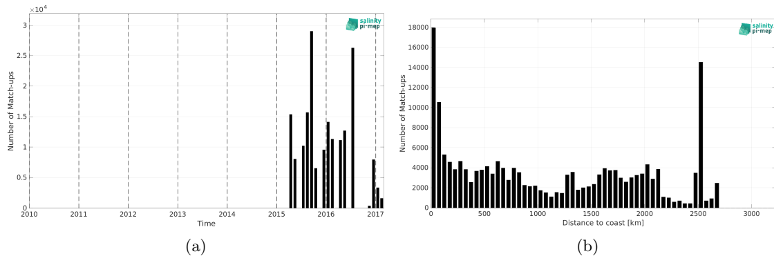
Figure 2: Number of match-ups between TSG (NCEI-0170743) and SMAP SSS L3 v5.3 - 8-Day running (RSS) SSS as a function of time (a) and as function of the distance to coast (b) over the Global Ocean Pi-MEP region and for the full satellite product period.
