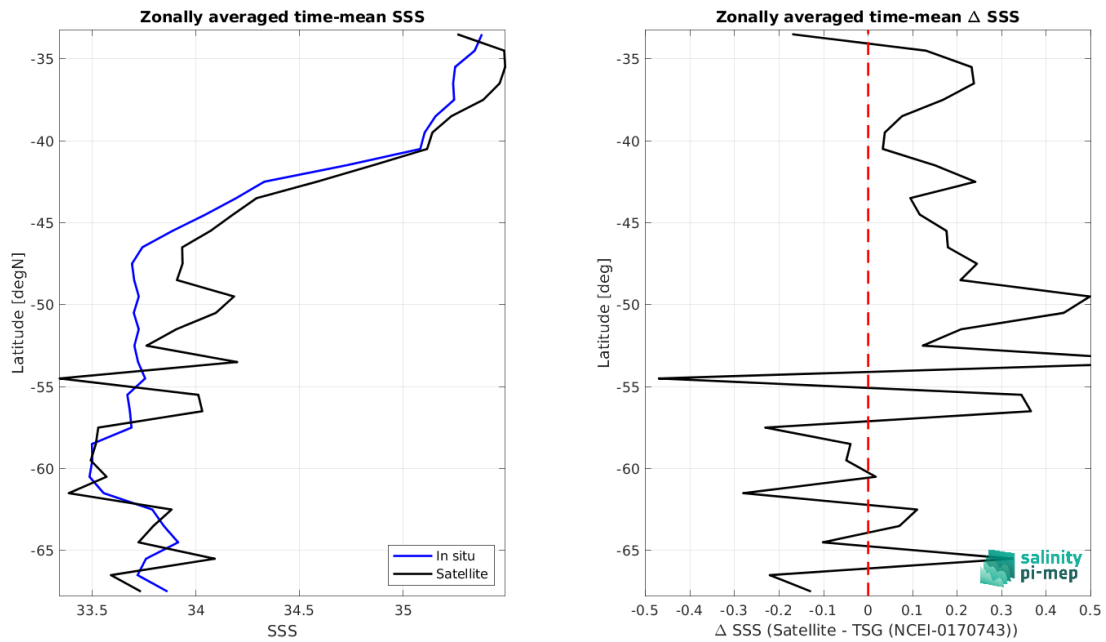
Figure 9: Left panel: Zonal mean SSS from SMAP SSS L3 v5.3 - 8-Day running (RSS) satellite product (black) and from TSG (NCEI-0170743) (blue). Right panel: Zonal mean of \Delta SSS (Satellite - TSG (NCEI-0170743)) for all the collected Pi-MEP match-up pairs estimated over the full satellite product period.
