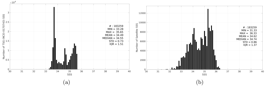
Figure 3: Histograms of SSS from TSG (NCEI-0170743) (a) and SMAP SSS L3 v5.3 - 8-Day running (RSS) (b) considering all match-up pairs per bins of 0.1 over the Global Ocean Pi-MEP region and for the full satellite product period.
