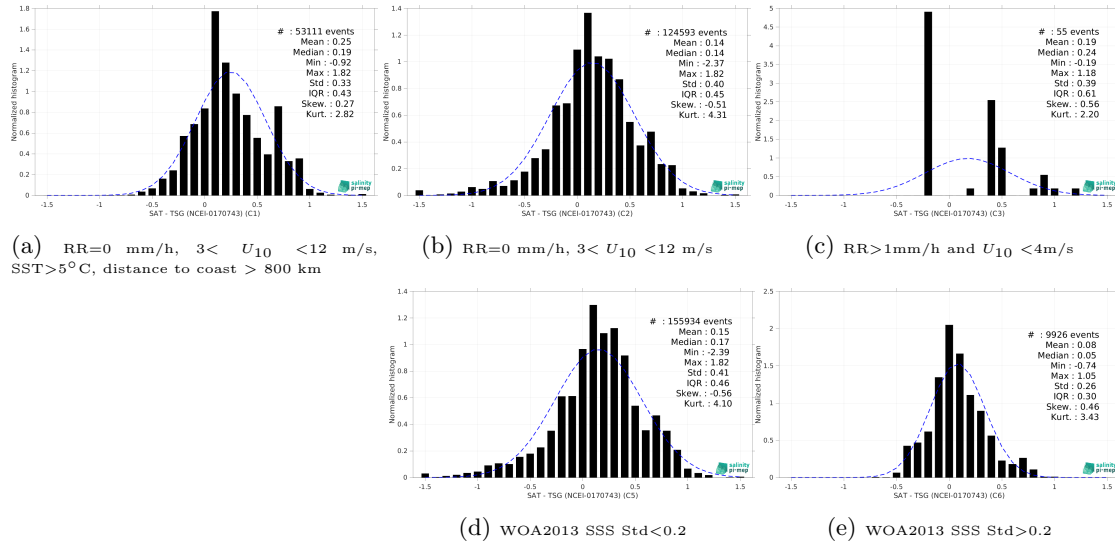
Figure 15: Normalized histogram of \Delta SSS (SMAP SSS L3 v5.3 - 8-Day running (RSS) - TSG (NCEI-0170743)) for 5 different subdatasets corresponding to: RR=0 mm/h, 3 < U_{10} < 12 m/s, SST > 5°C, distance to coast > 800 km (a), RR=0 mm/h, 3 < U_{10} < 12 m/s (b), RR > 1mm/h and U_{10} < 4 m/s (c), WOA2013 SSS Std < 0.2 (d), WOA2013 SSS Std > 0.2 (e).
