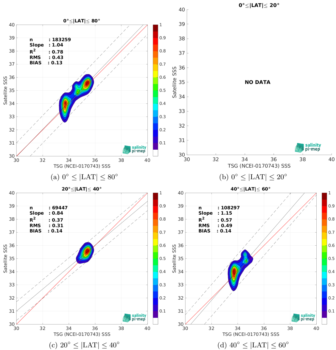
Figure 10: Contour maps of the concentration of SMAP SSS L3 v5.3 - 8-Day running (RSS) SSS (y-axis) versus TSG (NCEI-0170743) SSS (x-axis) at match-up pairs for different latitude bands. For each plot, the red line shows x=y . The black thin and dashed lines indicate a linear fit through the data cloud and the \pm 95\% confidence levels, respectively. The number match-up pairs n , the slope and R^2 coefficient of the linear fit, the root mean square (RMS) and the mean bias between satellite and in situ data are indicated for each latitude band in each plots.
