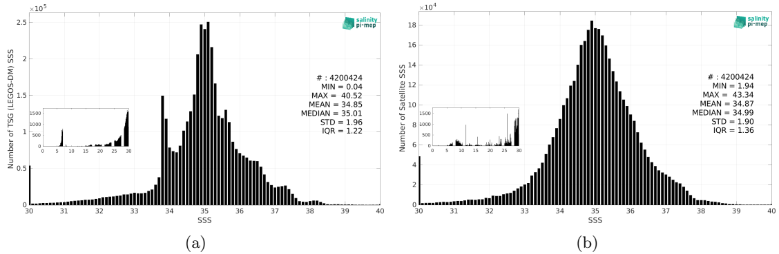
Figure 3: Histograms of SSS from TSG (LEGOS-DM) (a) and SMAP SSS L3 v5.3 - 8-Day running (RSS) (b) considering all match-up pairs per bins of 0.1 over the Global Ocean Pi-MEP region and for the full satellite product period.
