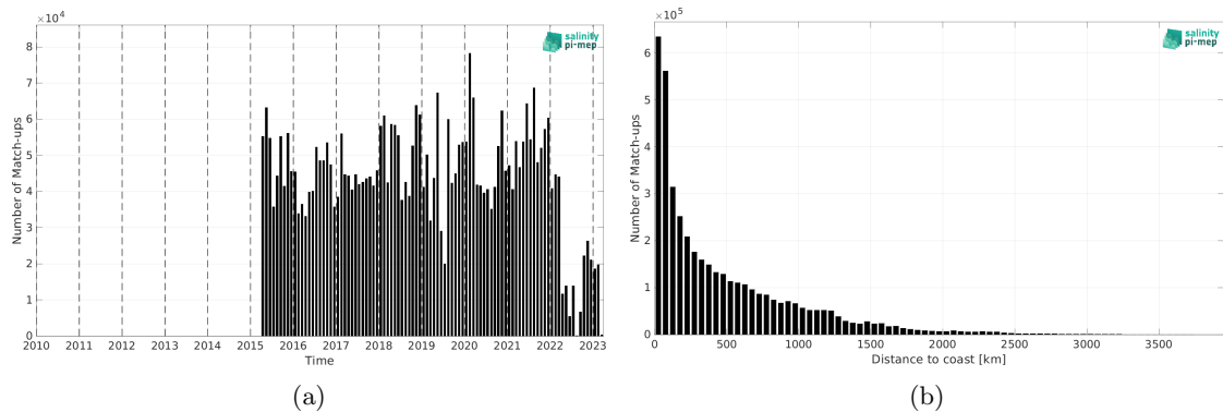
Figure 2: Number of match-ups between TSG (LEGOS-DM) and SMAP SSS L3 v5.3 - 8-Day running (RSS) SSS as a function of time (a) and as function of the distance to coast (b) over the Global Ocean Pi-MEP region and for the full satellite product period.
