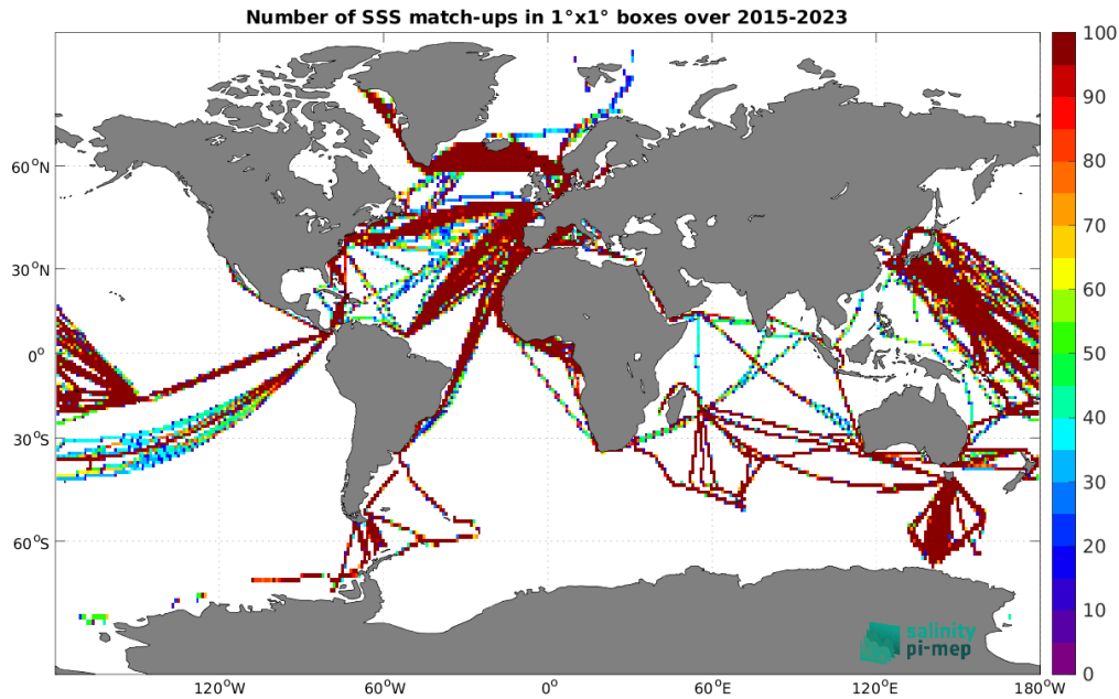
Figure 5: Number of SSS match-ups between TSG (LEGOS-DM) SSS and the SMAP SSS L3 v5.3 - 8-Day running (RSS) SSS product for the Global Ocean Pi-MEP region over 1^\circ \times 1^\circ boxes and for the full satellite product period.
