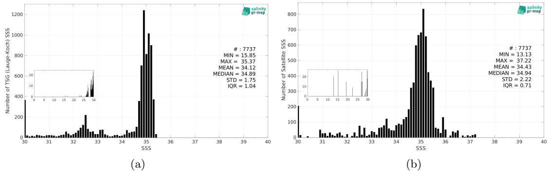
Figure 3: Histograms of SSS from TSG (Lauge-Koch) (a) and SMAP SSS L3 v5.3 - 8-Day running (RSS) (b) considering all match-up pairs per bins of 0.1 over the Global Ocean Pi-MEP region and for the full satellite product period.
