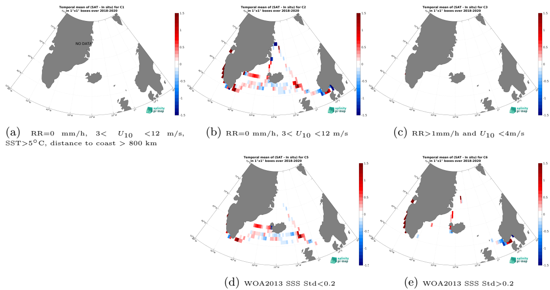
Figure 14: Temporal mean gridded over spatial boxes of size 1^\circ \times 1^\circ of \Delta SSS (SMAP SSS L3 v5.3 - 8-Day running (RSS) - TSG (Lauge-Koch)) for 5 different subdatasets corresponding to:RR=0 mm/h, 3 < U_{10} < 12 m/s, SST > 5^\circ\text{C} , distance to coast > 800 km (a), RR=0 mm/h, 3 < U_{10} < 12 m/s (b), RR > 1 mm/h and U_{10} < 4 m/s (c), WOA2013 SSS Std < 0.2 (d), WOA2013 SSS Std > 0.2 (e).
