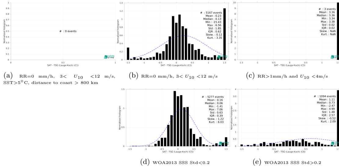
Figure 15: Normalized histogram of \Delta SSS (SMAP SSS L3 v5.3 - 8-Day running (RSS) - TSG (Lauge-Koch)) for 5 different subdatasets corresponding to: RR=0 mm/h, 3 < U_{10} < 12 m/s, SST > 5°C, distance to coast > 800 km (a), RR=0 mm/h, 3 < U_{10} < 12 m/s (b), RR > 1mm/h and U_{10} < 4 m/s (c), WOA2013 SSS Std < 0.2 (d), WOA2013 SSS Std > 0.2 (e).
