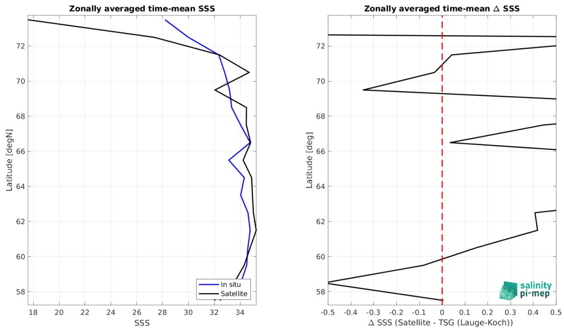
Figure 9: Left panel: Zonal mean SSS from SMAP SSS L3 v5.3 - 8-Day running (RSS) satellite product (black) and from TSG (Lauge-Koch) (blue). Right panel: Zonal mean of \Delta SSS (Satellite - TSG (Lauge-Koch)) for all the collected Pi-MEP match-up pairs estimated over the full satellite product period.
