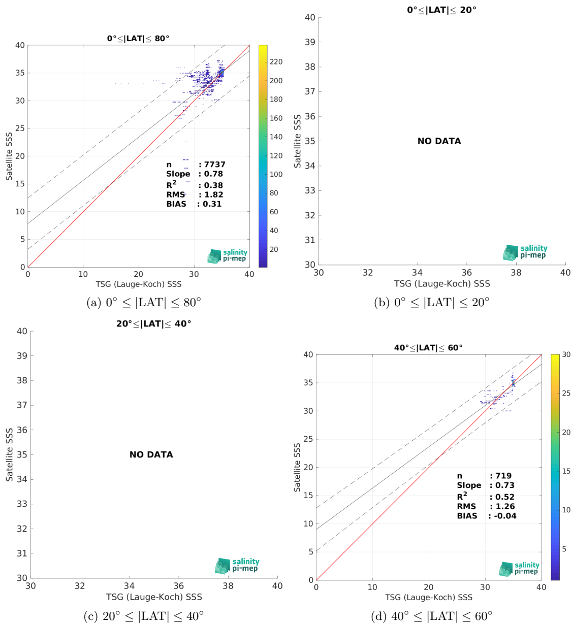
Figure 10: Contour maps of the concentration of SMAP SSS L3 v5.3 - 8-Day running (RSS) SSS (y-axis) versus TSG (Lauge-Koch) SSS (x-axis) at match-up pairs for different latitude bands. For each plot, the red line shows x=y . The black thin and dashed lines indicate a linear fit through the data cloud and the \pm 95\% confidence levels, respectively. The number match-up pairs n , the slope and R^2 coefficient of the linear fit, the root mean square (RMS) and the mean bias between satellite and in situ data are indicated for each latitude band in each plots.
