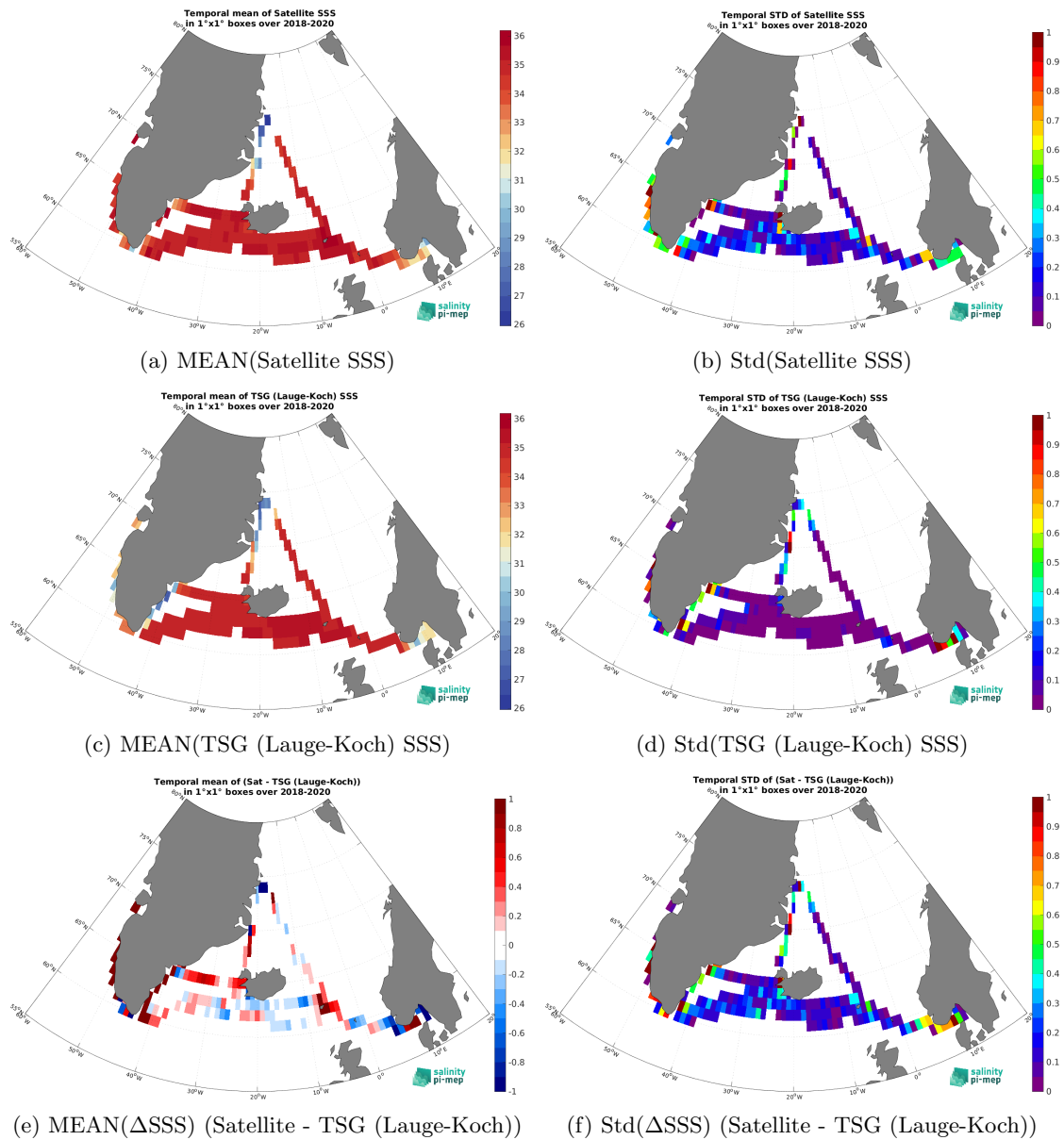
Figure 7: Temporal mean (left) and Std (right) of SSS from SMAP SSS L3 v5.3 - 8-Day running (RSS) (top), TSG (Lauge-Koch) (middle), and of \Delta SSS (Satellite - TSG (Lauge-Koch)). Only match-up pairs are used to generate these maps.
