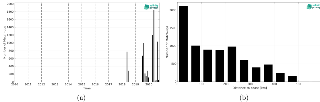
Figure 2: Number of match-ups between TSG (Lauge-Koch) and SMAP SSS L3 v5.3 - 8-Day running (RSS) SSS as a function of time (a) and as function of the distance to coast (b) over the Global Ocean Pi-MEP region and for the full satellite product period.
