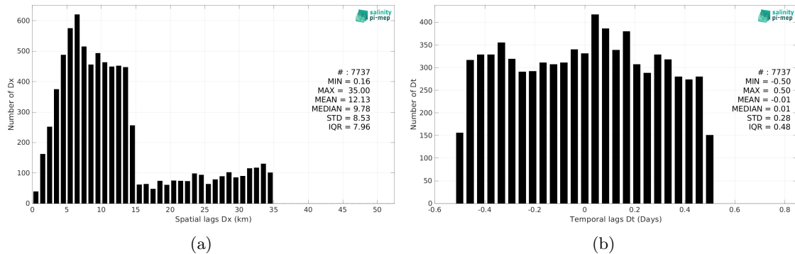
Figure 6: Histograms of the spatial (a) and temporal (b) lags between the location/time of the TSG (Lauge-Koch) measurement and the date of the corresponding SMAP SSS L3 v5.3 - 8-Day running (RSS) SSS pixel.
