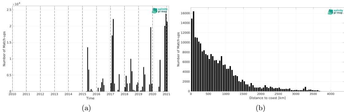
Figure 2: Number of match-ups between TSG (GOSUD-Sailing-ship) and SMAP SSS L3 v5.3 - 8-Day running (RSS) SSS as a function of time (a) and as function of the distance to coast (b) over the Global Ocean Pi-MEP region and for the full satellite product period.
