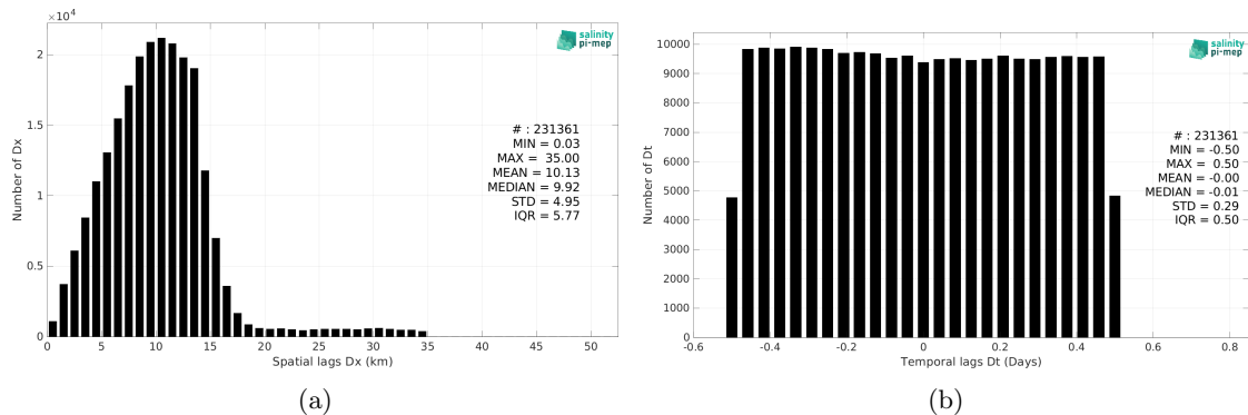
Figure 6: Histograms of the spatial (a) and temporal (b) lags between the location/time of the TSG (GOSUD-Sailing-ship) measurement and the date of the corresponding SMAP SSS L3 v5.3 - 8-Day running (RSS) SSS pixel.
