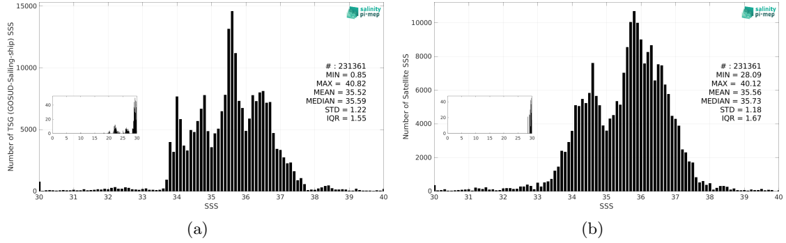
Figure 3: Histograms of SSS from TSG (GOSUD-Sailing-ship) (a) and SMAP SSS L3 v5.3 - 8-Day running (RSS) (b) considering all match-up pairs per bins of 0.1 over the Global Ocean Pi-MEP region and for the full satellite product period.
