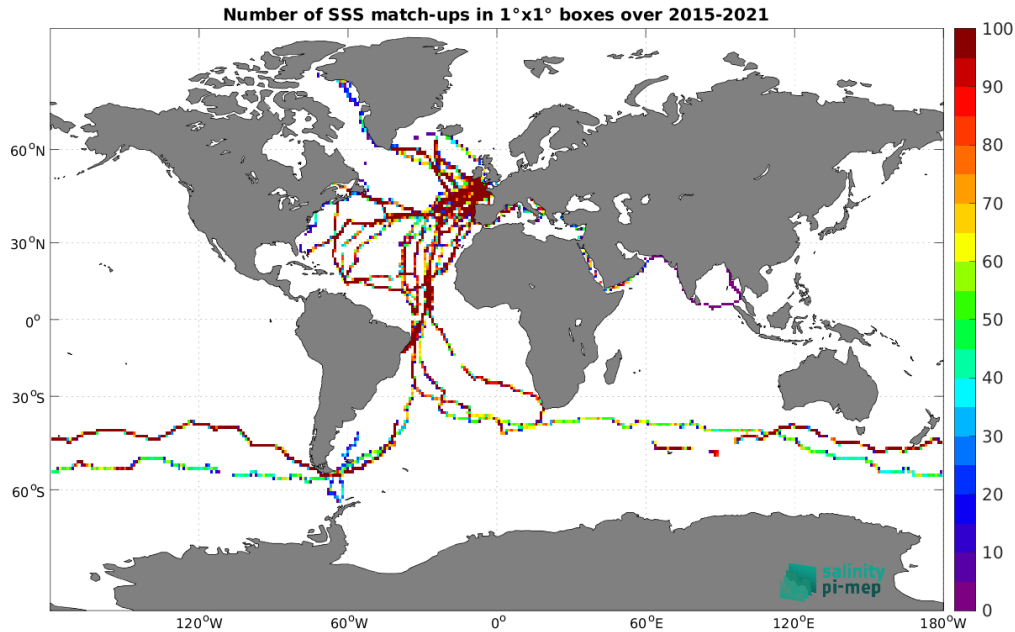
Figure 5: Number of SSS match-ups between TSG (GOSUD-Sailing-ship) SSS and the SMAP SSS L3 v5.3 - 8-Day running (RSS) SSS product for the Global Ocean Pi-MEP region over 1^\circ \times 1^\circ boxes and for the full satellite product period.
