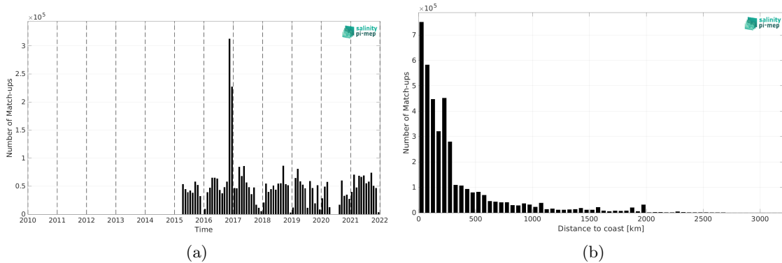
Figure 2: Number of match-ups between TSG (GOSUD-Research-vessel) and SMAP SSS L3 v5.3 - 8-Day running (RSS) SSS as a function of time (a) and as function of the distance to coast (b) over the Global Ocean Pi-MEP region and for the full satellite product period.
