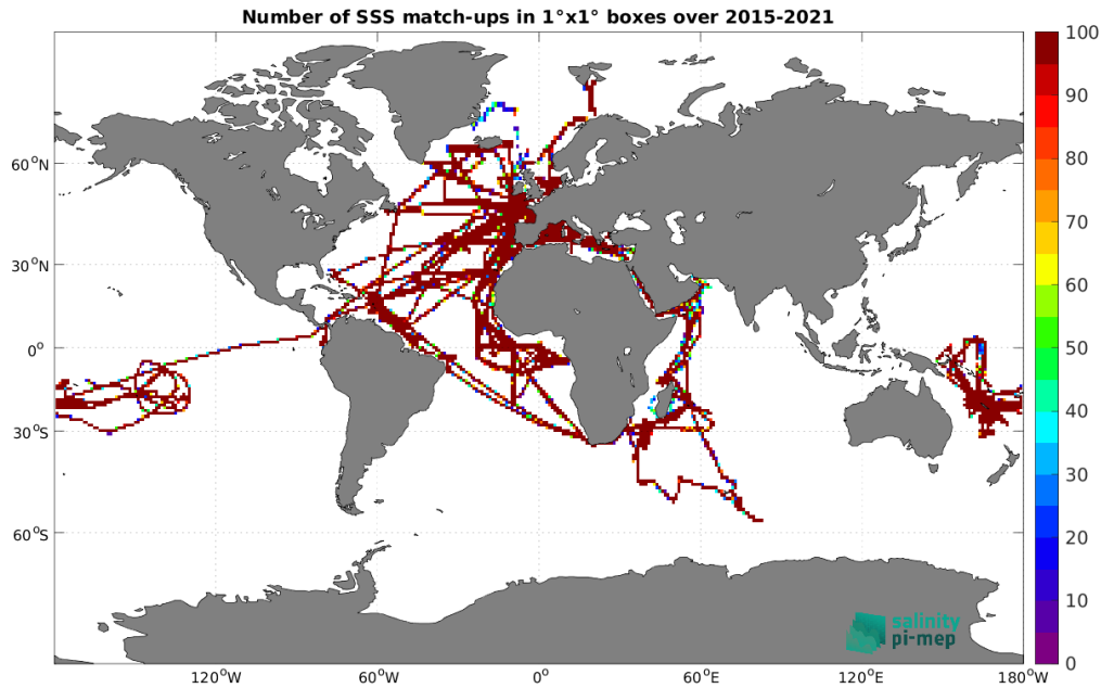
Figure 5: Number of SSS match-ups between TSG (GOSUD-Research-vessel) SSS and the SMAP SSS L3 v5.3 - 8-Day running (RSS) SSS product for the Global Ocean Pi-MEP region over 1^\circ \times 1^\circ boxes and for the full satellite product period.
