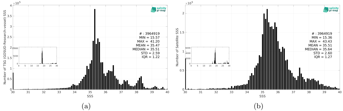
Figure 3: Histograms of SSS from TSG (GOSUD-Research-vessel) (a) and SMAP SSS L3 v5.3 - 8-Day running (RSS) (b) considering all match-up pairs per bins of 0.1 over the Global Ocean Pi-MEP region and for the full satellite product period.
