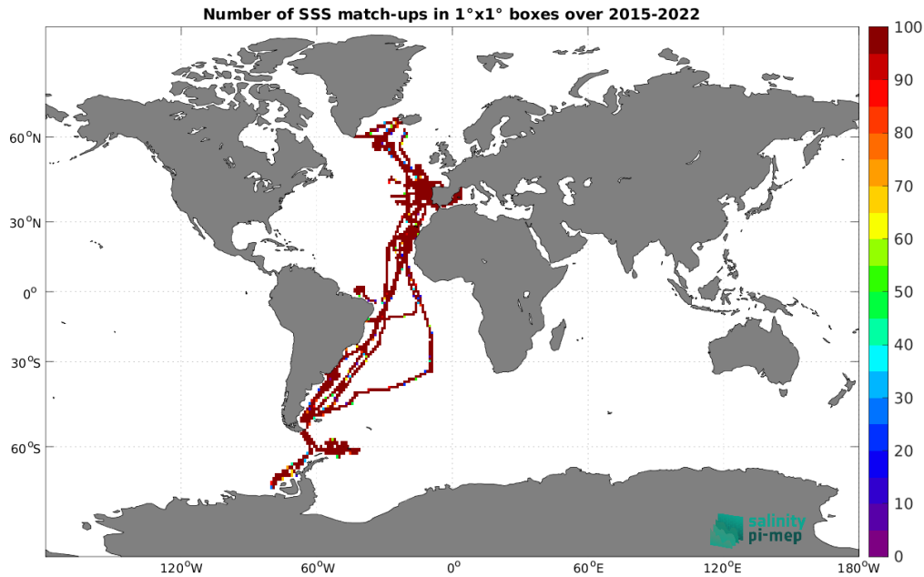
Figure 5: Number of SSS match-ups between TSG (CSIC-UTM) SSS and the SMAP SSS L3 v5.3 - 8-Day running (RSS) SSS product for the Global Ocean Pi-MEP region over 1°x1° boxes and for the full satellite product period.
