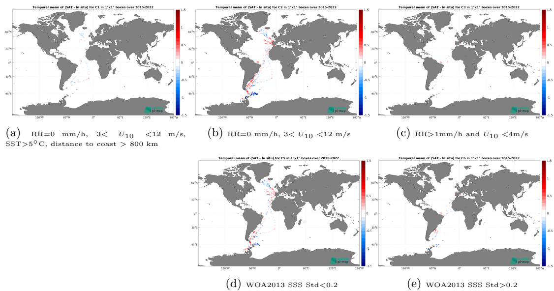
Figure 14: Temporal mean gridded over spatial boxes of size 1^\circ \times 1^\circ of \Delta SSS (SMAP SSS L3 v5.3 - 8-Day running (RSS) - TSG (CSIC-UTM)) for 5 different subdatasets corresponding to:RR=0 mm/h, 3 < U_{10} < 12 m/s, SST > 5^\circ\text{C} , distance to coast > 800 km (a), RR=0 mm/h, 3 < U_{10} < 12 m/s (b), RR > 1 mm/h and U_{10} < 4 m/s (c), WOA2013 SSS Std < 0.2 (d), WOA2013 SSS Std > 0.2 (e).
