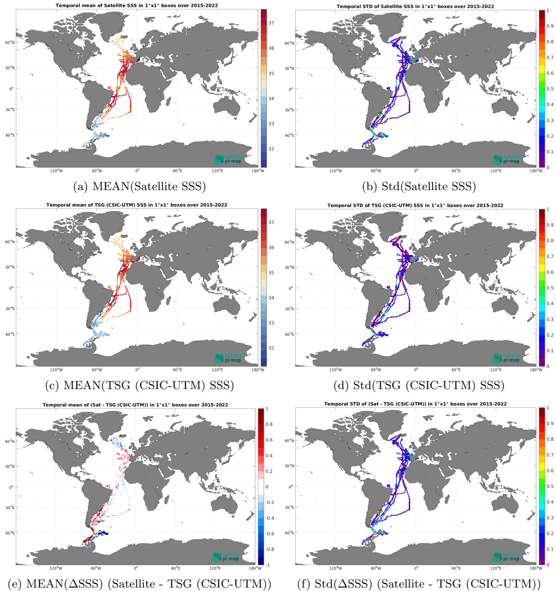
Figure 7: Temporal mean (left) and Std (right) of SSS from SMAP SSS L3 v5.3 - 8-Day running (RSS) (top), TSG (CSIC-UTM) (middle), and of \Delta SSS (Satellite - TSG (CSIC-UTM)). Only match-up pairs are used to generate these maps.
