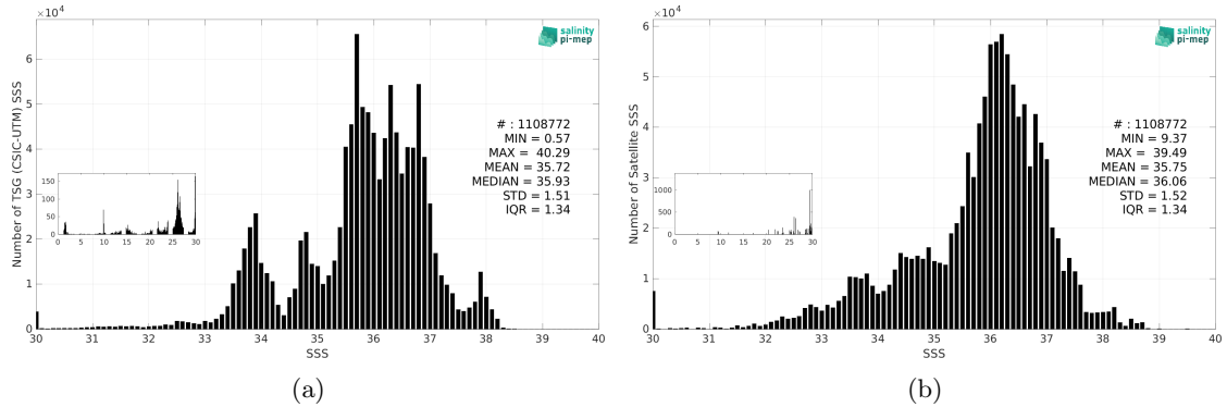
Figure 3: Histograms of SSS from TSG (CSIC-UTM) (a) and SMAP SSS L3 v5.3 - 8-Day running (RSS) (b) considering all match-up pairs per bins of 0.1 over the Global Ocean Pi-MEP region and for the full satellite product period.
