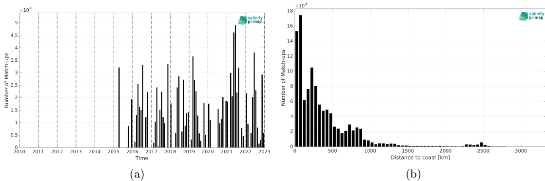
Figure 2: Number of match-ups between TSG (CSIC-UTM) and SMAP SSS L3 v5.3 - 8-Day running (RSS) SSS as a function of time (a) and as function of the distance to coast (b) over the Global Ocean Pi-MEP region and for the full satellite product period.
