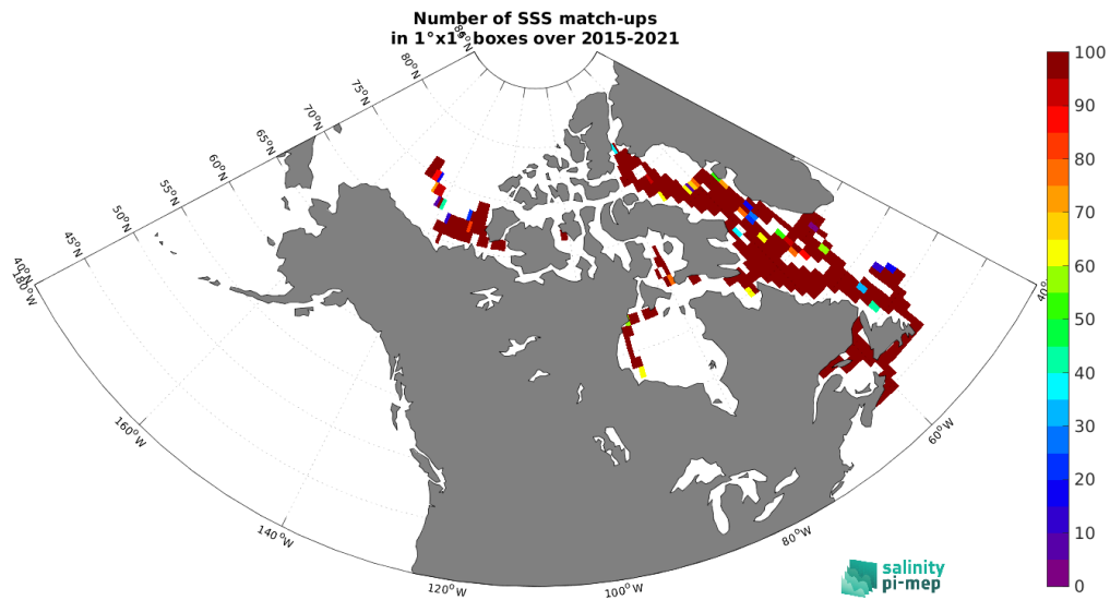
Figure 5: Number of SSS match-ups between TSG (Amundsen) SSS and the SMAP SSS L3 v5.3 - 8-Day running (RSS) SSS product for the Global Ocean Pi-MEP region over 1^\circ \times 1^\circ boxes and for the full satellite product period.
