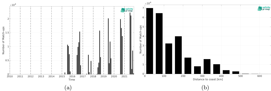
Figure 2: Number of match-ups between TSG (Amundsen) and SMAP SSS L3 v5.3 - 8-Day running (RSS) SSS as a function of time (a) and as function of the distance to coast (b) over the Global Ocean Pi-MEP region and for the full satellite product period.
