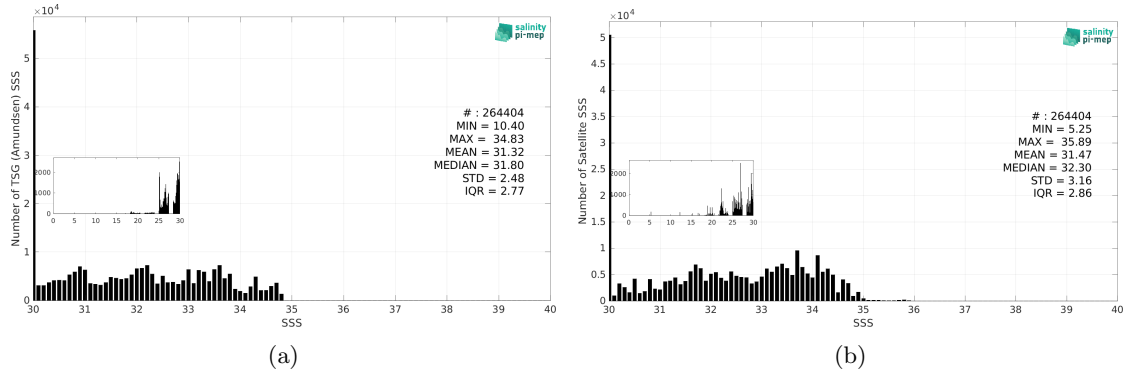
Figure 3: Histograms of SSS from TSG (Amundsen) (a) and SMAP SSS L3 v5.3 - 8-Day running (RSS) (b) considering all match-up pairs per bins of 0.1 over the Global Ocean Pi-MEP region and for the full satellite product period.
