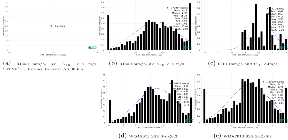
Figure 15: Normalized histogram of \Delta SSS (SMAP SSS L3 v5.3 - 8-Day running (RSS) - TSG (Amundsen)) for 5 different subdatasets corresponding to: RR=0 mm/h, 3 < U_{10} < 12 m/s, SST > 5°C, distance to coast > 800 km (a), RR=0 mm/h, 3 < U_{10} < 12 m/s (b), RR > 1mm/h and U_{10} < 4 m/s (c), WOA2013 SSS Std < 0.2 (d), WOA2013 SSS Std > 0.2 (e).
