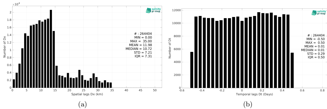
Figure 6: Histograms of the spatial (a) and temporal (b) lags between the location/time of the TSG (Amundsen) measurement and the date of the corresponding SMAP SSS L3 v5.3 - 8-Day running (RSS) SSS pixel.
