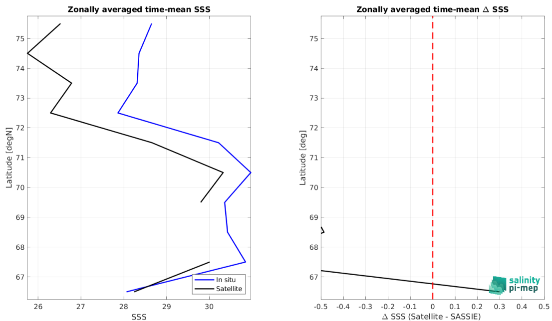
Figure 9: Left panel: Zonal mean SSS from SMAP SSS L3 v5.3 - 8-Day running (RSS) satellite product (black) and from SASSIE (blue). Right panel: Zonal mean of \Delta SSS (Satellite - SASSIE) for all the collected Pi-MEP match-up pairs estimated over the full satellite product period.
