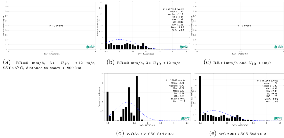
Figure 15: Normalized histogram of \Delta SSS (SMAP SSS L3 v5.3 - 8-Day running (RSS) - SASSIE) for 5 different subdatasets corresponding to: RR=0 mm/h, 3 < U_{10} < 12 m/s, SST > 5°C, distance to coast > 800 km (a), RR=0 mm/h, 3 < U_{10} < 12 m/s (b), RR > 1mm/h and U_{10} < 4 m/s (c), WOA2013 SSS Std < 0.2 (d), WOA2013 SSS Std > 0.2 (e).
