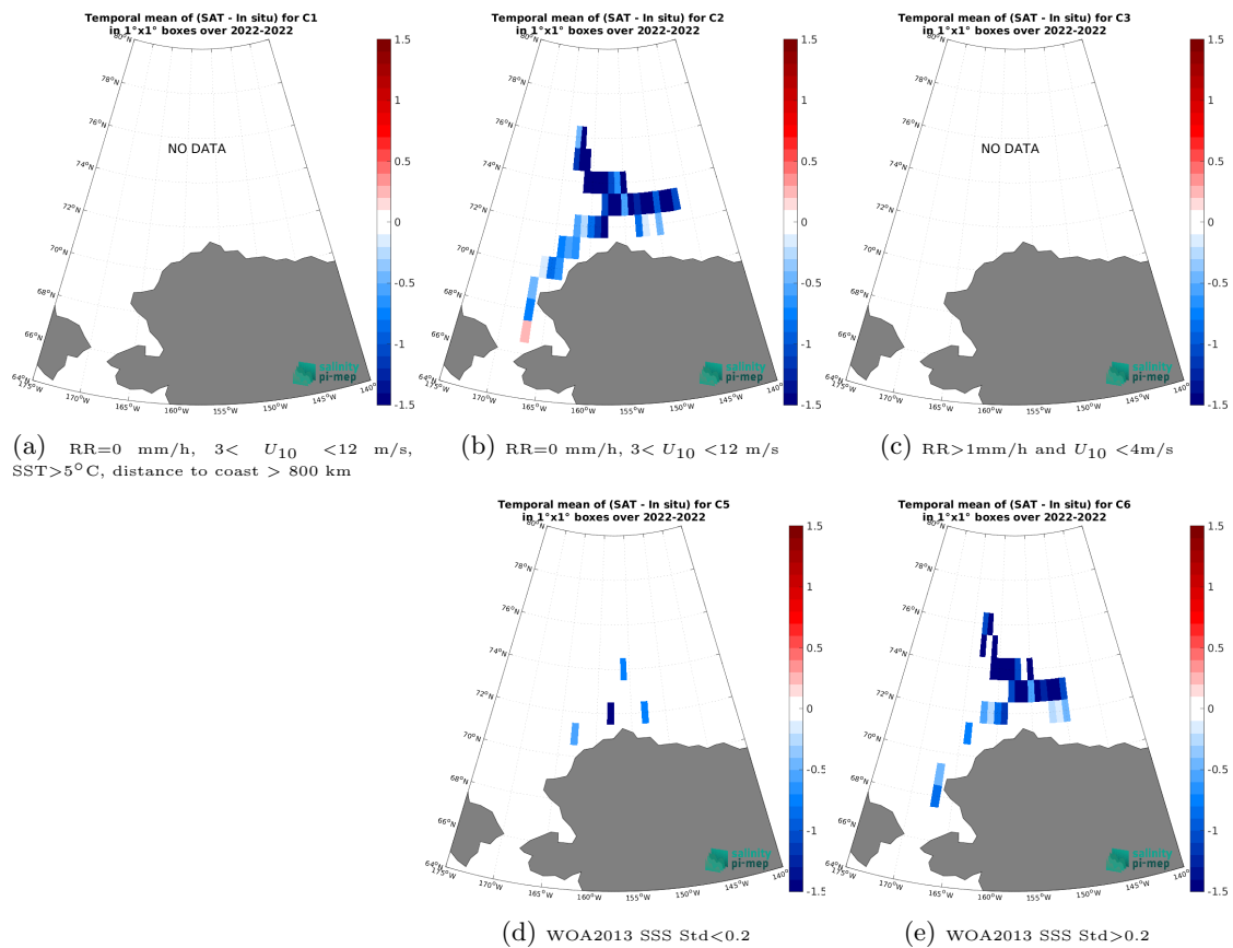
Figure 14: Temporal mean gridded over spatial boxes of size 1^\circ \times 1^\circ of \Delta SSS (SMAP SSS L3 v5.3 - 8-Day running (RSS) - SASSIE) for 5 different subdatasets corresponding to:RR=0 mm/h, 3 < U_{10} < 12 m/s, SST >5^\circ\text{C} , distance to coast > 800 km (a), RR=0 mm/h, 3 < U_{10} < 12 m/s (b), RR >1 mm/h and U_{10} < 4 m/s (c), WOA2013 SSS Std <0.2 (d), WOA2013 SSS Std >0.2 (e).
