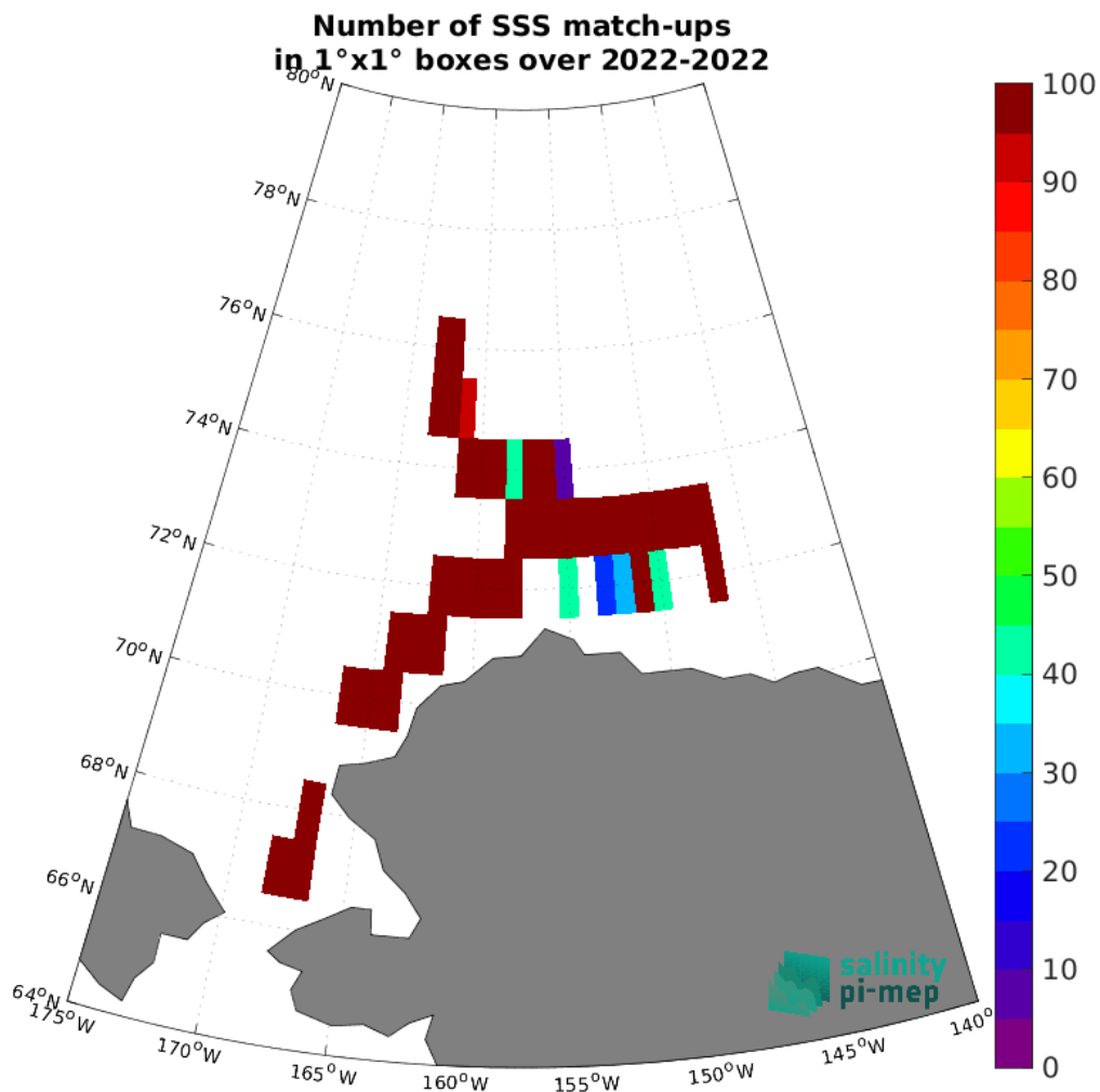
Figure 5: Number of SSS match-ups between SASSIE SSS and the SMAP SSS L3 v5.3 - 8-Day running (RSS) SSS product for the Global Ocean Pi-MEP region over 1^\circ \times 1^\circ boxes and for the full satellite product period.
