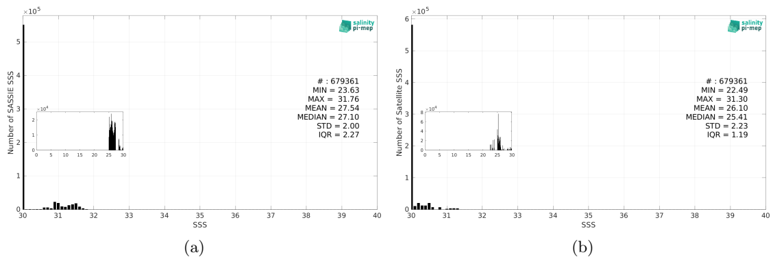
Figure 3: Histograms of SSS from SASSIE (a) and SMAP SSS L3 v5.3 - 8-Day running (RSS) (b) considering all match-up pairs per bins of 0.1 over the Global Ocean Pi-MEP region and for the full satellite product period.
