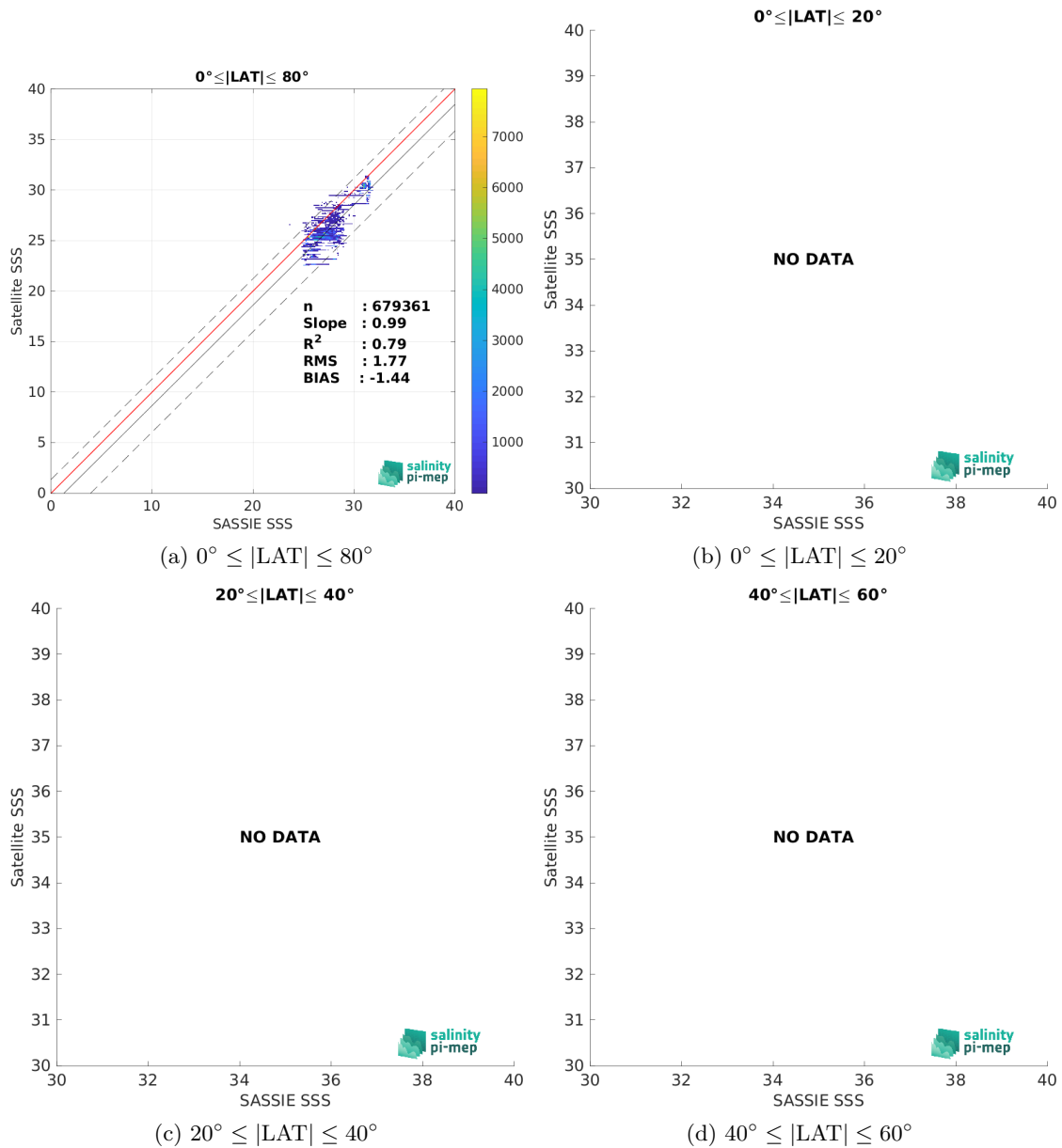
Figure 10: Contour maps of the concentration of SMAP SSS L3 v5.3 - 8-Day running (RSS) SSS (y-axis) versus SASSIE SSS (x-axis) at match-up pairs for different latitude bands. For each plot, the red line shows x=y . The black thin and dashed lines indicate a linear fit through the data cloud and the \pm 95\% confidence levels, respectively. The number match-up pairs n , the slope and R^2 coefficient of the linear fit, the root mean square (RMS) and the mean bias between satellite and in situ data are indicated for each latitude band in each plots.
