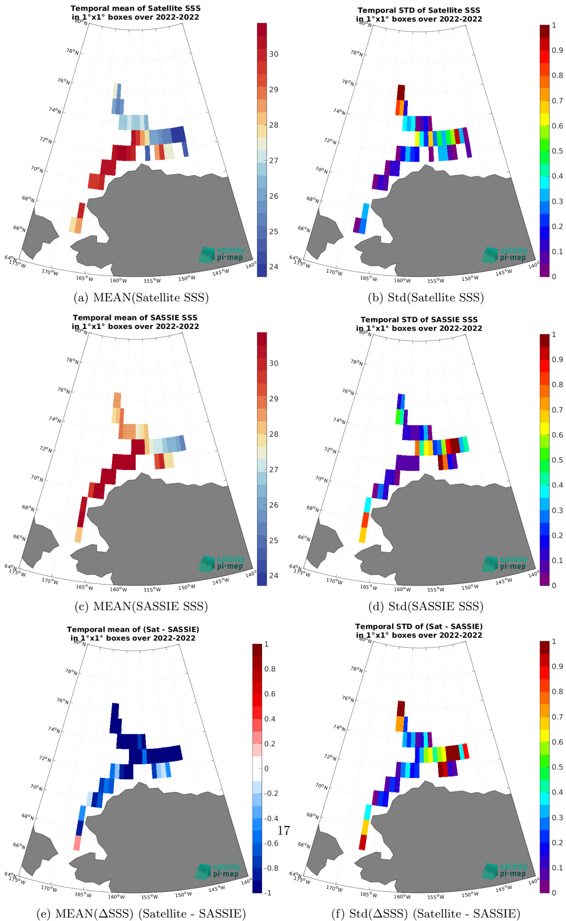
Figure 7: Temporal mean (left) and Std (right) of SSS from SMAP SSS L3 v5.3 - 8-Day running (RSS) (top), SASSIE (middle), and of \Delta SSS (Satellite - SASSIE). Only match-up pairs are used to generate these maps.
