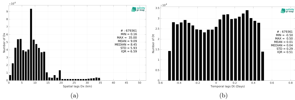
Figure 6: Histograms of the spatial (a) and temporal (b) lags between the location/time of the SASSIE measurement and the date of the corresponding SMAP SSS L3 v5.3 - 8-Day running (RSS) SSS pixel.
