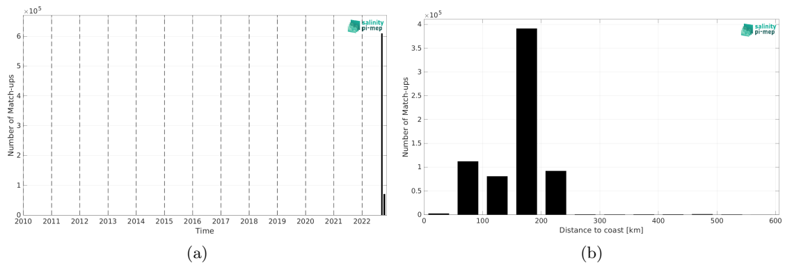
Figure 2: Number of match-ups between SASSIE and SMAP SSS L3 v5.3 - 8-Day running (RSS) SSS as a function of time (a) and as function of the distance to coast (b) over the Global Ocean Pi-MEP region and for the full satellite product period.
