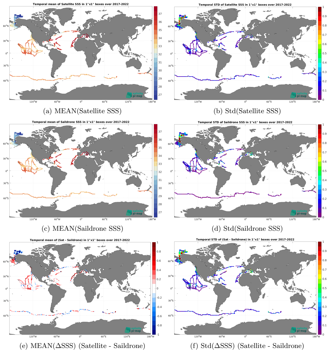
Figure 7: Temporal mean (left) and Std (right) of SSS from SMAP SSS L3 v5.3 - 8-Day running (RSS) (top), Saildrone (middle), and of \Delta SSS (Satellite - Saildrone). Only match-up pairs are used to generate these maps.
