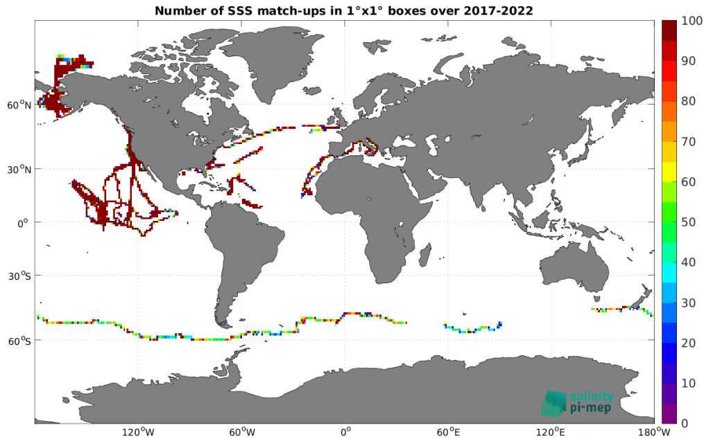
Figure 5: Number of SSS match-ups between Saildrone SSS and the SMAP SSS L3 v5.3 - 8-Day running (RSS) SSS product for the Global Ocean Pi-MEP region over 1^\circ \times 1^\circ boxes and for the full satellite product period.
