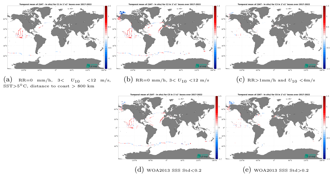
Figure 14: Temporal mean gridded over spatial boxes of size 1^\circ \times 1^\circ of \Delta SSS (SMAP SSS L3 v5.3 - 8-Day running (RSS) - Sailability) for 5 different subdatasets corresponding to:RR=0 mm/h, 3 < U_{10} < 12 m/s, SST > 5^\circ\text{C} , distance to coast > 800 km (a), RR=0 mm/h, 3 < U_{10} < 12 m/s (b), RR > 1 mm/h and U_{10} < 4 m/s (c), WOA2013 SSS Std < 0.2 (d), WOA2013 SSS Std > 0.2 (e).
