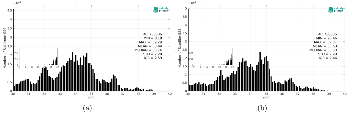
Figure 3: Histograms of SSS from Saildrone (a) and SMAP SSS L3 v5.3 - 8-Day running (RSS) (b) considering all match-up pairs per bins of 0.1 over the Global Ocean Pi-MEP region and for the full satellite product period.
