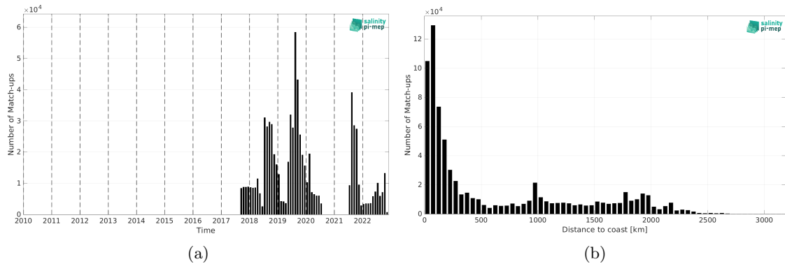
Figure 2: Number of match-ups between Saildrone and SMAP SSS L3 v5.3 - 8-Day running (RSS) SSS as a function of time (a) and as function of the distance to coast (b) over the Global Ocean Pi-MEP region and for the full satellite product period.
