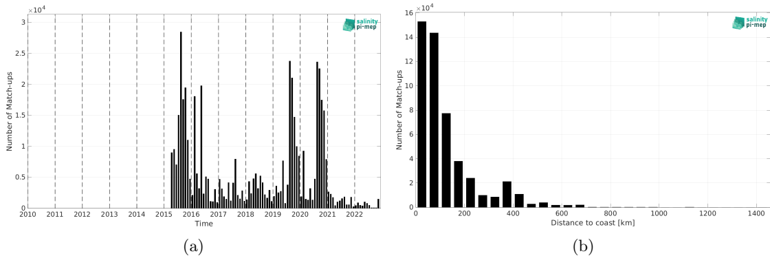
Figure 2: Number of match-ups between ICES and SMAP SSS L3 v5.3 - 8-Day running (RSS) SSS as a function of time (a) and as function of the distance to coast (b) over the Global Ocean Pi-MEP region and for the full satellite product period.
