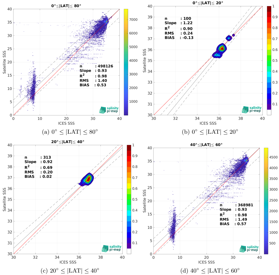
Figure 10: Contour maps of the concentration of SMAP SSS L3 v5.3 - 8-Day running (RSS) SSS (y-axis) versus ICES SSS (x-axis) at match-up pairs for different latitude bands. For each plot, the red line shows x=y . The black thin and dashed lines indicate a linear fit through the data cloud and the \pm 95\% confidence levels, respectively. The number match-up pairs n , the slope and R^2 coefficient of the linear fit, the root mean square (RMS) and the mean bias between satellite and in situ data are indicated for each latitude band in each plots.
