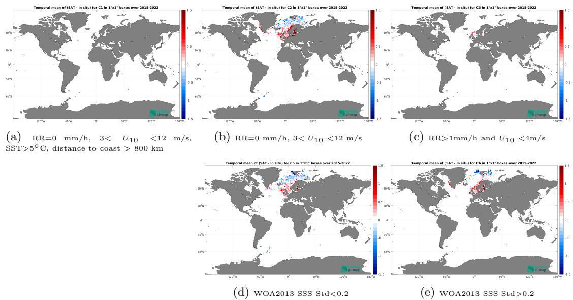
Figure 14: Temporal mean gridded over spatial boxes of size 1^\circ \times 1^\circ of \Delta SSS (SMAP SSS L3 v5.3 - 8-Day running (RSS) - ICES) for 5 different subdatasets corresponding to:RR=0 mm/h, 3 < U_{10} < 12 m/s, SST >5^\circ C, distance to coast > 800 km (a), RR=0 mm/h, 3 < U_{10} < 12 m/s (b), RR >1 mm/h and U_{10} < 4 m/s (c), WOA2013 SSS Std <0.2 (d), WOA2013 SSS Std >0.2 (e).
