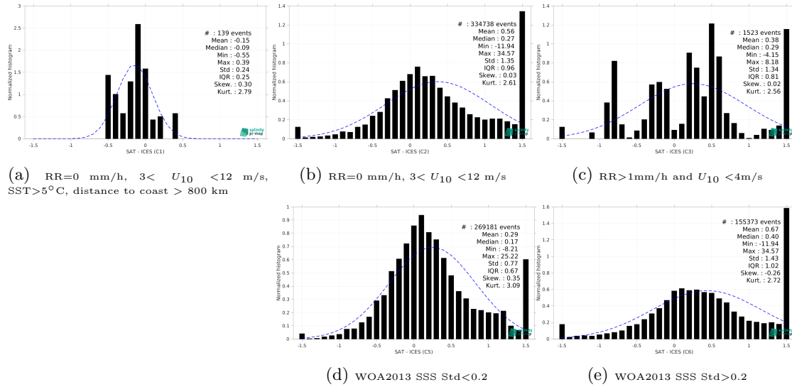
Figure 15: Normalized histogram of \Delta SSS (SMAP SSS L3 v5.3 - 8-Day running (RSS) - ICES) for 5 different subdatasets corresponding to: RR=0 mm/h, 3 < U_{10} < 12 m/s, SST > 5°C, distance to coast > 800 km (a), RR=0 mm/h, 3 < U_{10} < 12 m/s (b), RR > 1mm/h and U_{10} < 4 m/s (c), WOA2013 SSS Std < 0.2 (d), WOA2013 SSS Std > 0.2 (e).
