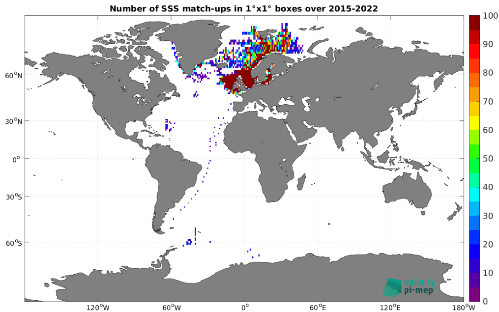
Figure 5: Number of SSS match-ups between ICES SSS and the SMAP SSS L3 v5.3 - 8-Day running (RSS) SSS product for the Global Ocean Pi-MEP region over 1^\circ \times 1^\circ boxes and for the full satellite product period.
