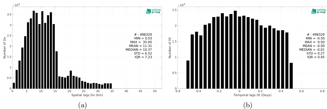
Figure 6: Histograms of the spatial (a) and temporal (b) lags between the location/time of the ICES measurement and the date of the corresponding SMAP SSS L3 v5.3 - 8-Day running (RSS) SSS pixel.
