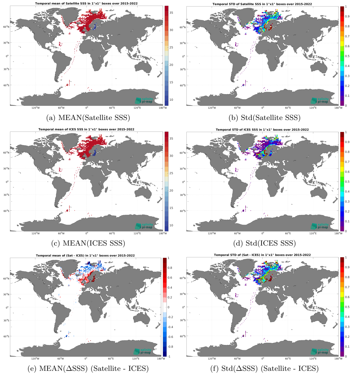
Figure 7: Temporal mean (left) and Std (right) of SSS from SMAP SSS L3 v5.3 - 8-Day running (RSS) (top), ICES (middle), and of \Delta SSS (Satellite - ICES). Only match-up pairs are used to generate these maps.
