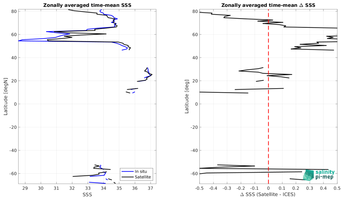
Figure 9: Left panel: Zonal mean SSS from SMAP SSS L3 v5.3 - 8-Day running (RSS) satellite product (black) and from ICES (blue). Right panel: Zonal mean of \Delta SSS (Satellite - ICES) for all the collected Pi-MEP match-up pairs estimated over the full satellite product period.
