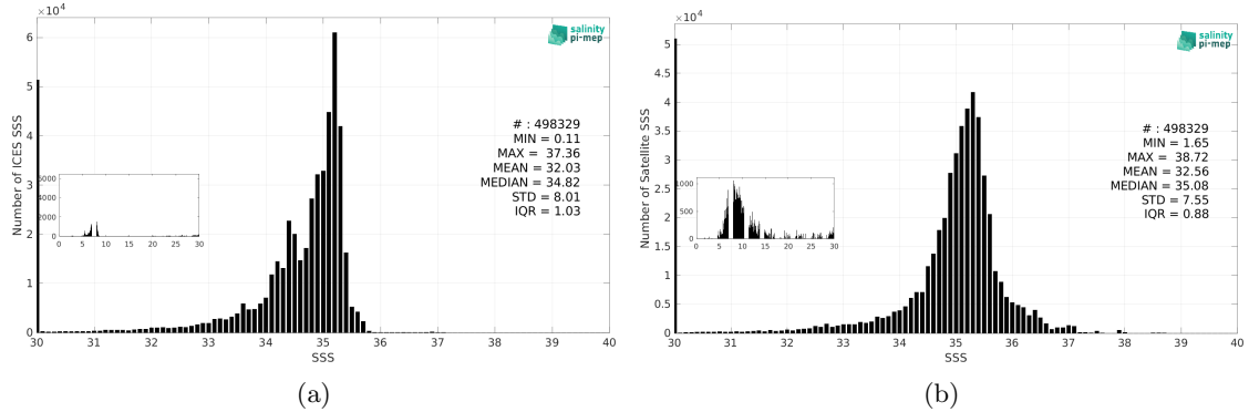
Figure 3: Histograms of SSS from ICES (a) and SMAP SSS L3 v5.3 - 8-Day running (RSS) (b) considering all match-up pairs per bins of 0.1 over the Global Ocean Pi-MEP region and for the full satellite product period.
