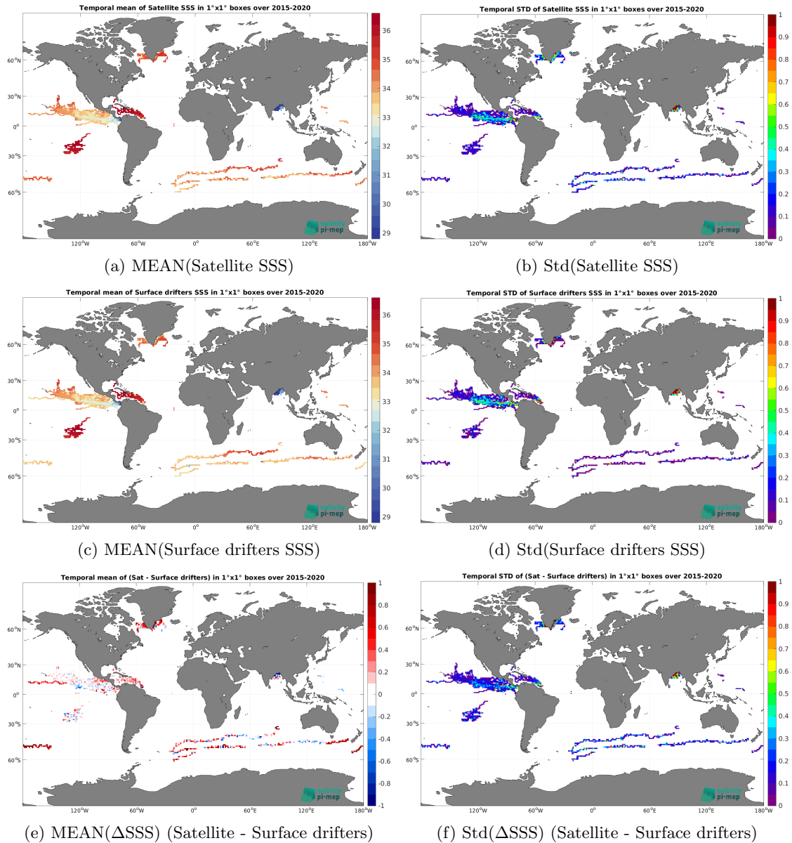
Figure 6: Temporal mean (left) and Std (right) of SSS from SMAP SSS L3 v5.3 - 8-Day running (RSS) (top), Surface drifters (middle), and of \Delta SSS (Satellite - Surface drifters). Only match-up pairs are used to generate these maps.
