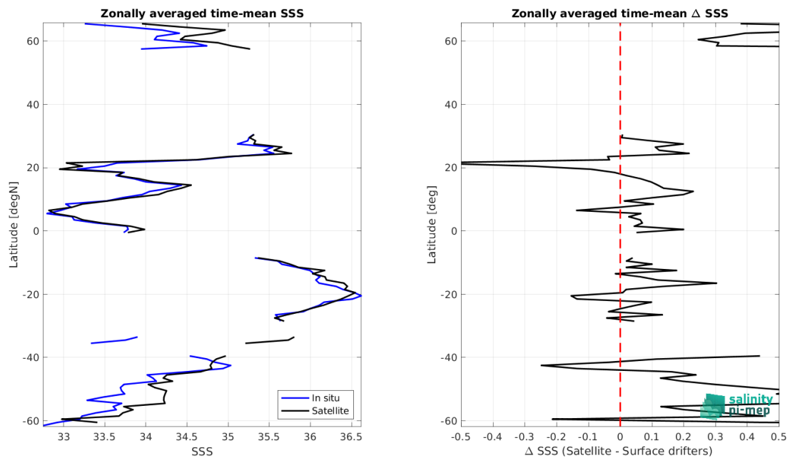
Figure 8: Left panel: Zonal mean SSS from SMAP SSS L3 v5.3 - 8-Day running (RSS) satellite product (black) and from Surface drifters (blue). Right panel: Zonal mean of \Delta SSS (Satellite - Surface drifters) for all the collected Pi-MEP match-up pairs estimated over the full satellite product period.
