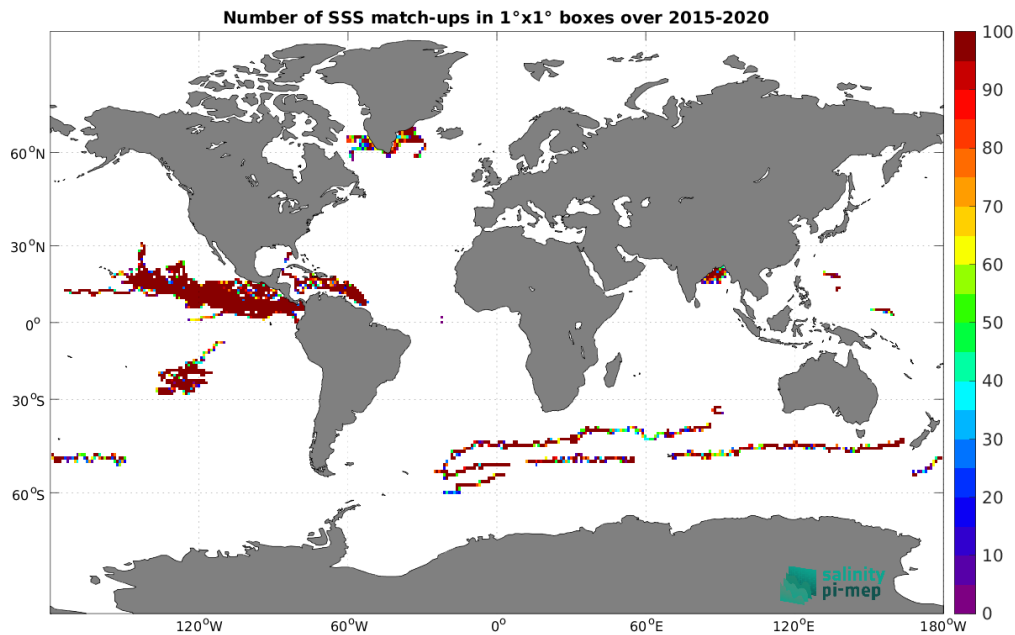
Figure 4: Number of SSS match-ups between Surface drifters SSS and the SMAP SSS L3 v5.3 - 8-Day running (RSS) SSS product for the Global Ocean Pi-MEP region over 1°×1° boxes and for the full satellite product period.
