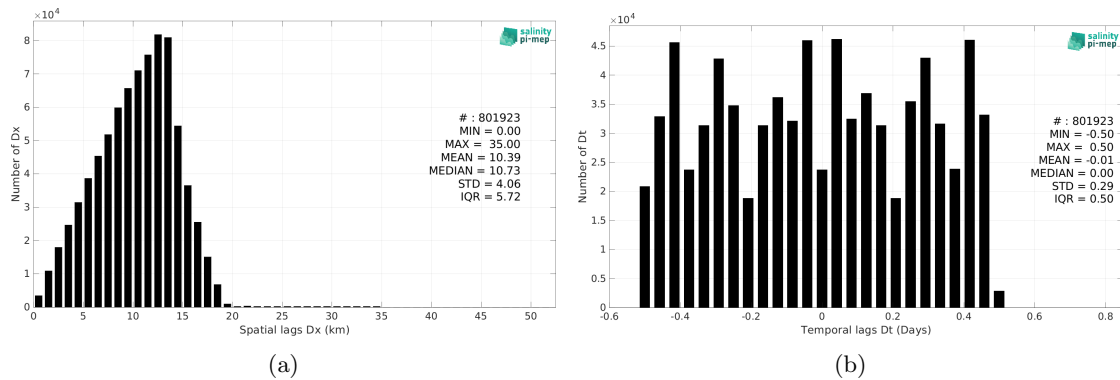
Figure 5: Histograms of the spatial (a) and temporal (b) lags between the location/time of the Surface drifters measurement and the date of the corresponding SMAP SSS L3 v5.3 - 8-Day running (RSS) SSS pixel.
