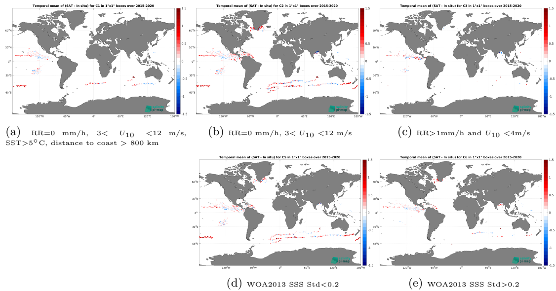
Figure 13: Temporal mean gridded over spatial boxes of size 1^\circ \times 1^\circ of \Delta SSS (SMAP SSS L3 v5.3 - 8-Day running (RSS) - Surface drifters) for 5 different subdatasets corresponding to:RR=0 mm/h, 3 < U_{10} < 12 m/s, SST > 5^\circ\text{C} , distance to coast > 800 km (a), RR=0 mm/h, 3 < U_{10} < 12 m/s (b), RR > 1 mm/h and U_{10} < 4 m/s (c), WOA2013 SSS Std < 0.2 (d), WOA2013 SSS Std > 0.2 (e).
