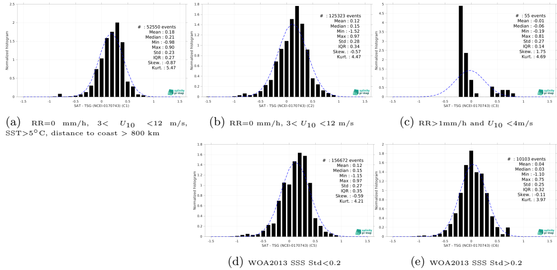
Figure 15: Normalized histogram of \Delta SSS (SMAP SSS L3 v5.3 - Monthly (RSS) - TSG (NCEI-0170743)) for 5 different subdatasets corresponding to: RR=0 mm/h, 3 < U_{10} < 12 m/s, SST > 5°C, distance to coast > 800 km (a), RR=0 mm/h, 3 < U_{10} < 12 m/s (b), RR > 1mm/h and U_{10} < 4 m/s (c), WOA2013 SSS Std < 0.2 (d), WOA2013 SSS Std > 0.2 (e).
