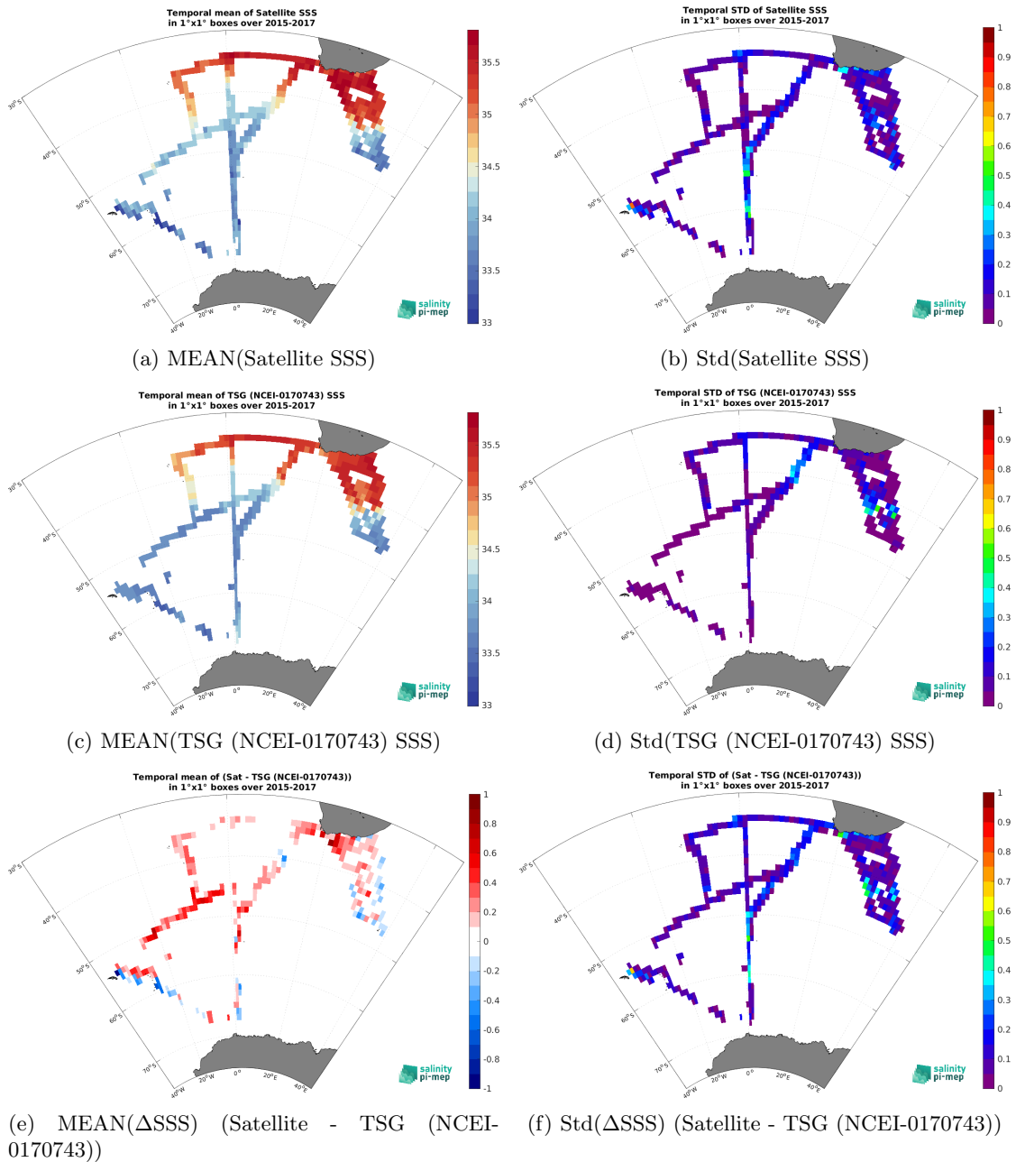
Figure 7: Temporal mean (left) and Std (right) of SSS from SMAP SSS L3 v5.3 - Monthly (RSS) (top), TSG (NCEI-0170743) (middle), and of \Delta SSS (Satellite - TSG (NCEI-0170743)). Only match-up pairs are used to generate these maps.
