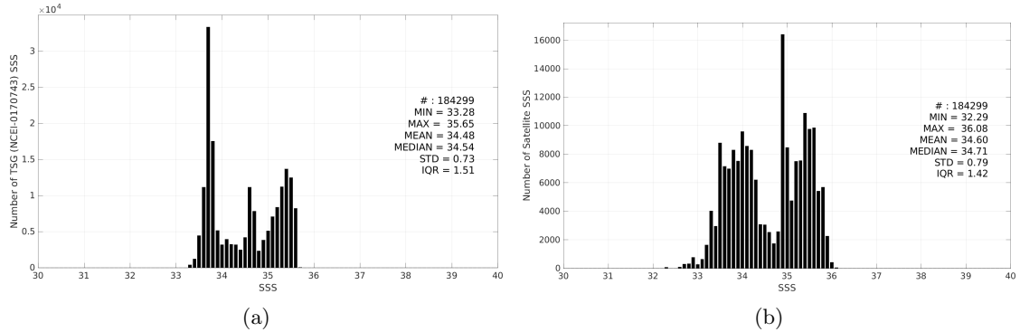
Figure 3: Histograms of SSS from TSG (NCEI-0170743) (a) and SMAP SSS L3 v5.3 - Monthly (RSS) (b) considering all match-up pairs per bins of 0.1 over the Global Ocean Pi-MEP region and for the full satellite product period.
