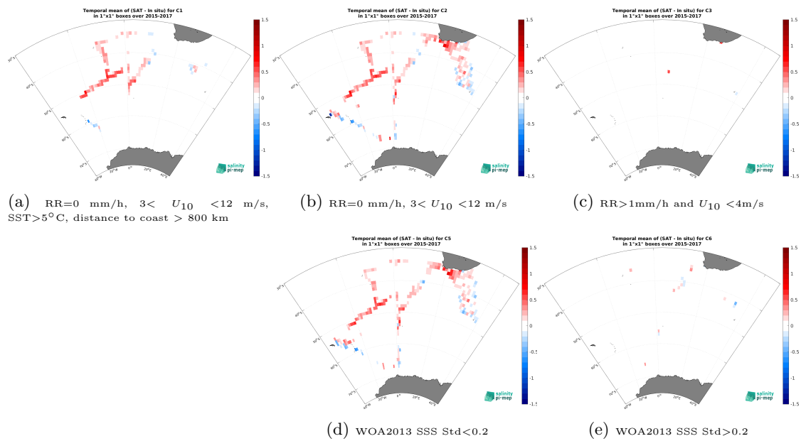
Figure 14: Temporal mean gridded over spatial boxes of size 1^\circ \times 1^\circ of \Delta SSS (SMAP SSS L3 v5.3 - Monthly (RSS) - TSG (NCEI-0170743)) for 5 different subdatasets corresponding to:RR=0 mm/h, 3 < U_{10} < 12 m/s, SST >5^\circ C, distance to coast > 800 km (a), RR=0 mm/h, 3 < U_{10} < 12 m/s (b), RR >1 mm/h and U_{10} < 4 m/s (c), WOA2013 SSS Std <0.2 (d), WOA2013 SSS Std >0.2 (e).
