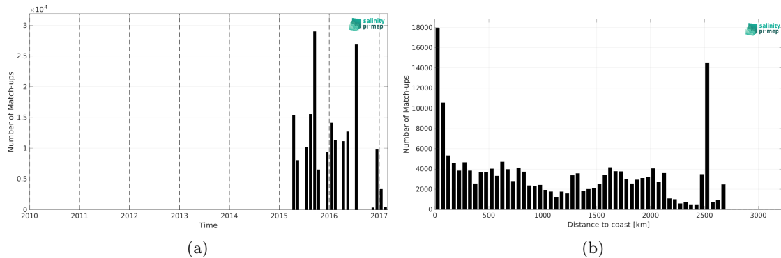
Figure 2: Number of match-ups between TSG (NCEI-0170743) and SMAP SSS L3 v5.3 - Monthly (RSS) SSS as a function of time (a) and as function of the distance to coast (b) over the Global Ocean Pi-MEP region and for the full satellite product period.
