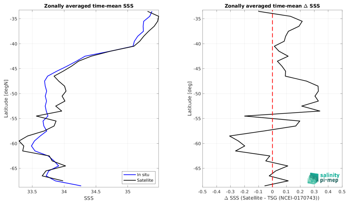
Figure 9: Left panel: Zonal mean SSS from SMAP SSS L3 v5.3 - Monthly (RSS) satellite product (black) and from TSG (NCEI-0170743) (blue). Right panel: Zonal mean of \Delta SSS (Satellite - TSG (NCEI-0170743)) for all the collected Pi-MEP match-up pairs estimated over the full satellite product period.
