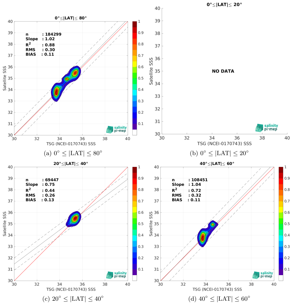
Figure 10: Contour maps of the concentration of SMAP SSS L3 v5.3 - Monthly (RSS) SSS (y-axis) versus TSG (NCEI-0170743) SSS (x-axis) at match-up pairs for different latitude bands. For each plot, the red line shows x=y . The black thin and dashed lines indicate a linear fit through the data cloud and the \pm 95\% confidence levels, respectively. The number match-up pairs n , the slope and R^2 coefficient of the linear fit, the root mean square (RMS) and the mean bias between satellite and in situ data are indicated for each latitude band in each plots.
