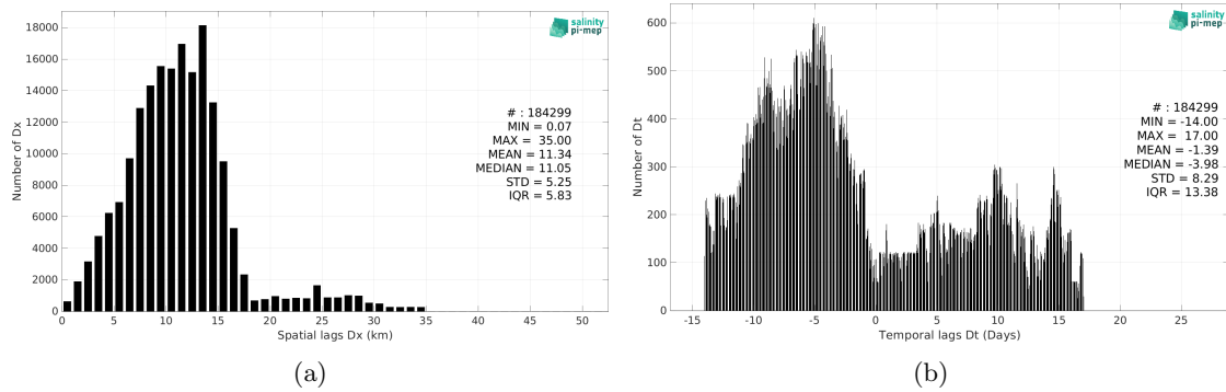
Figure 6: Histograms of the spatial (a) and temporal (b) lags between the location/time of the TSG (NCEI-0170743) measurement and the date of the corresponding SMAP SSS L3 v5.3 - Monthly (RSS) SSS pixel.
