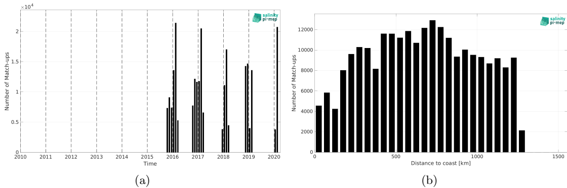
Figure 2: Number of match-ups between TSG (LEGOS-Survostral) and SMAP SSS L3 v5.3 - Monthly (RSS) SSS as a function of time (a) and as function of the distance to coast (b) over the Global Ocean Pi-MEP region and for the full satellite product period.
