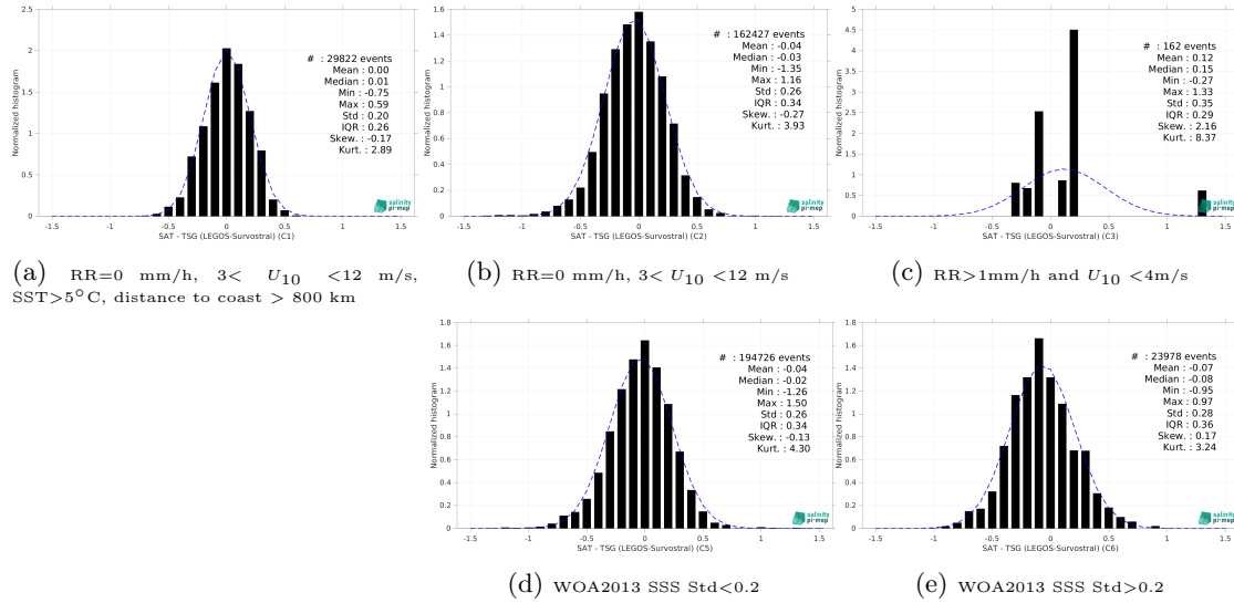
Figure 15: Normalized histogram of \Delta SSS (SMAP SSS L3 v5.3 - Monthly (RSS) - TSG (LEGOS-Survostral)) for 5 different subdatasets corresponding to: RR=0 mm/h, 3 < U_{10} < 12 m/s, SST > 5°C, distance to coast > 800 km (a), RR=0 mm/h, 3 < U_{10} < 12 m/s (b), RR > 1mm/h and U_{10} < 4 m/s (c), WOA2013 SSS Std < 0.2 (d), WOA2013 SSS Std > 0.2 (e).
