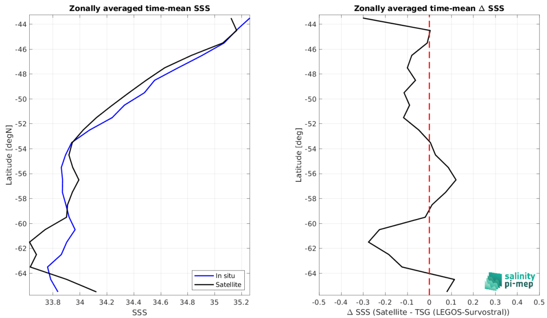
Figure 9: Left panel: Zonal mean SSS from SMAP SSS L3 v5.3 - Monthly (RSS) satellite product (black) and from TSG (LEGOS-Survostral) (blue). Right panel: Zonal mean of \Delta SSS (Satellite - TSG (LEGOS-Survostral)) for all the collected Pi-MEP match-up pairs estimated over the full satellite product period.
