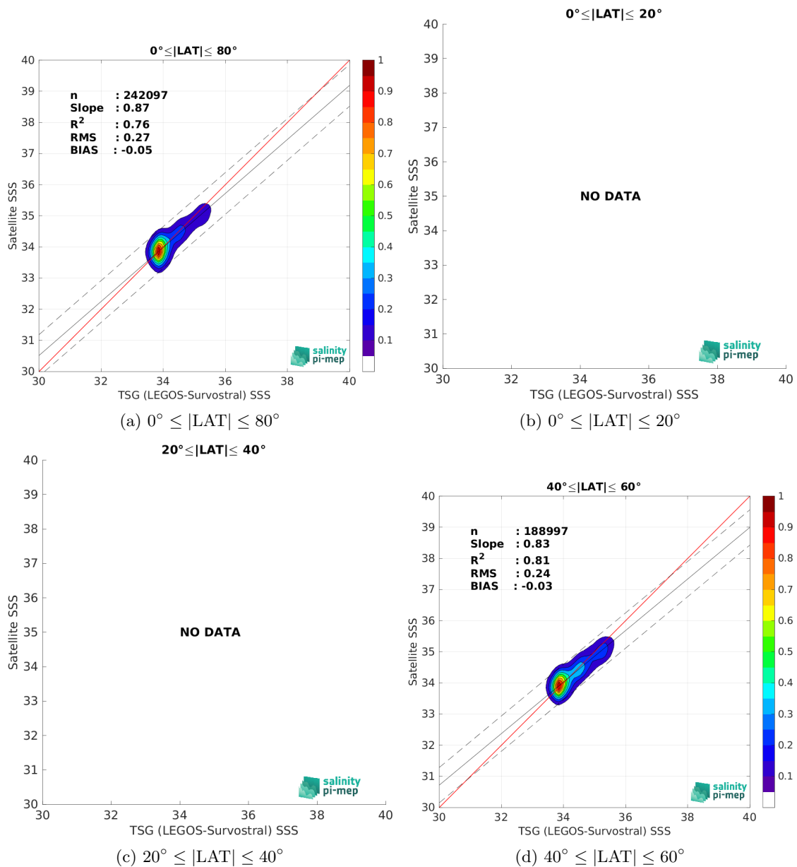
Figure 10: Contour maps of the concentration of SMAP SSS L3 v5.3 - Monthly (RSS) SSS (y-axis) versus TSG (LEGOS-Survostral) SSS (x-axis) at match-up pairs for different latitude bands. For each plot, the red line shows x=y . The black thin and dashed lines indicate a linear fit through the data cloud and the \pm 95\% confidence levels, respectively. The number match-up pairs n , the slope and R^2 coefficient of the linear fit, the root mean square (RMS) and the mean bias between satellite and in situ data are indicated for each latitude band in each plots.
