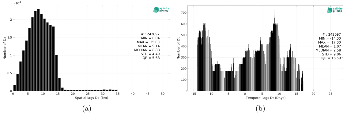
Figure 6: Histograms of the spatial (a) and temporal (b) lags between the location/time of the TSG (LEGOS-Survostral) measurement and the date of the corresponding SMAP SSS L3 v5.3 - Monthly (RSS) SSS pixel.
