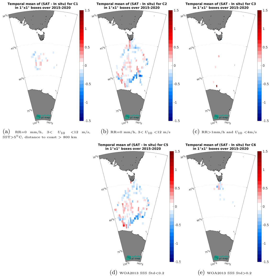
Figure 14: Temporal mean gridded over spatial boxes of size 1^\circ \times 1^\circ of \Delta\text{SSS} (SMAP SSS L3 v5.3 - Monthly (RSS) - TSG (LEGOS-Survostral)) for 5 different subdatasets corresponding to: RR=0 mm/h, 3 < U_{10} < 12 m/s, SST > 5^\circ\text{C} , distance to coast > 800 km (a), RR=0 mm/h, 3 < U_{10} < 12 m/s (b), RR > 1\text{mm/h} and U_{10} < 4\text{m/s} (c), WOA2013 SSS Std < 0.2 (d), WOA2013 SSS Std > 0.2 (e).
