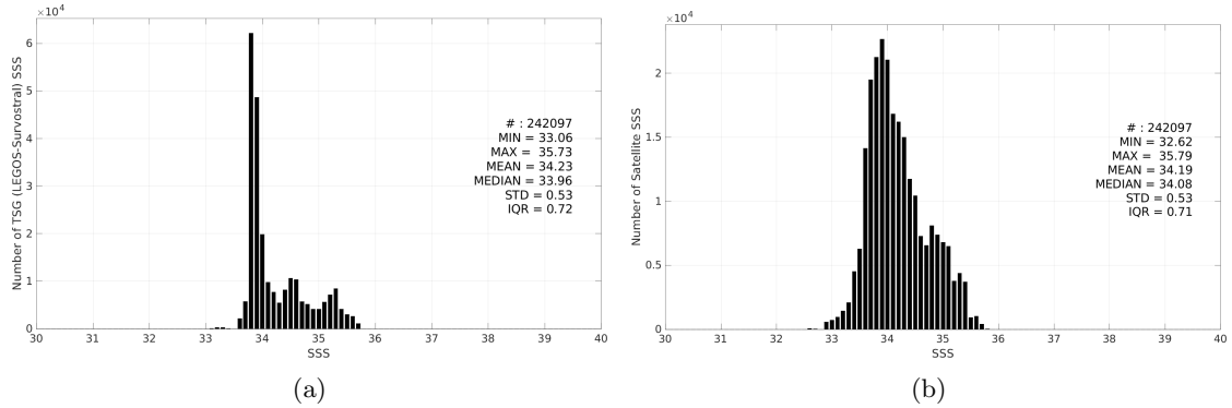
Figure 3: Histograms of SSS from TSG (LEGOS-Survostral) (a) and SMAP SSS L3 v5.3 - Monthly (RSS) (b) considering all match-up pairs per bins of 0.1 over the Global Ocean Pi-MEP region and for the full satellite product period.
