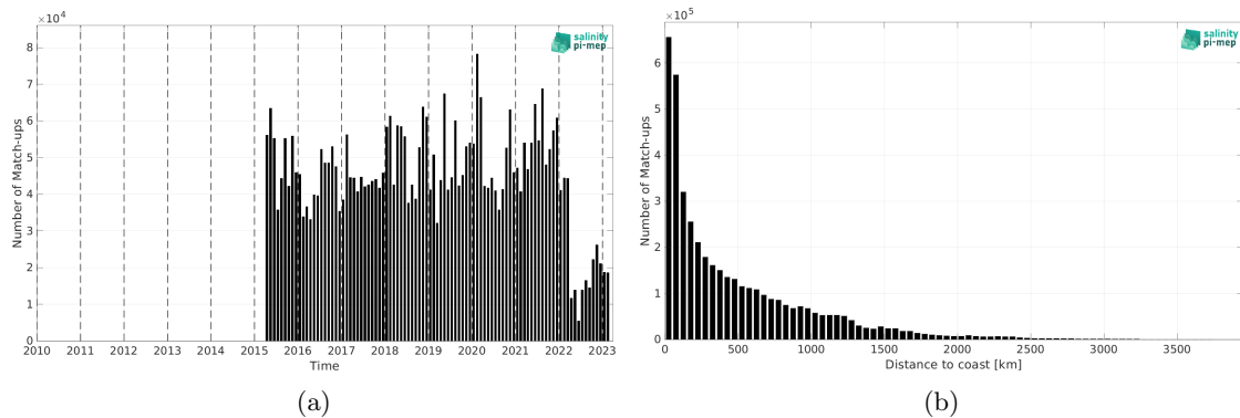
Figure 2: Number of match-ups between TSG (LEGOS-DM) and SMAP SSS L3 v5.3 - Monthly (RSS) SSS as a function of time (a) and as function of the distance to coast (b) over the Global Ocean Pi-MEP region and for the full satellite product period.
