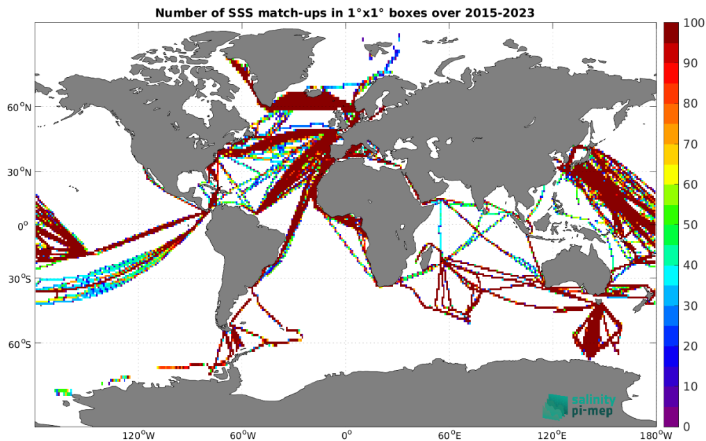
Figure 5: Number of SSS match-ups between TSG (LEGOS-DM) SSS and the SMAP SSS L3 v5.3 - Monthly (RSS) SSS product for the Global Ocean Pi-MEP region over 1^\circ \times 1^\circ boxes and for the full satellite product period.
