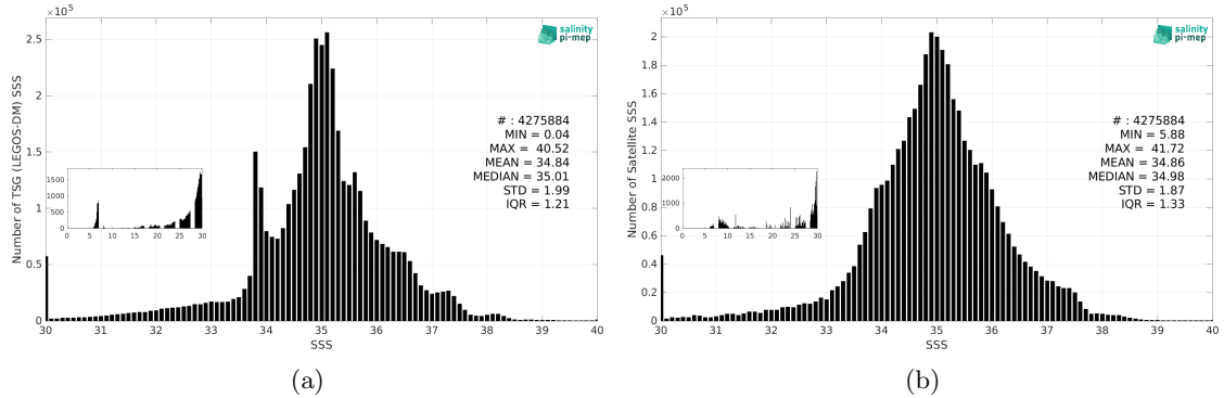
Figure 3: Histograms of SSS from TSG (LEGOS-DM) (a) and SMAP SSS L3 v5.3 - Monthly (RSS) (b) considering all match-up pairs per bins of 0.1 over the Global Ocean Pi-MEP region and for the full satellite product period.
