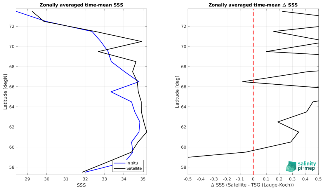
Figure 9: Left panel: Zonal mean SSS from SMAP SSS L3 v5.3 - Monthly (RSS) satellite product (black) and from TSG (Lauge-Koch) (blue). Right panel: Zonal mean of \Delta SSS (Satellite - TSG (Lauge-Koch)) for all the collected Pi-MEP match-up pairs estimated over the full satellite product period.
