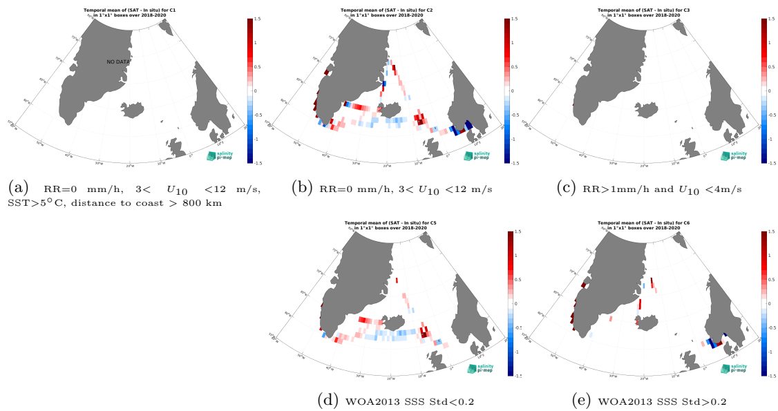
Figure 14: Temporal mean gridded over spatial boxes of size 1^\circ \times 1^\circ of \Delta SSS (SMAP SSS L3 v5.3 - Monthly (RSS) - TSG (Lauge-Koch)) for 5 different subdatasets corresponding to: RR=0 mm/h, 3 < U_{10} < 12 m/s, SST > 5^\circ\text{C} , distance to coast > 800 km (a), RR=0 mm/h, 3 < U_{10} < 12 m/s (b), RR > 1 mm/h and U_{10} < 4 m/s (c), WOA2013 SSS Std < 0.2 (d), WOA2013 SSS Std > 0.2 (e).
