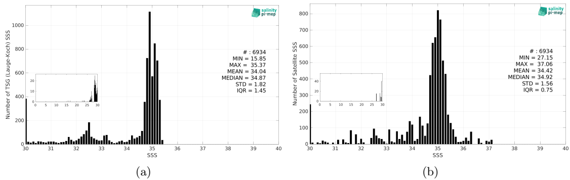
Figure 3: Histograms of SSS from TSG (Lauge-Koch) (a) and SMAP SSS L3 v5.3 - Monthly (RSS) (b) considering all match-up pairs per bins of 0.1 over the Global Ocean Pi-MEP region and for the full satellite product period.
