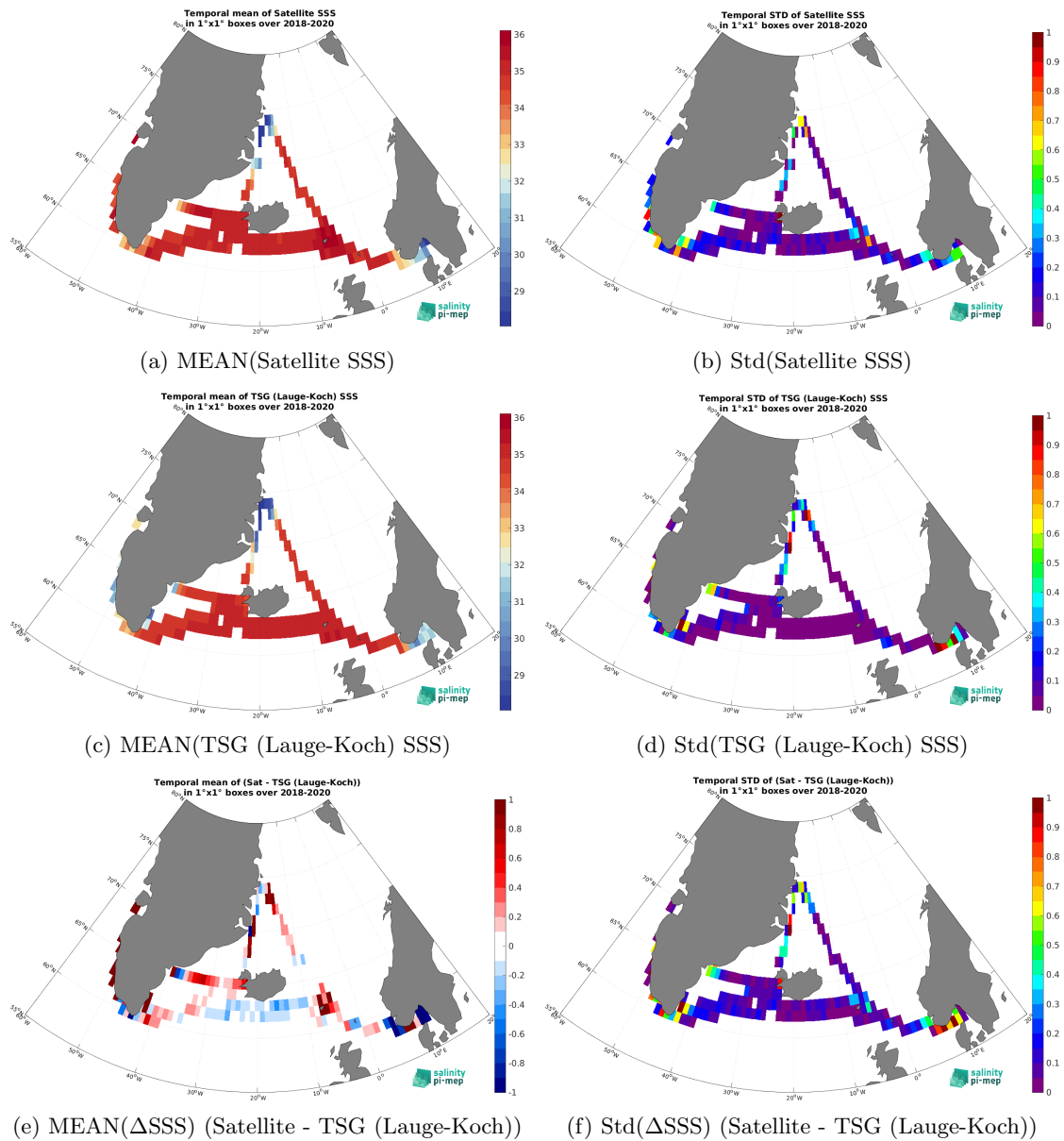
Figure 7: Temporal mean (left) and Std (right) of SSS from SMAP SSS L3 v5.3 - Monthly (RSS) (top), TSG (Lauge-Koch) (middle), and of \Delta SSS (Satellite - TSG (Lauge-Koch)). Only match-up pairs are used to generate these maps.
