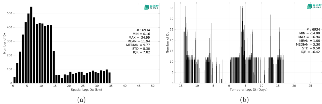
Figure 6: Histograms of the spatial (a) and temporal (b) lags between the location/time of the TSG (Lauge-Koch) measurement and the date of the corresponding SMAP SSS L3 v5.3 - Monthly (RSS) SSS pixel.
