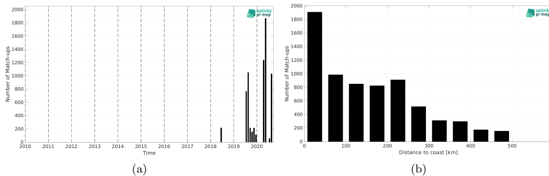
Figure 2: Number of match-ups between TSG (Lauge-Koch) and SMAP SSS L3 v5.3 - Monthly (RSS) SSS as a function of time (a) and as function of the distance to coast (b) over the Global Ocean Pi-MEP region and for the full satellite product period.
