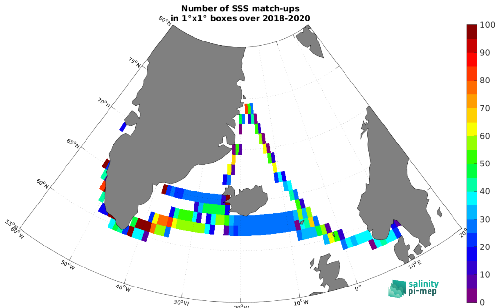
Figure 5: Number of SSS match-ups between TSG (Lauge-Koch) SSS and the SMAP SSS L3 v5.3 - Monthly (RSS) SSS product for the Global Ocean Pi-MEP region over 1^\circ \times 1^\circ boxes and for the full satellite product period.
