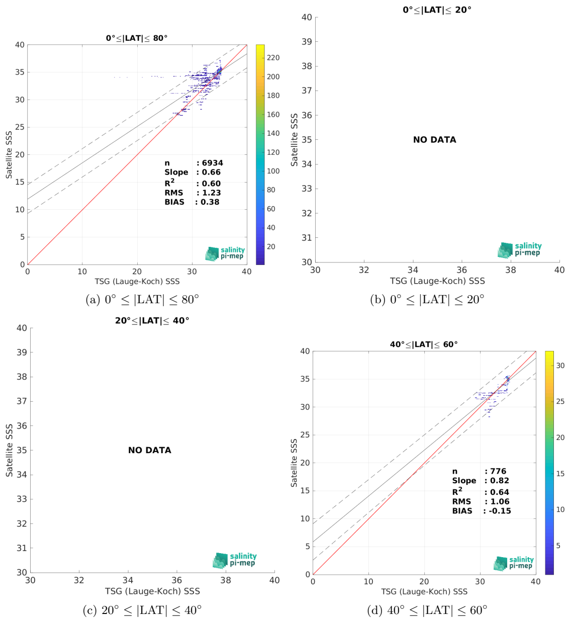
Figure 10: Contour maps of the concentration of SMAP SSS L3 v5.3 - Monthly (RSS) SSS (y-axis) versus TSG (Lauge-Koch) SSS (x-axis) at match-up pairs for different latitude bands. For each plot, the red line shows x=y . The black thin and dashed lines indicate a linear fit through the data cloud and the \pm 95\% confidence levels, respectively. The number match-up pairs n , the slope and R^2 coefficient of the linear fit, the root mean square (RMS) and the mean bias between satellite and in situ data are indicated for each latitude band in each plots.
