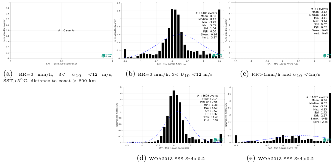
Figure 15: Normalized histogram of \Delta SSS (SMAP SSS L3 v5.3 - Monthly (RSS) - TSG (Lauge-Koch)) for 5 different subdatasets corresponding to: RR=0 mm/h, 3 < U_{10} < 12 m/s, SST > 5°C, distance to coast > 800 km (a), RR=0 mm/h, 3 < U_{10} < 12 m/s (b), RR > 1mm/h and U_{10} < 4 m/s (c), WOA2013 SSS Std < 0.2 (d), WOA2013 SSS Std > 0.2 (e).
