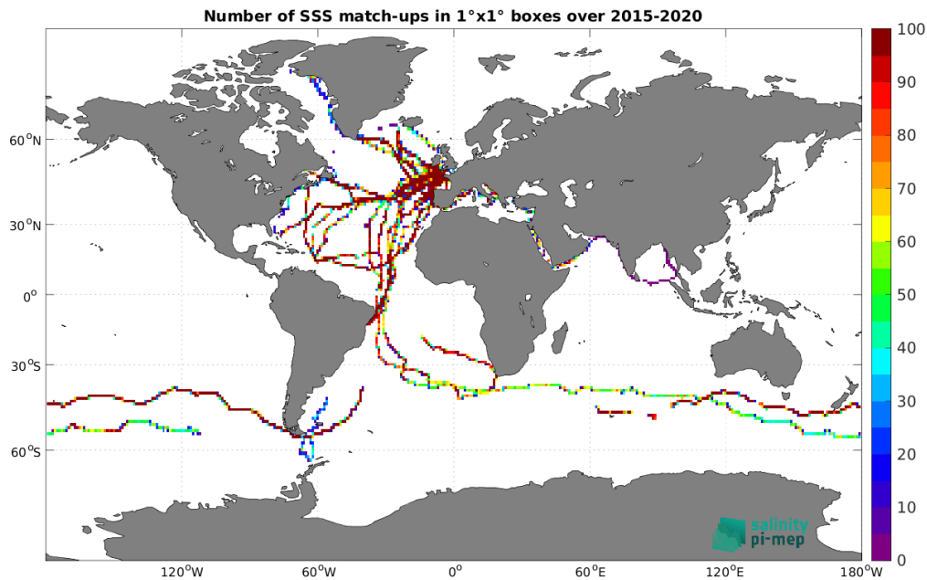
Figure 5: Number of SSS match-ups between TSG (GOSUD-Sailing-ship) SSS and the SMAP SSS L3 v5.3 - Monthly (RSS) SSS product for the Global Ocean Pi-MEP region over 1°x1° boxes and for the full satellite product period.
