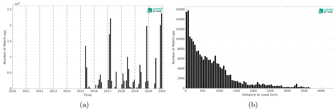
Figure 2: Number of match-ups between TSG (GOSUD-Sailing-ship) and SMAP SSS L3 v5.3 - Monthly (RSS) SSS as a function of time (a) and as function of the distance to coast (b) over the Global Ocean Pi-MEP region and for the full satellite product period.
