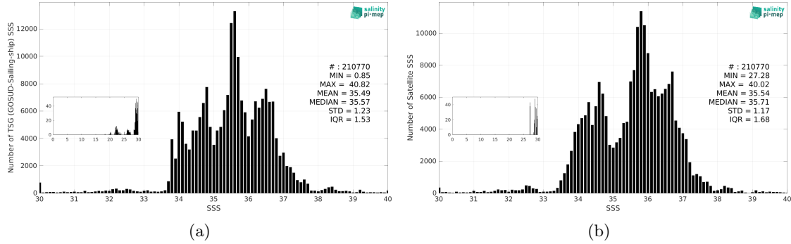
Figure 3: Histograms of SSS from TSG (GOSUD-Sailing-ship) (a) and SMAP SSS L3 v5.3 - Monthly (RSS) (b) considering all match-up pairs per bins of 0.1 over the Global Ocean Pi-MEP region and for the full satellite product period.
