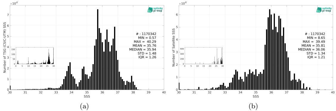
Figure 3: Histograms of SSS from TSG (CSIC-UTM) (a) and SMAP SSS L3 v5.3 - Monthly (RSS) (b) considering all match-up pairs per bins of 0.1 over the Global Ocean Pi-MEP region and for the full satellite product period.
