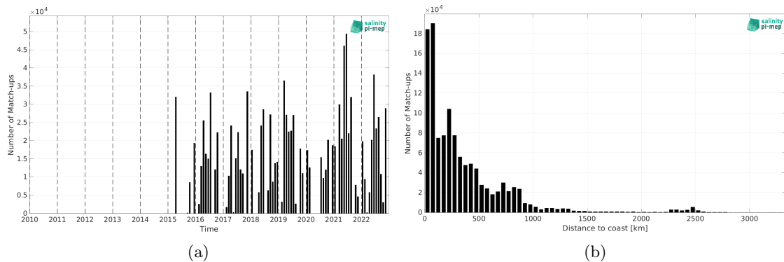
Figure 2: Number of match-ups between TSG (CSIC-UTM) and SMAP SSS L3 v5.3 - Monthly (RSS) SSS as a function of time (a) and as function of the distance to coast (b) over the Global Ocean Pi-MEP region and for the full satellite product period.
