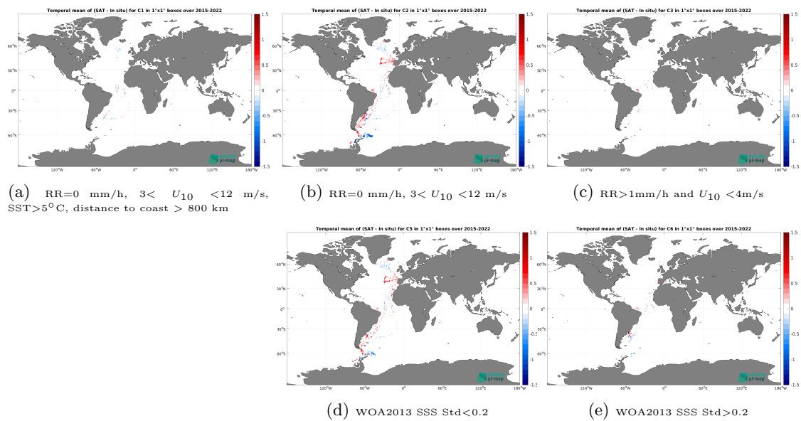
Figure 14: Temporal mean gridded over spatial boxes of size 1^\circ \times 1^\circ of \Delta SSS (SMAP SSS L3 v5.3 - Monthly (RSS) - TSG (CSIC-UTM)) for 5 different subdatasets corresponding to:RR=0 mm/h, 3 < U_{10} < 12 m/s, SST > 5^\circ\text{C} , distance to coast > 800 km (a), RR=0 mm/h, 3 < U_{10} < 12 m/s (b), RR > 1 mm/h and U_{10} < 4 m/s (c), WOA2013 SSS Std < 0.2 (d), WOA2013 SSS Std > 0.2 (e).
