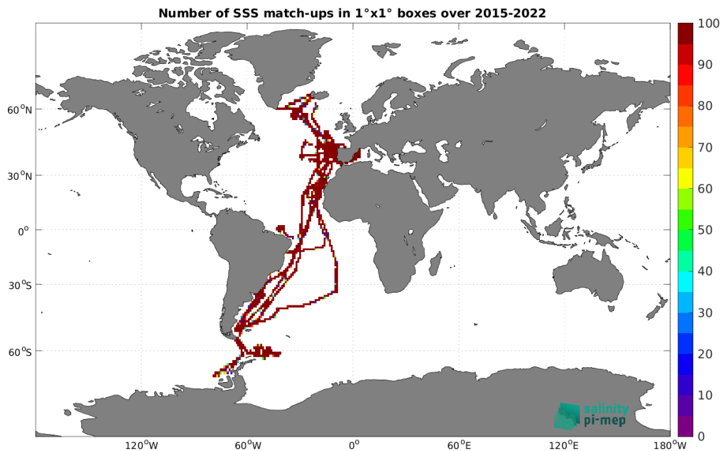
Figure 5: Number of SSS match-ups between TSG (CSIC-UTM) SSS and the SMAP SSS L3 v5.3 - Monthly (RSS) SSS product for the Global Ocean Pi-MEP region over 1°x1° boxes and for the full satellite product period.
