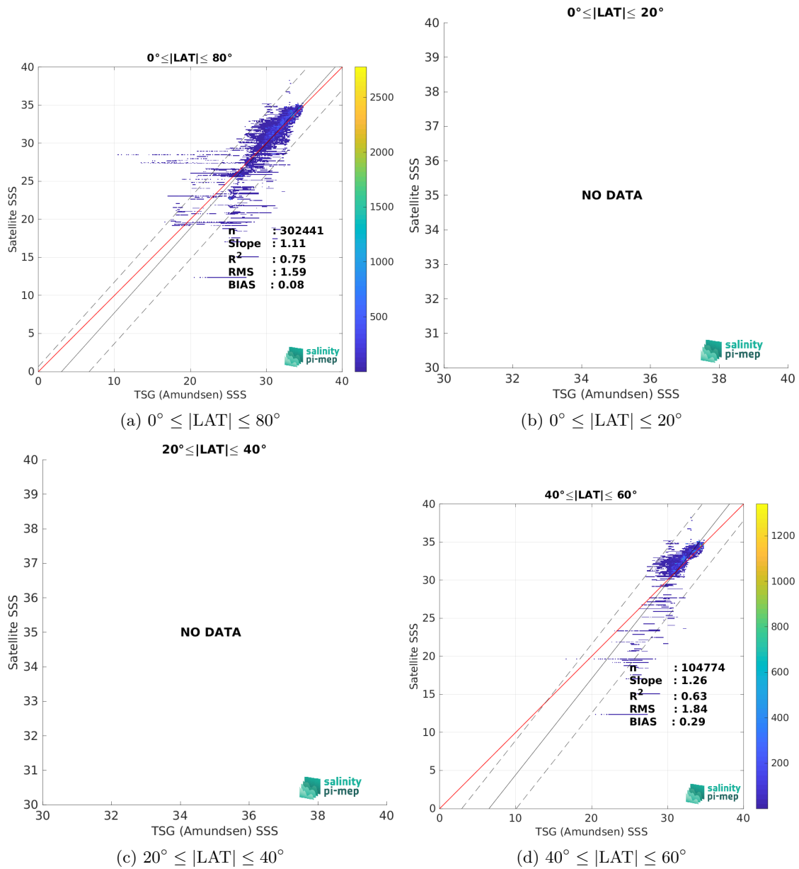
Figure 10: Contour maps of the concentration of SMAP SSS L3 v5.3 - Monthly (RSS) SSS (y-axis) versus TSG (Amundsen) SSS (x-axis) at match-up pairs for different latitude bands. For each plot, the red line shows x=y . The black thin and dashed lines indicate a linear fit through the data cloud and the \pm 95\% confidence levels, respectively. The number match-up pairs n , the slope and R^2 coefficient of the linear fit, the root mean square (RMS) and the mean bias between satellite and in situ data are indicated for each latitude band in each plot.
