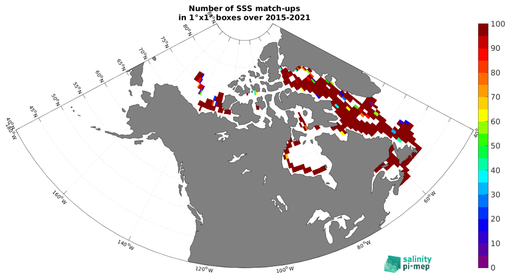
Figure 5: Number of SSS match-ups between TSG (Amundsen) SSS and the SMAP SSS L3 v5.3 - Monthly (RSS) SSS product for the Global Ocean Pi-MEP region over 1^\circ \times 1^\circ boxes and for the full satellite product period.
