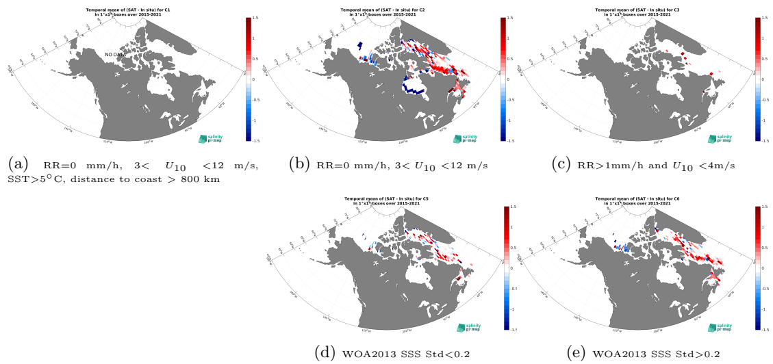
Figure 14: Temporal mean gridded over spatial boxes of size 1^\circ \times 1^\circ of \Delta SSS (SMAP SSS L3 v5.3 - Monthly (RSS) - TSG (Amundsen)) for 5 different subdatasets corresponding to:RR=0 mm/h, 3 < U_{10} < 12 m/s, SST > 5°C, distance to coast > 800 km (a), RR=0 mm/h, 3 < U_{10} < 12 m/s (b), RR > 1mm/h and U_{10} < 4 m/s (c), WOA2013 SSS Std < 0.2 (d), WOA2013 SSS Std > 0.2 (e).
