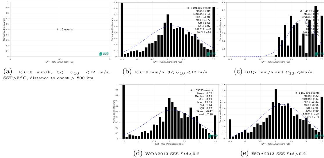
Figure 15: Normalized histogram of \Delta SSS (SMAP SSS L3 v5.3 - Monthly (RSS) - TSG (Amundsen)) for 5 different subdatasets corresponding to: RR=0 mm/h, 3 < U_{10} < 12 m/s, SST > 5°C, distance to coast > 800 km (a), RR=0 mm/h, 3 < U_{10} < 12 m/s (b), RR > 1mm/h and U_{10} < 4 m/s (c), WOA2013 SSS Std < 0.2 (d), WOA2013 SSS Std > 0.2 (e).
