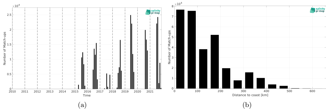
Figure 2: Number of match-ups between TSG (Amundsen) and SMAP SSS L3 v5.3 - Monthly (RSS) SSS as a function of time (a) and as function of the distance to coast (b) over the Global Ocean Pi-MEP region and for the full satellite product period.
