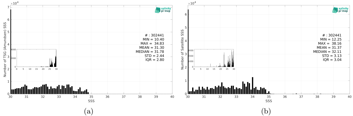
Figure 3: Histograms of SSS from TSG (Amundsen) (a) and SMAP SSS L3 v5.3 - Monthly (RSS) (b) considering all match-up pairs per bins of 0.1 over the Global Ocean Pi-MEP region and for the full satellite product period.
