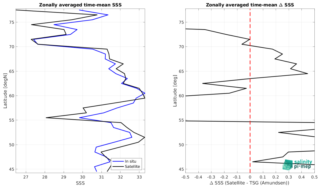
Figure 9: Left panel: Zonal mean SSS from SMAP SSS L3 v5.3 - Monthly (RSS) satellite product (black) and from TSG (Amundsen) (blue). Right panel: Zonal mean of \Delta SSS (Satellite - TSG (Amundsen)) for all the collected Pi-MEP match-up pairs estimated over the full satellite product period.
