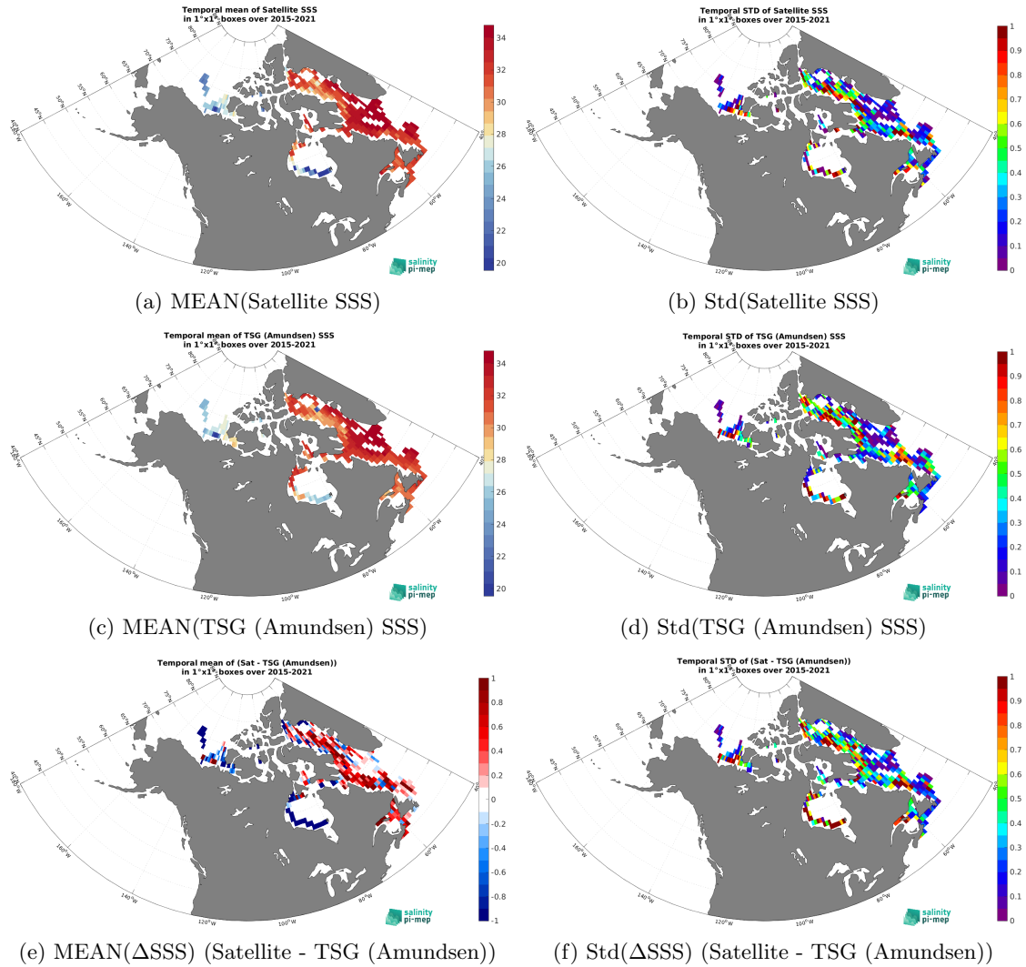
Figure 7: Temporal mean (left) and Std (right) of SSS from SMAP SSS L3 v5.3 - Monthly (RSS) (top), TSG (Amundsen) (middle), and of \Delta SSS (Satellite - TSG (Amundsen)). Only match-up pairs are used to generate these maps.
