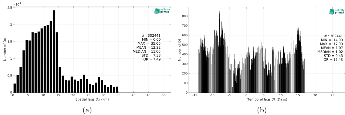
Figure 6: Histograms of the spatial (a) and temporal (b) lags between the location/time of the TSG (Amundsen) measurement and the date of the corresponding SMAP SSS L3 v5.3 - Monthly (RSS) SSS pixel.
