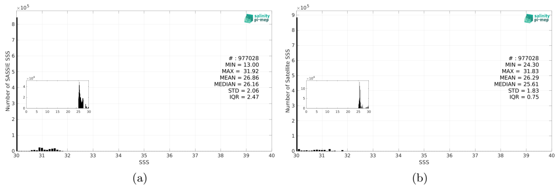
Figure 3: Histograms of SSS from SASSIE (a) and SMAP SSS L3 v5.3 - Monthly (RSS) (b) considering all match-up pairs per bins of 0.1 over the Global Ocean Pi-MEP region and for the full satellite product period.
