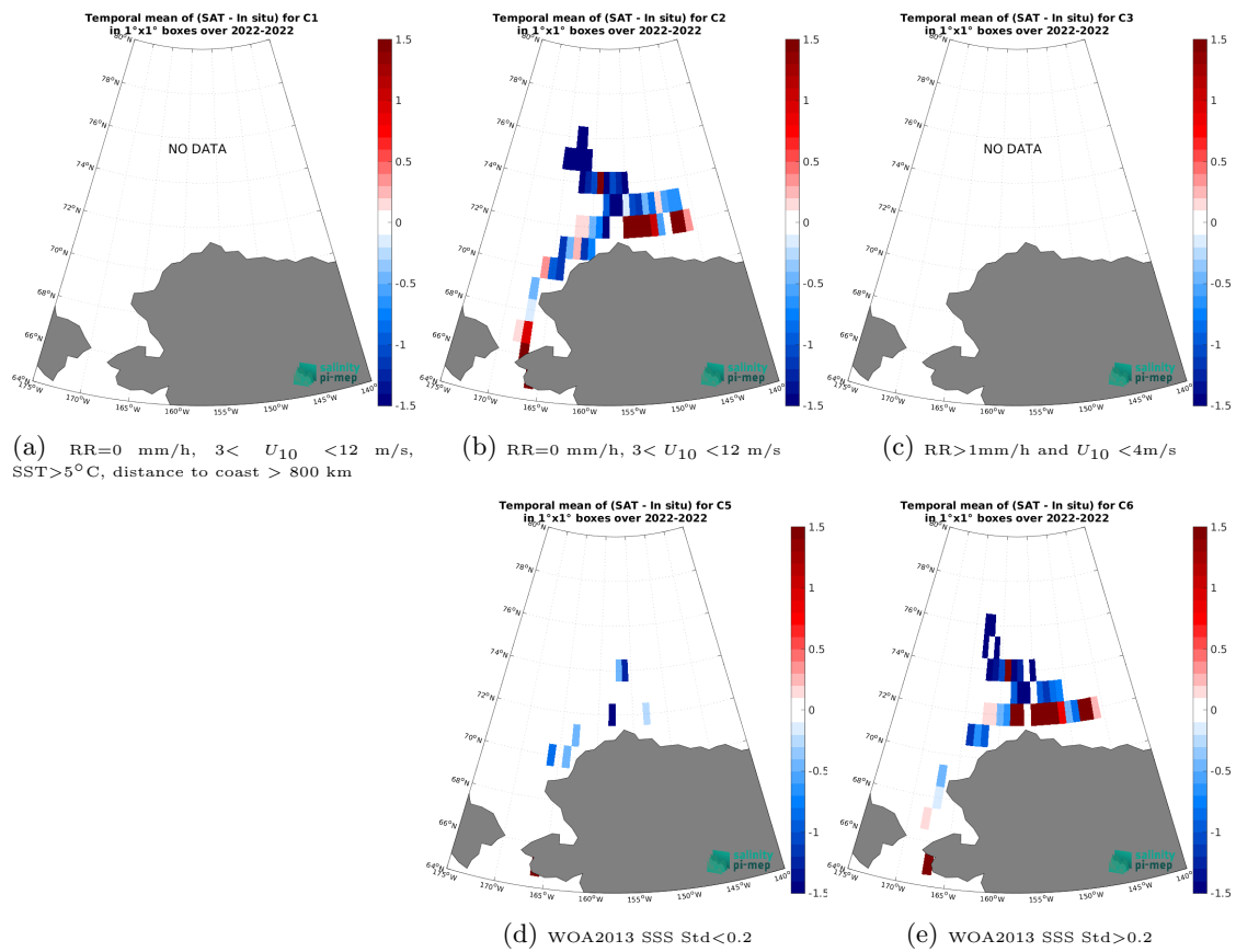
Figure 14: Temporal mean gridded over spatial boxes of size 1^\circ \times 1^\circ of \Delta SSS (SMAP SSS L3 v5.3 - Monthly (RSS) - SASSIE) for 5 different subdatasets corresponding to:RR=0 mm/h, 3 < U_{10} < 12 m/s, SST>5°C, distance to coast > 800 km (a), RR=0 mm/h, 3 < U_{10} < 12 m/s (b), RR>1mm/h and U_{10} < 4 m/s (c), WOA2013 SSS Std<0.2 (d), WOA2013 SSS Std>0.2 (e).
