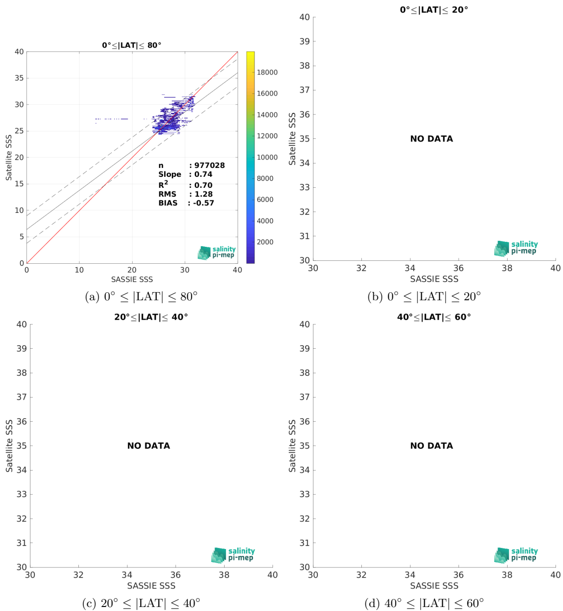
Figure 10: Contour maps of the concentration of SMAP SSS L3 v5.3 - Monthly (RSS) SSS (y-axis) versus SASSIE SSS (x-axis) at match-up pairs for different latitude bands. For each plot, the red line shows x=y . The black thin and dashed lines indicate a linear fit through the data cloud and the \pm 95\% confidence levels, respectively. The number match-up pairs n , the slope and R^2 coefficient of the linear fit, the root mean square (RMS) and the mean bias between satellite and in situ data are indicated for each latitude band in each plots.
