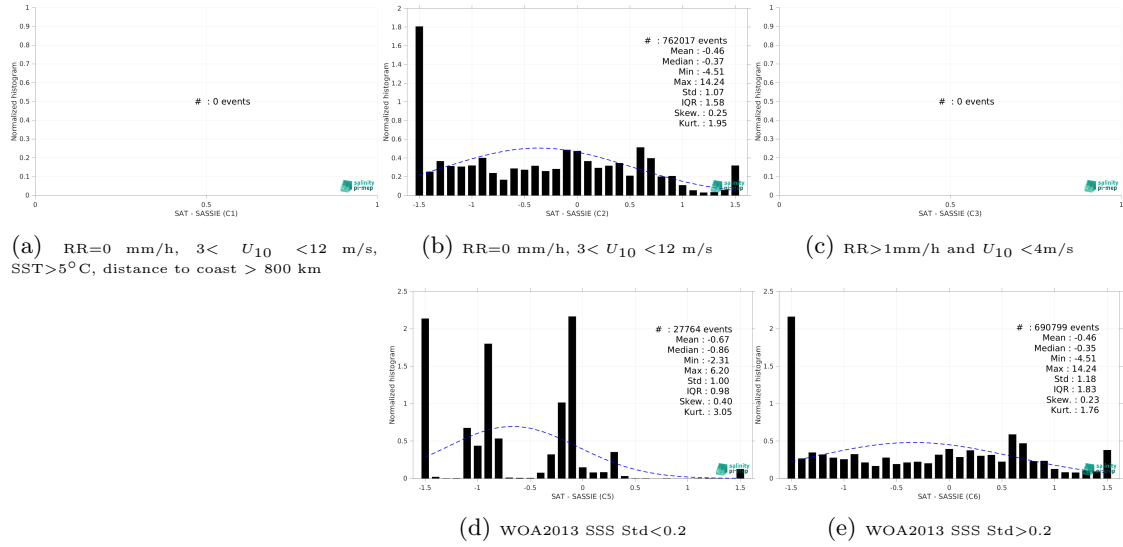
Figure 15: Normalized histogram of \Delta SSS (SMAP SSS L3 v5.3 - Monthly (RSS) - SASSIE) for 5 different subdatasets corresponding to: RR=0 mm/h, 3 < U_{10} < 12 m/s, SST > 5°C, distance to coast > 800 km (a), RR=0 mm/h, 3 < U_{10} < 12 m/s (b), RR > 1mm/h and U_{10} < 4 m/s (c), WOA2013 SSS Std < 0.2 (d), WOA2013 SSS Std > 0.2 (e).
