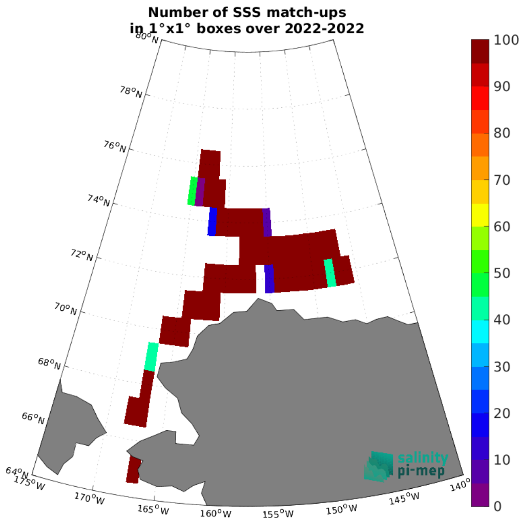
Figure 5: Number of SSS match-ups between SASSIE SSS and the SMAP SSS L3 v5.3 - Monthly (RSS) SSS product for the Global Ocean Pi-MEP region over 1^\circ \times 1^\circ boxes and for the full satellite product period.
