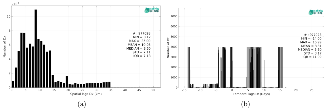
Figure 6: Histograms of the spatial (a) and temporal (b) lags between the location/time of the SASSIE measurement and the date of the corresponding SMAP SSS L3 v5.3 - Monthly (RSS) SSS pixel.
