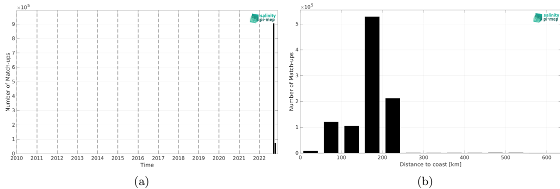
Figure 2: Number of match-ups between SASSIE and SMAP SSS L3 v5.3 - Monthly (RSS) SSS as a function of time (a) and as function of the distance to coast (b) over the Global Ocean Pi-MEP region and for the full satellite product period.
