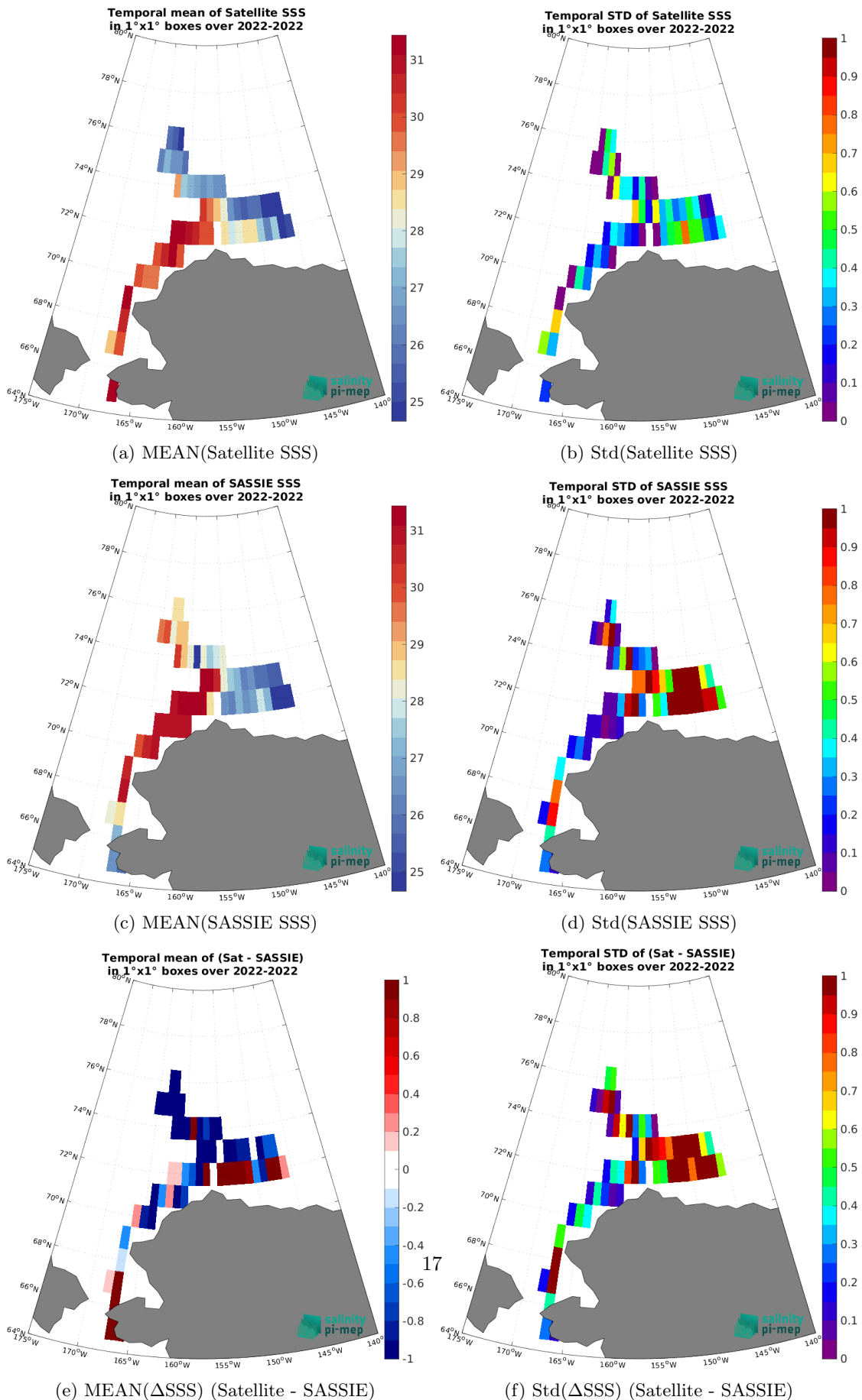
Figure 7: Temporal mean (left) and Std (right) of SSS from SMAP SSS L3 v5.3 - Monthly (RSS) (top), SASSIE (middle), and of \Delta SSS (Satellite - SASSIE). Only match-up pairs are used to generate these maps.
