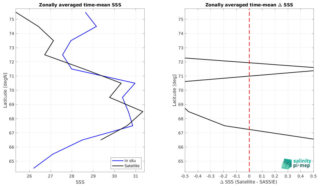
Figure 9: Left panel: Zonal mean SSS from SMAP SSS L3 v5.3 - Monthly (RSS) satellite product (black) and from SASSIE (blue). Right panel: Zonal mean of \Delta SSS (Satellite - SASSIE) for all the collected Pi-MEP match-up pairs estimated over the full satellite product period.
