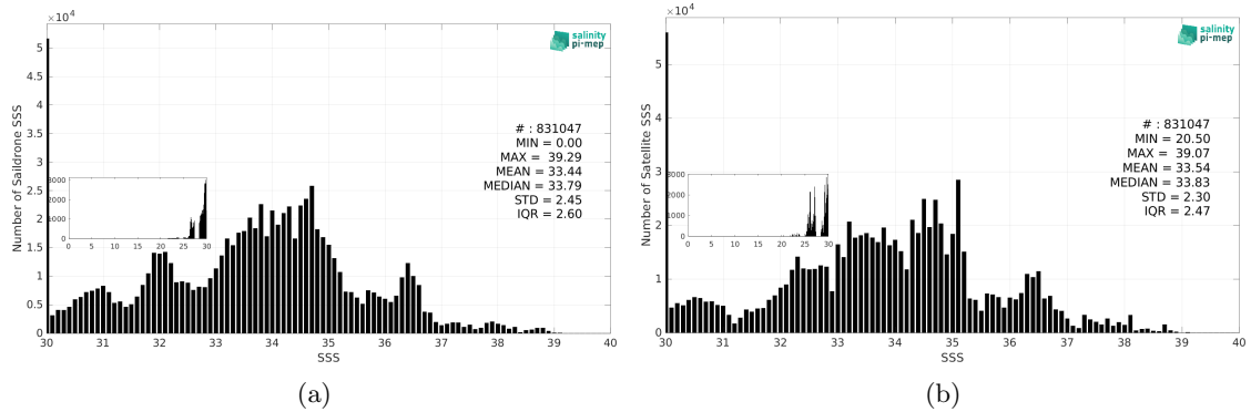
Figure 3: Histograms of SSS from Saildrone (a) and SMAP SSS L3 v5.3 - Monthly (RSS) (b) considering all match-up pairs per bins of 0.1 over the Global Ocean Pi-MEP region and for the full satellite product period.
