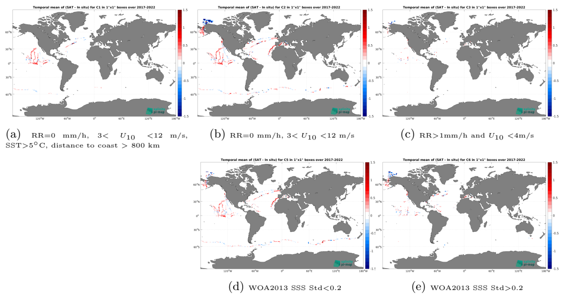
Figure 14: Temporal mean gridded over spatial boxes of size 1^\circ \times 1^\circ of \Delta SSS (SMAP SSS L3 v5.3 - Monthly (RSS) - Saifdrone) for 5 different subdatasets corresponding to:RR=0 mm/h, 3 < U_{10} < 12 m/s, SST > 5^\circ\text{C} , distance to coast > 800 km (a), RR=0 mm/h, 3 < U_{10} < 12 m/s (b), RR > 1 mm/h and U_{10} < 4 m/s (c), WOA2013 SSS Std < 0.2 (d), WOA2013 SSS Std > 0.2 (e).
