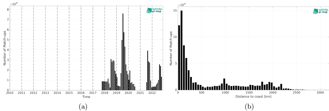
Figure 2: Number of match-ups between Saildrone and SMAP SSS L3 v5.3 - Monthly (RSS) SSS as a function of time (a) and as function of the distance to coast (b) over the Global Ocean Pi-MEP region and for the full satellite product period.
