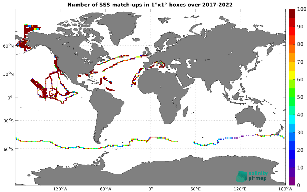
Figure 5: Number of SSS match-ups between Saildrone SSS and the SMAP SSS L3 v5.3 - Monthly (RSS) SSS product for the Global Ocean Pi-MEP region over 1°×1° boxes and for the full satellite product period.
