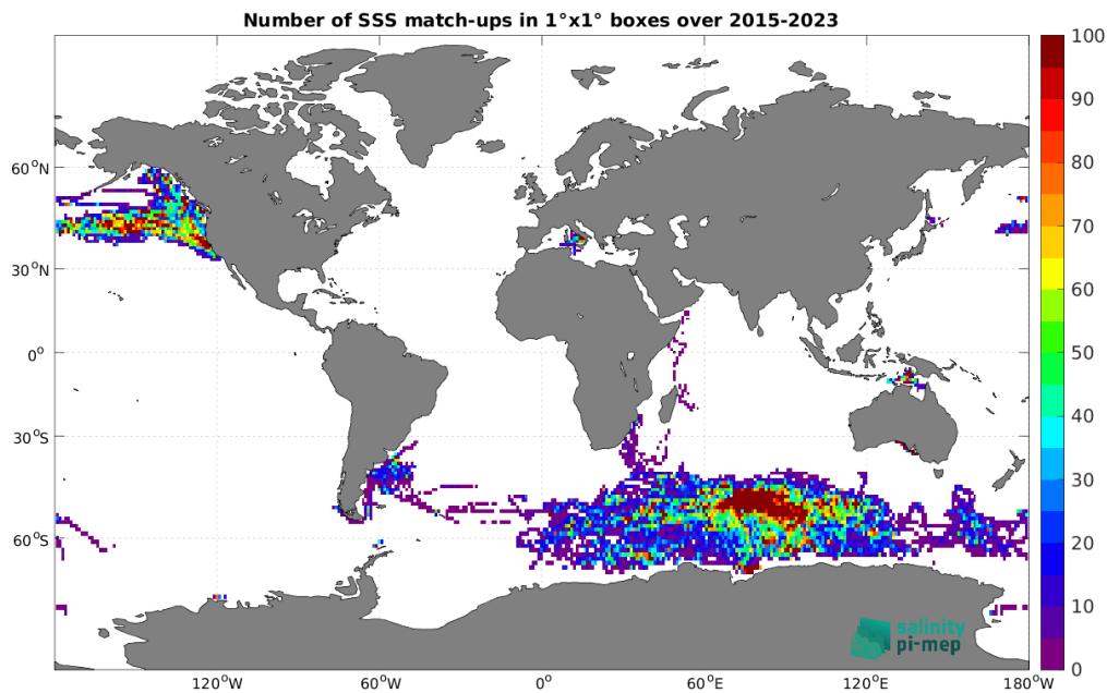
Figure 5: Number of SSS match-ups between Marine mammals SSS and the SMAP SSS L3 v5.3 - Monthly (RSS) SSS product for the Global Ocean Pi-MEP region over 1^\circ \times 1^\circ boxes and for the full satellite product period.
