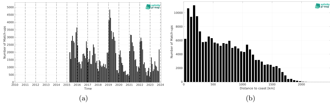
Figure 2: Number of match-ups between Marine mammals and SMAP SSS L3 v5.3 - Monthly (RSS) SSS as a function of time (a) and as function of the distance to coast (b) over the Global Ocean Pi-MEP region and for the full satellite product period.
