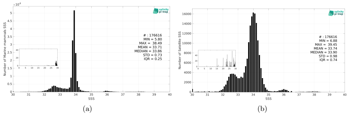
Figure 3: Histograms of SSS from Marine mammals (a) and SMAP SSS L3 v5.3 - Monthly (RSS) (b) considering all match-up pairs per bins of 0.1 over the Global Ocean Pi-MEP region and for the full satellite product period.
