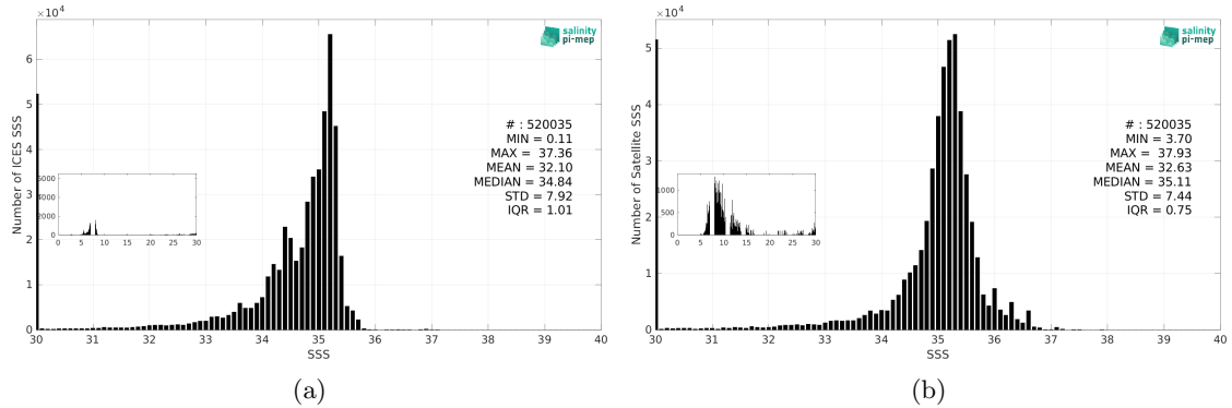
Figure 3: Histograms of SSS from ICES (a) and SMAP SSS L3 v5.3 - Monthly (RSS) (b) considering all match-up pairs per bins of 0.1 over the Global Ocean Pi-MEP region and for the full satellite product period.
