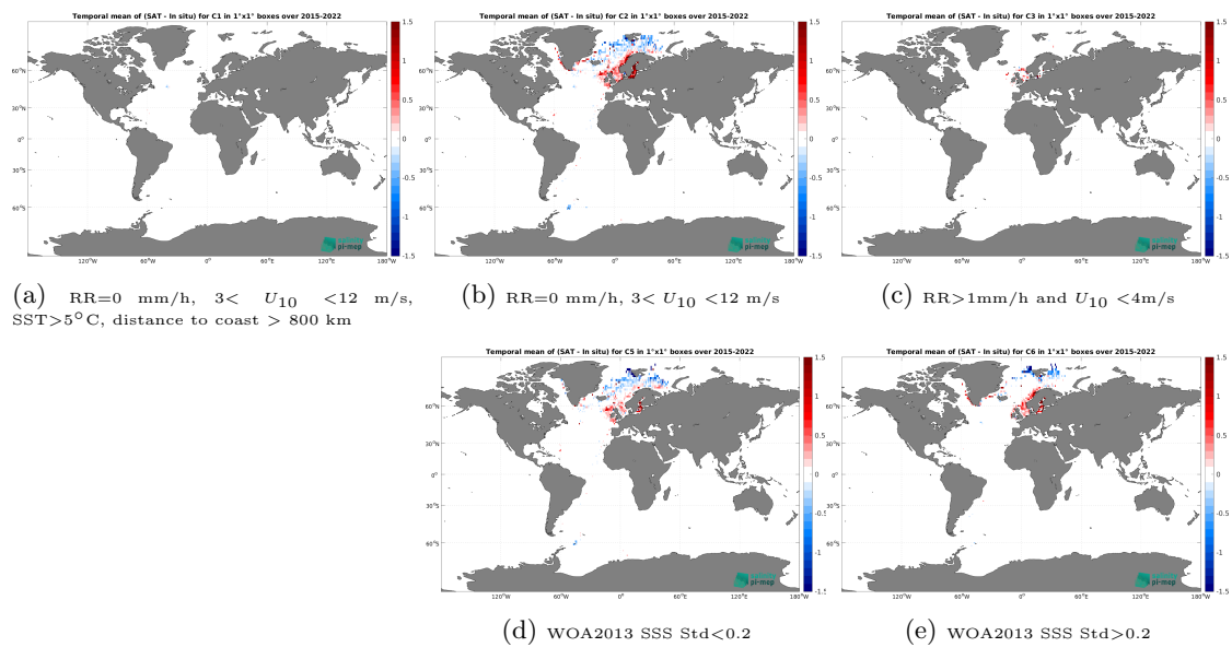
Figure 14: Temporal mean gridded over spatial boxes of size 1^\circ \times 1^\circ of \Delta SSS (SMAP SSS L3 v5.3 - Monthly (RSS) - ICES) for 5 different subdatasets corresponding to:RR=0 mm/h, 3 < U_{10} < 12 m/s, SST > 5^\circ\text{C} , distance to coast > 800 km (a), RR=0 mm/h, 3 < U_{10} < 12 m/s (b), RR > 1 mm/h and U_{10} < 4 m/s (c), WOA2013 SSS Std < 0.2 (d), WOA2013 SSS Std > 0.2 (e).
