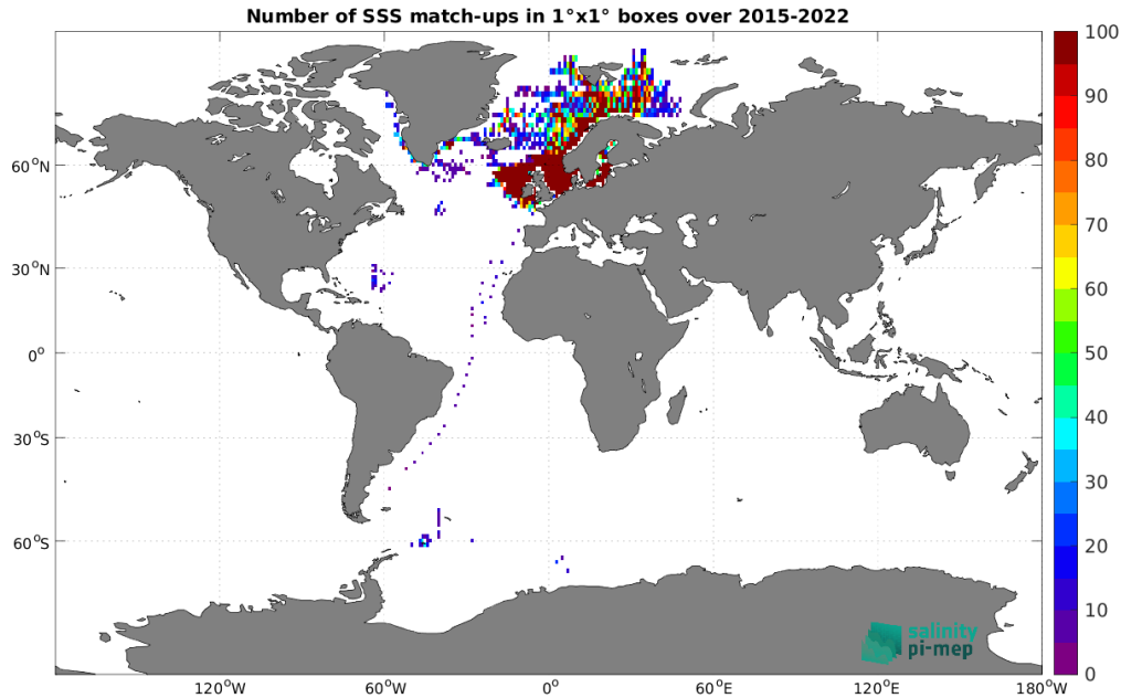
Figure 5: Number of SSS match-ups between ICES SSS and the SMAP SSS L3 v5.3 - Monthly (RSS) SSS product for the Global Ocean Pi-MEP region over 1^\circ \times 1^\circ boxes and for the full satellite product period.
