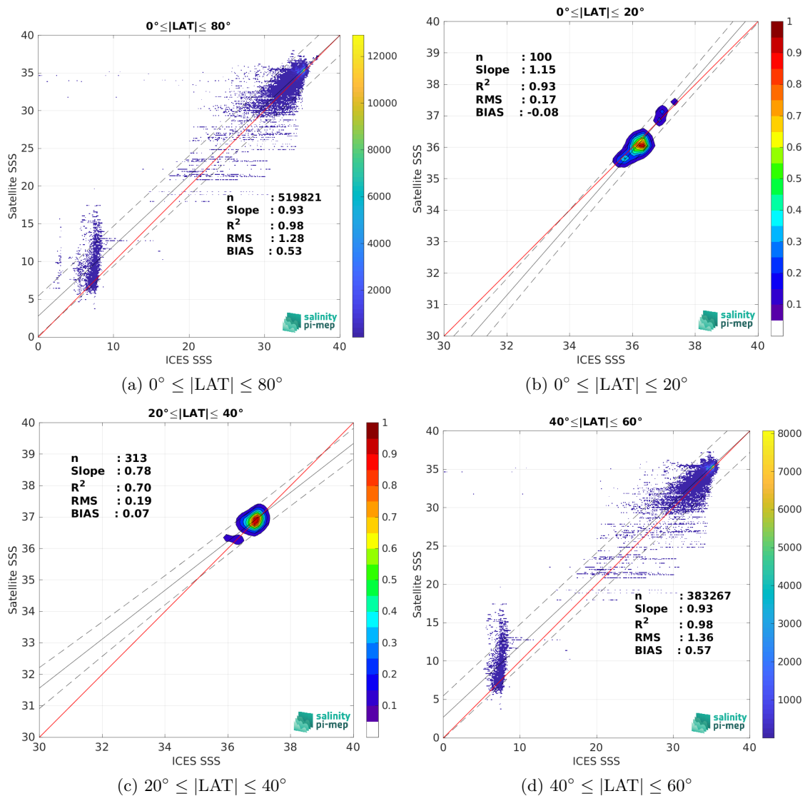
Figure 10: Contour maps of the concentration of SMAP SSS L3 v5.3 - Monthly (RSS) SSS (y-axis) versus ICES SSS (x-axis) at match-up pairs for different latitude bands. For each plot, the red line shows x=y . The black thin and dashed lines indicate a linear fit through the data cloud and the \pm 95\% confidence levels, respectively. The number match-up pairs n , the slope and R^2 coefficient of the linear fit, the root mean square (RMS) and the mean bias between satellite and in situ data are indicated for each latitude band in each plots.
