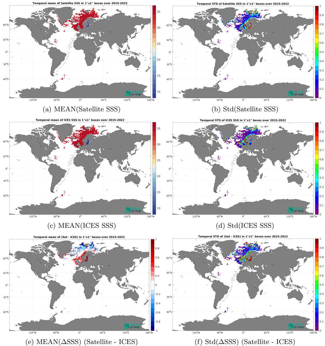
Figure 7: Temporal mean (left) and Std (right) of SSS from SMAP SSS L3 v5.3 - Monthly (RSS) (top), ICES (middle), and of \Delta SSS (Satellite - ICES). Only match-up pairs are used to generate these maps.
