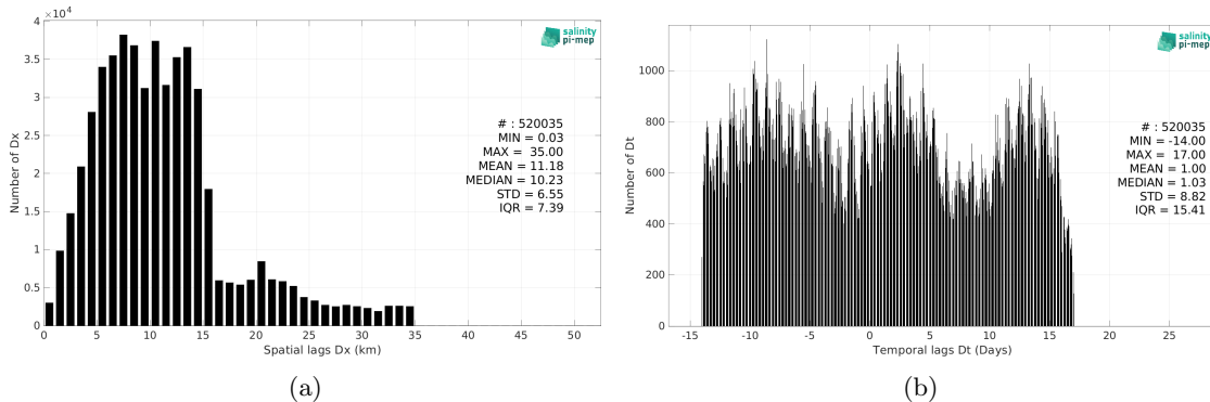
Figure 6: Histograms of the spatial (a) and temporal (b) lags between the location/time of the ICES measurement and the date of the corresponding SMAP SSS L3 v5.3 - Monthly (RSS) SSS pixel.
