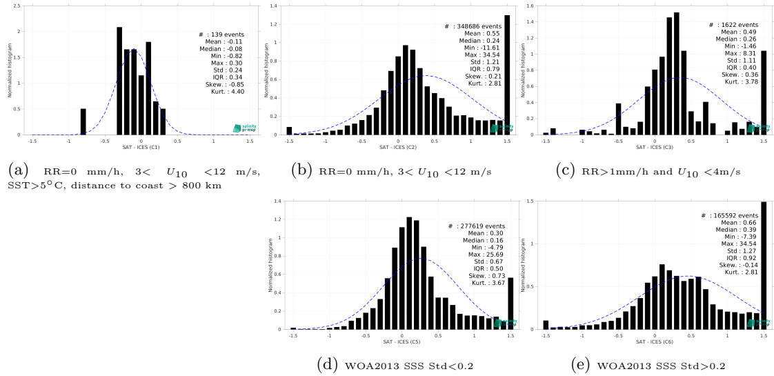
Figure 15: Normalized histogram of \Delta\text{SSS} (SMAP SSS L3 v5.3 - Monthly (RSS) - ICES) for 5 different subdatasets corresponding to: RR=0 mm/h, 3 < U_{10} < 12 m/s, SST>5°C, distance to coast > 800 km (a), RR=0 mm/h, 3 < U_{10} < 12 m/s (b), RR>1mm/h and U_{10} < 4 m/s (c), WOA2013 SSS Std<0.2 (d), WOA2013 SSS Std>0.2 (e).
