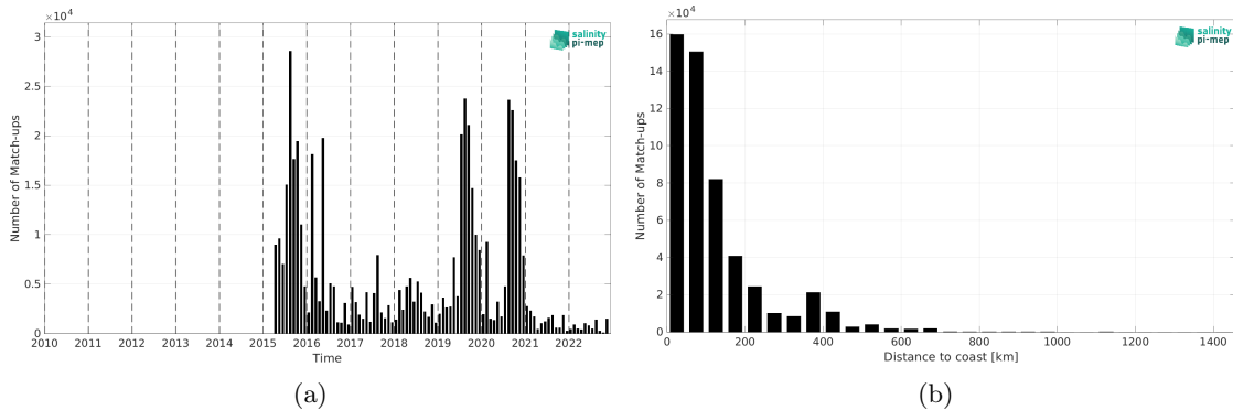
Figure 2: Number of match-ups between ICES and SMAP SSS L3 v5.3 - Monthly (RSS) SSS as a function of time (a) and as function of the distance to coast (b) over the Global Ocean Pi-MEP region and for the full satellite product period.
