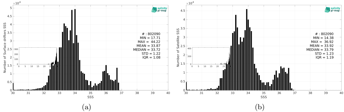
Figure 3: Histograms of SSS from Surface drifters (a) and SMAP SSS L3 v5.3 - Monthly (RSS) (b) considering all match-up pairs per bins of 0.1 over the Global Ocean Pi-MEP region and for the full satellite product period.
