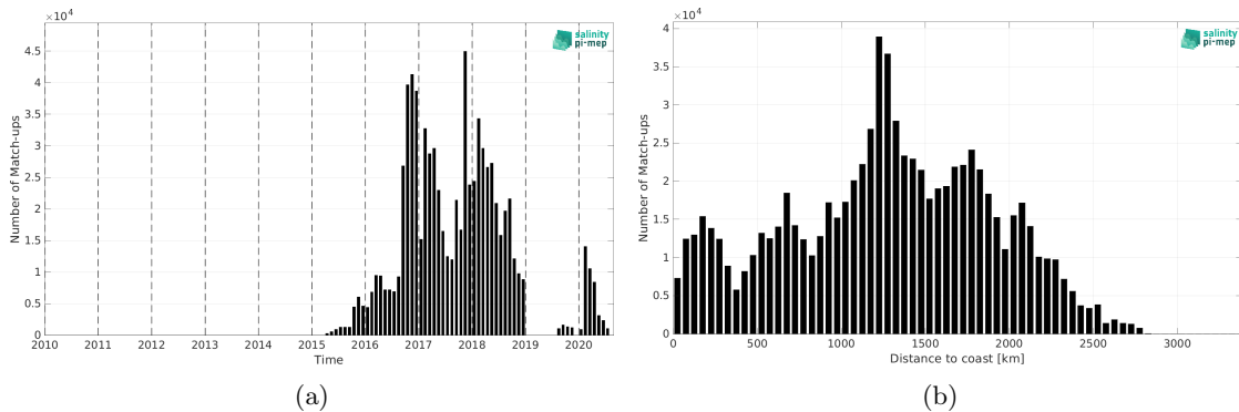
Figure 2: Number of match-ups between Surface drifters and SMAP SSS L3 v5.3 - Monthly (RSS) SSS as a function of time (a) and as function of the distance to coast (b) over the Global Ocean Pi-MEP region and for the full satellite product period.
