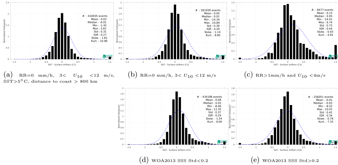
Figure 14: Normalized histogram of \Delta SSS (SMAP SSS L3 v5.3 - Monthly (RSS) - Surface drifters) for 5 different subdatasets corresponding to: RR=0 mm/h, 3 < U_{10} < 12 m/s, SST>5°C, distance to coast > 800 km (a), RR=0 mm/h, 3 < U_{10} < 12 m/s (b), RR>1mm/h and U_{10} < 4 m/s (c), WOA2013 SSS Std<0.2 (d), WOA2013 SSS Std>0.2 (e).
