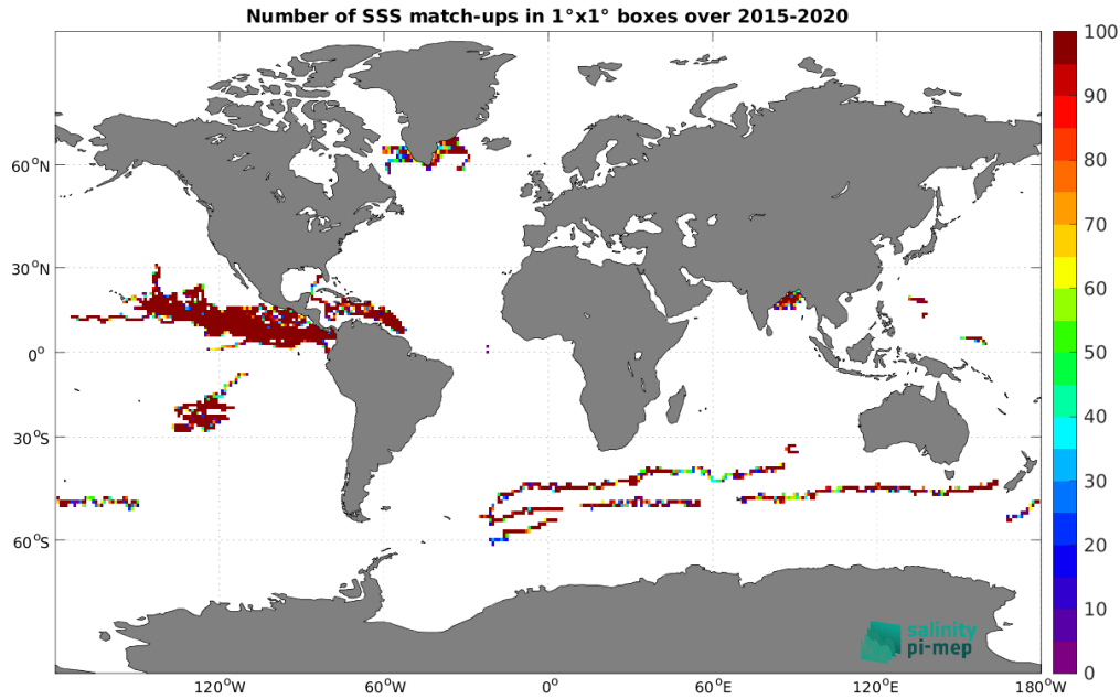
Figure 4: Number of SSS match-ups between Surface drifters SSS and the SMAP SSS L3 v5.3 - Monthly (RSS) SSS product for the Global Ocean Pi-MEP region over 1^\circ \times 1^\circ boxes and for the full satellite product period.
