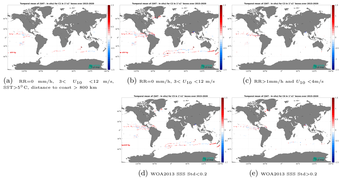
Figure 13: Temporal mean gridded over spatial boxes of size 1^\circ \times 1^\circ of \Delta SSS (SMAP SSS L3 v5.3 - Monthly (RSS) - Surface drifters) for 5 different subdatasets corresponding to:RR=0 mm/h, 3 < U_{10} < 12 m/s, SST > 5^\circ\text{C} , distance to coast > 800 km (a), RR=0 mm/h, 3 < U_{10} < 12 m/s (b), RR > 1 mm/h and U_{10} < 4 m/s (c), WOA2013 SSS Std < 0.2 (d), WOA2013 SSS Std > 0.2 (e).
